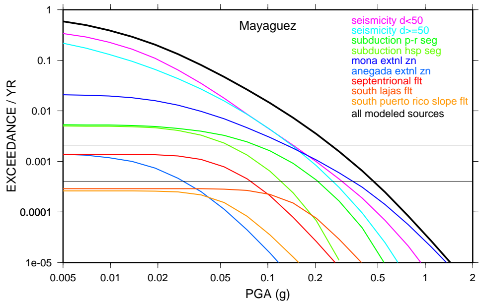
Fig.13b: PGA hazard curves for Mayaguez.
