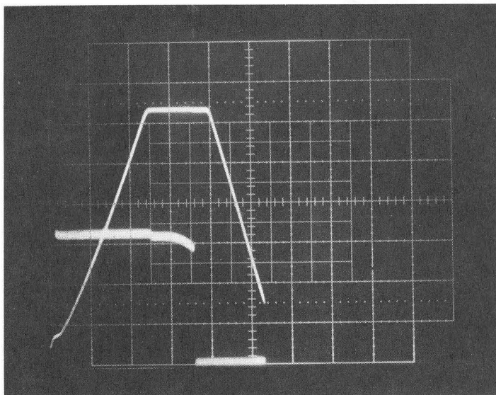
Oscilloscope trace of one cycle in the Energy Saver at 2054 (see Main Control Room Log entry) on February 15. The flat portion on the upper trace is the 800-GeV level.
