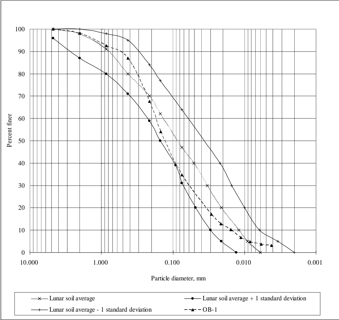
Figure 1, Particle size distribution of OB-1 lunar simulant
