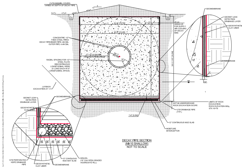
Figure 3-35: Typical cross section of concentric decay pipe and shielding concrete.
