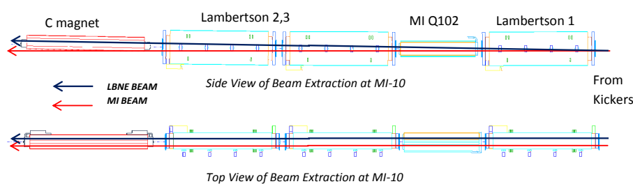
Figure 2–3: Configuration of the LBNE extraction Lambertsons and C-magnet straddling MI quad Q102
