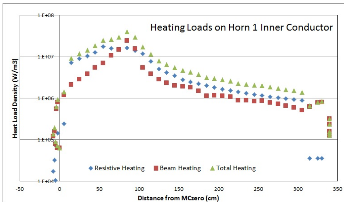
Figure 3–19: Heating loads on the inner conductor of Horn 1
