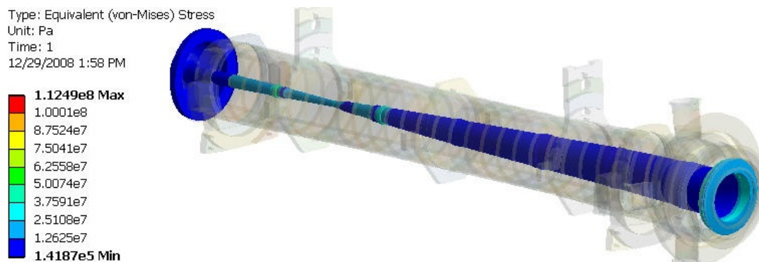
Figure 3–25: Stress due to magnetic loading at mid-pulse for Horn 1.
