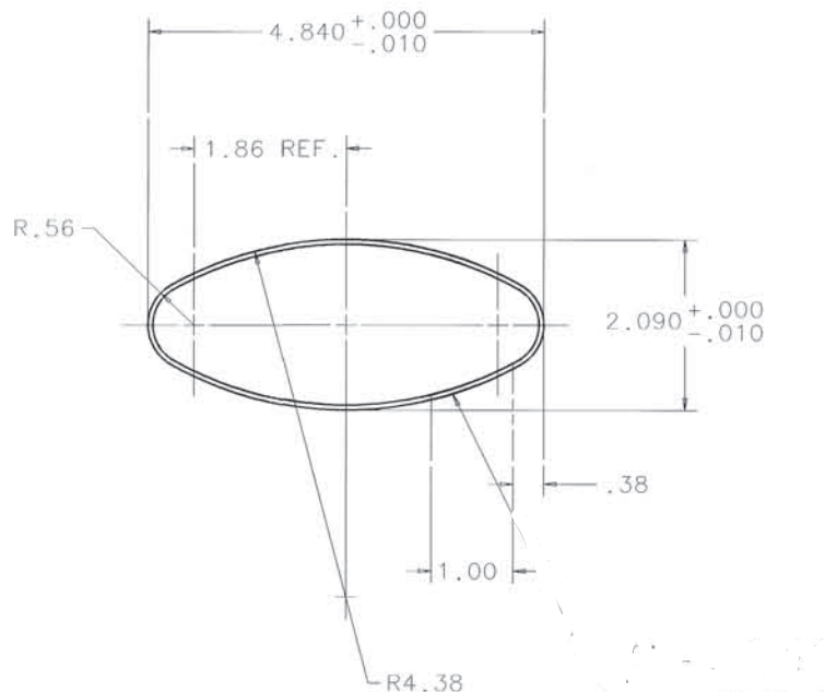
Figure 2-13: Beam tube cross section
