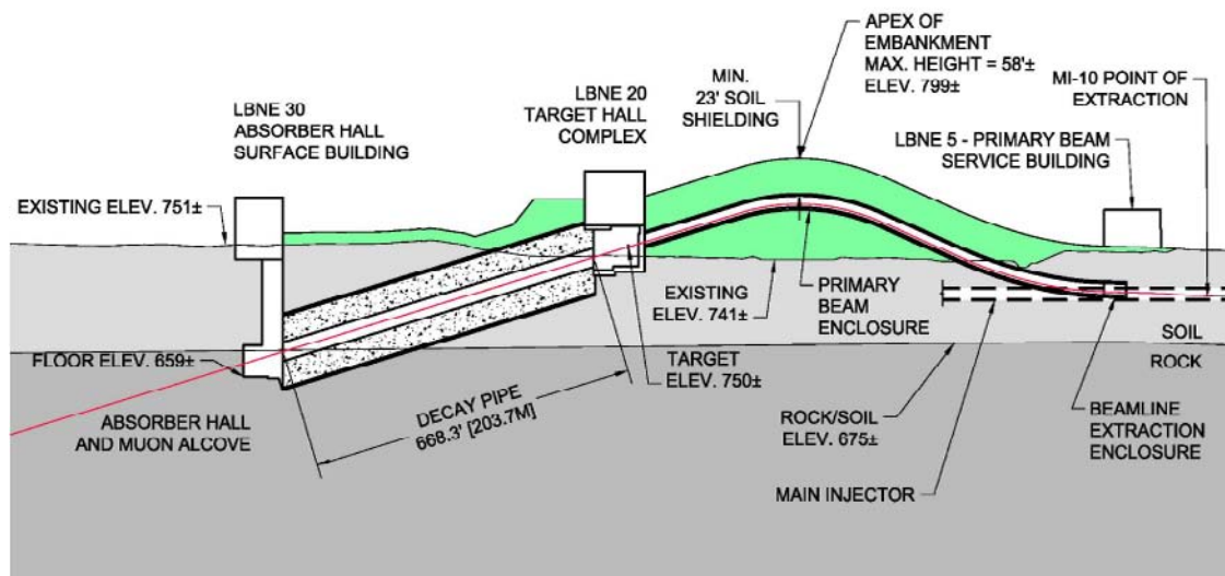
Figure 2-1: Elevation view showing the concept of elevating the beamline, thereby minimizing the amount of deep excavation and tunnels. The beam comes from the right through the primary beam enclosure and interacts at target within the Target Hall Complex. The green shaded part indicates fill used to elevate the beam.
