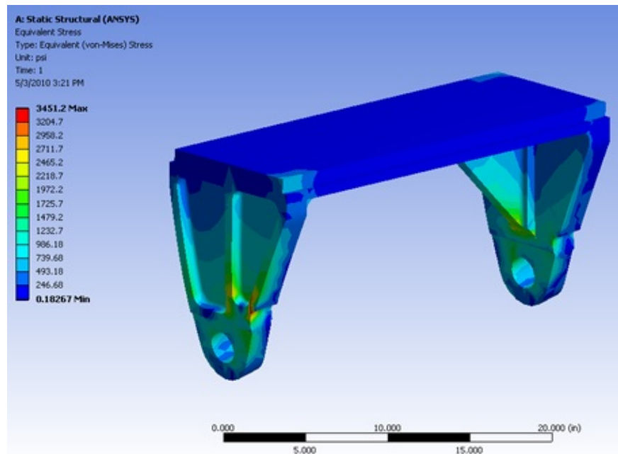
Figure 3–27: Horn hanger structural analysis with tri-axial loading.
