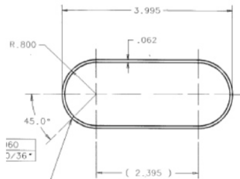
Figure 2-18: ICA beam tube shown in horizontal bending orientation.
