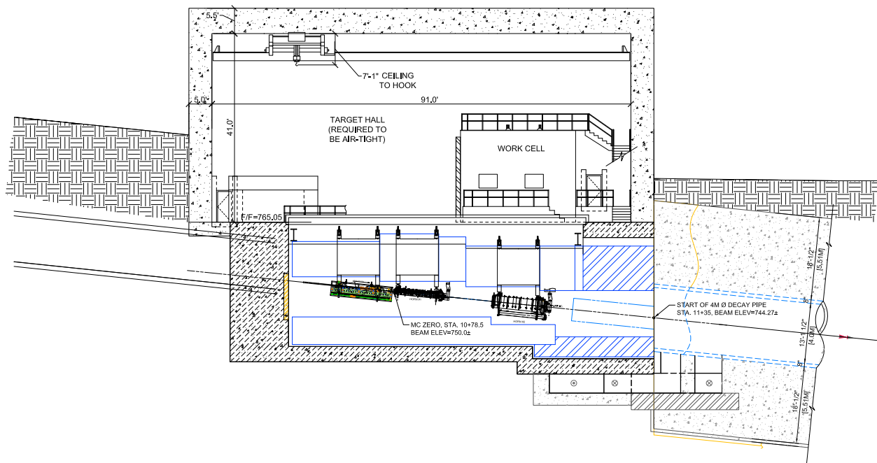
Figure 3-47: LBNE Target Hall enclosure beamline elevation section
