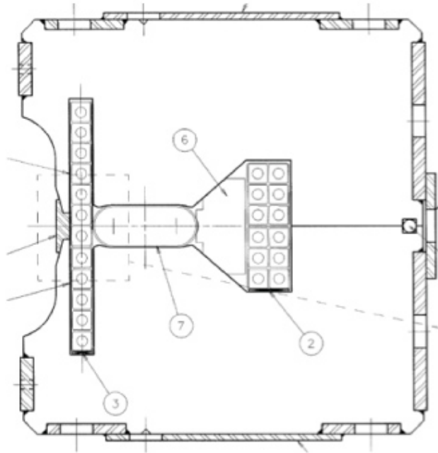
Figure 2-17: ICA MI C Magnet.
