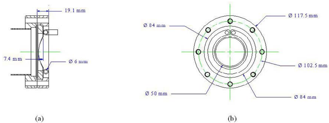
Figure 3-5: Section view of 2.3-MW-capable beryllium window. (b): End view of window assembly.
