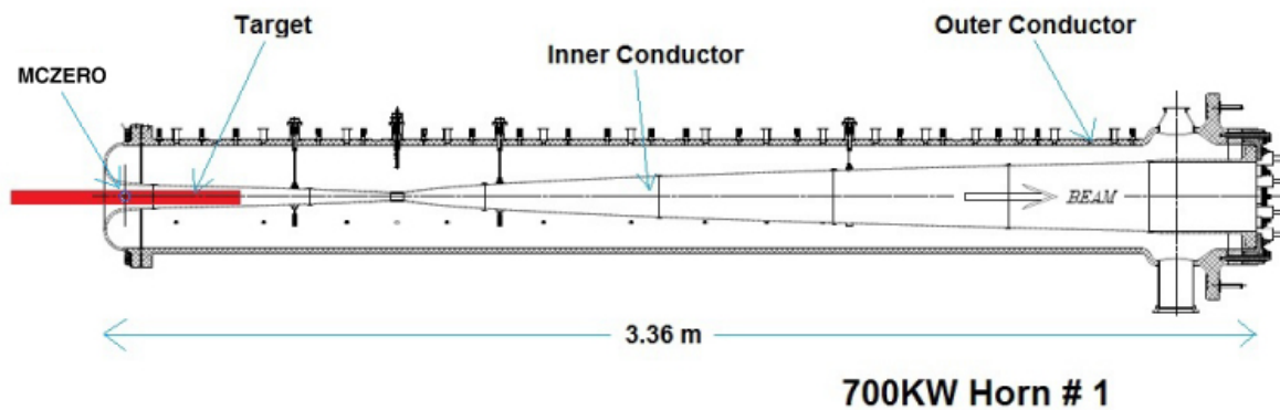
Figure 3-12: Horn 1 section. The reference “MCZERO” is the point along the beam that sets the coordinate system origin for Monte Carlo simulations. Horn 1 specifications are listed in Table 3-2.
