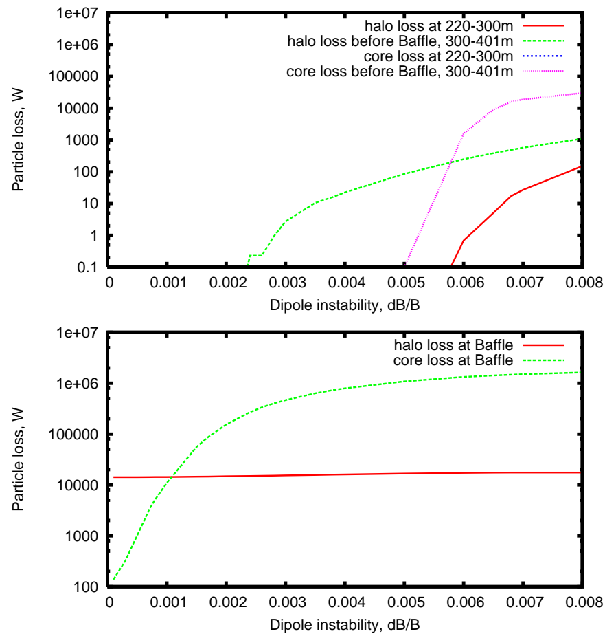
Figure 2-33: The halo and core beam loss at 120 GeV along the LBNE primary beam line (top) and at the Baffle (bottom) as a function of dipole magnet power supply instability, with common power supply for several dipoles.
