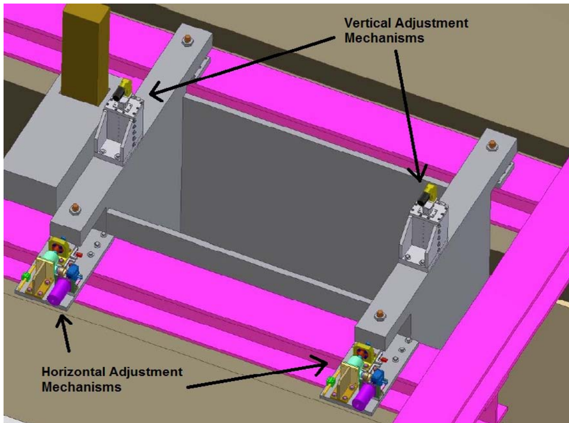
Figure 3-29: Adjustment fixtures for the horn-support module concept. The modules are fixed only horizontally along the beam direction.
