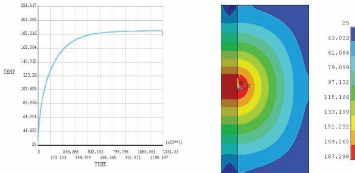
Figure 3-39: Results from ANSYS simulation. The maximum temperature ( ^{\circ}\text{C} ) versus time \times 10 (s) for the third Al core block is shown (left) after 10,000 normal pulses. The temperature distribution in the same block is shown to the right.
