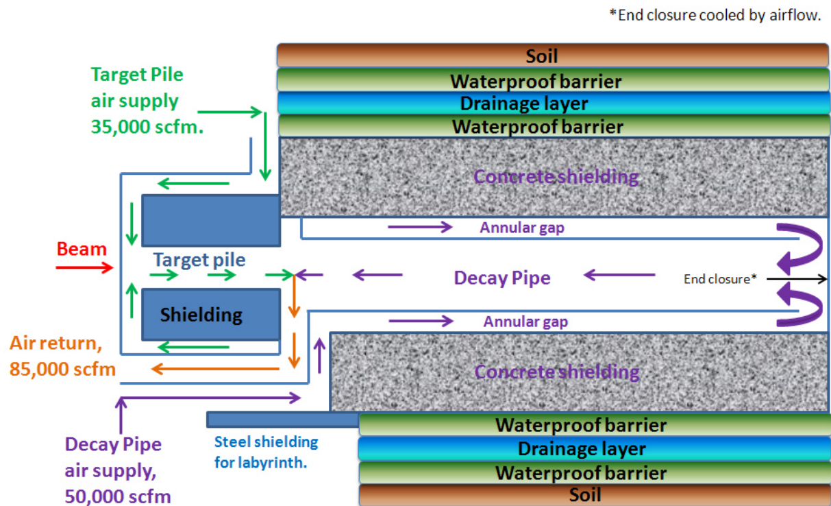
Figure 3-46: The flows for the Target pile and decay pipe air-cooling concept are shown schematically.
