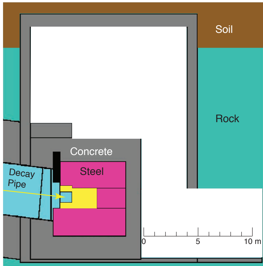
Figure 3–37: Simplified elevation view of the absorber within the Absorber Hall. The white zones are air. Most of the energy (from the uninteracted protons) is deposited into the Al absorber core (yellow). The excavation at the lower right is an alcove for beam muon monitors (described in Volume 3 of this CDR). The soil-rock interface is approximately 23 m below the surface.
