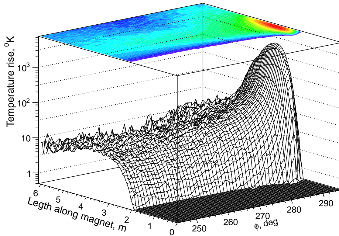
Figure 2-35: An instantaneous temperature rise along and across the dipole magnet beam pipe at accidental loss of entire beam.
