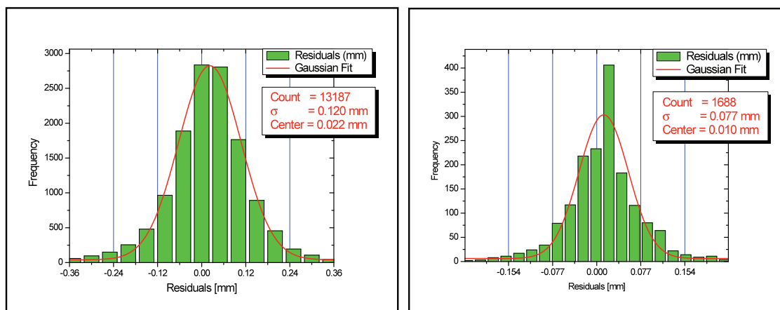
Figure 4-4: Distribution observation residuals for the Target and Near Detector Halls in MINOS
