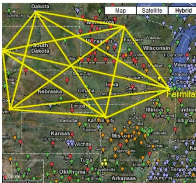
Figure 4-1: GPS network tying Fermilab and SURF to the CORS system
