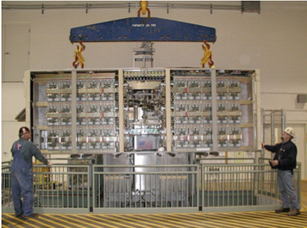
Figure 3–32: NuMI Capacitor Bank transport and installation, 2004.
