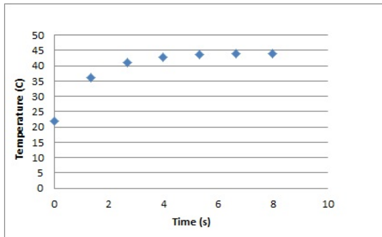
Figure 3-22: Temperature trends in the Horn 1 neck at beam cold start-up
