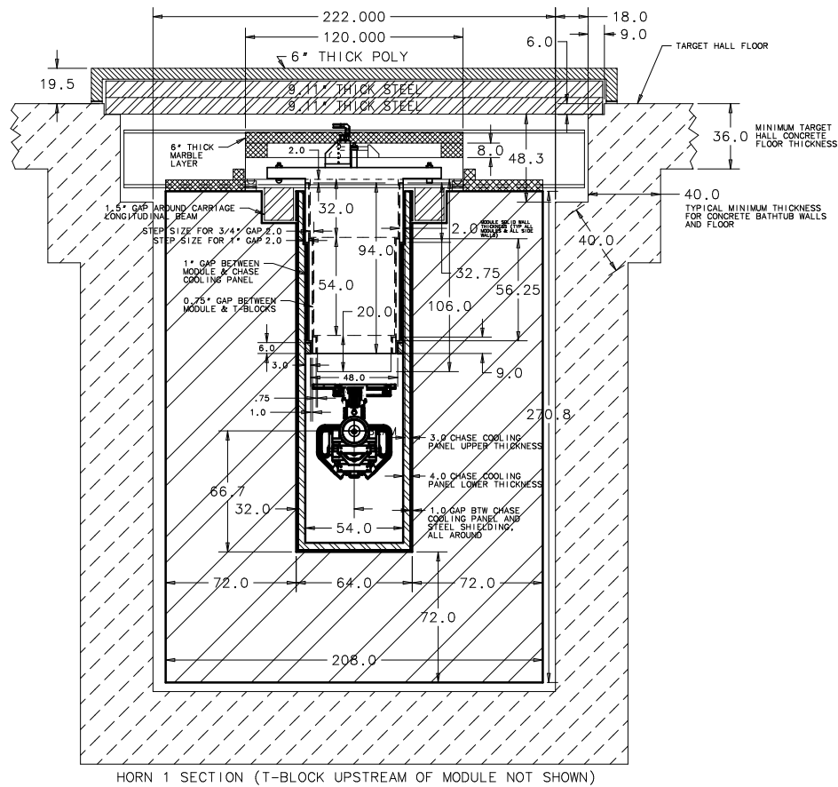
Figure 3-45: Cross section of target chase steel shielding (cross-hatched areas). The secondary beam is confined to the rectangular opening in the center
