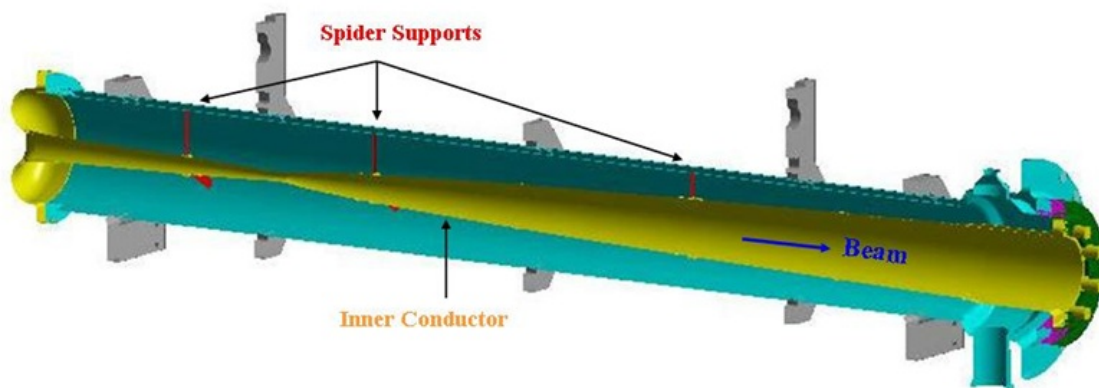
Figure 3–17: Additional support and stability for the thin inner conductor are provided by welded struts or "spider" (web) supports (thin red pieces).
