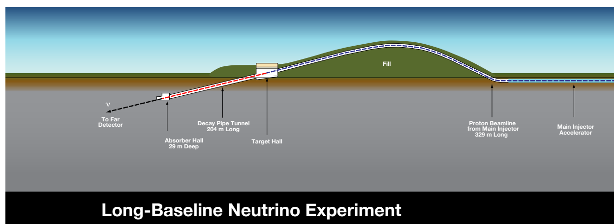
Figure 1–2: Schematic of the systems included in the LBNE Beamline. The top of the engineered hill is 18 m above grade.
