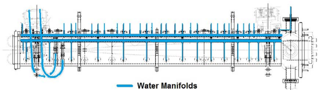
Figure 3–26: Horn cooling water manifolds.
