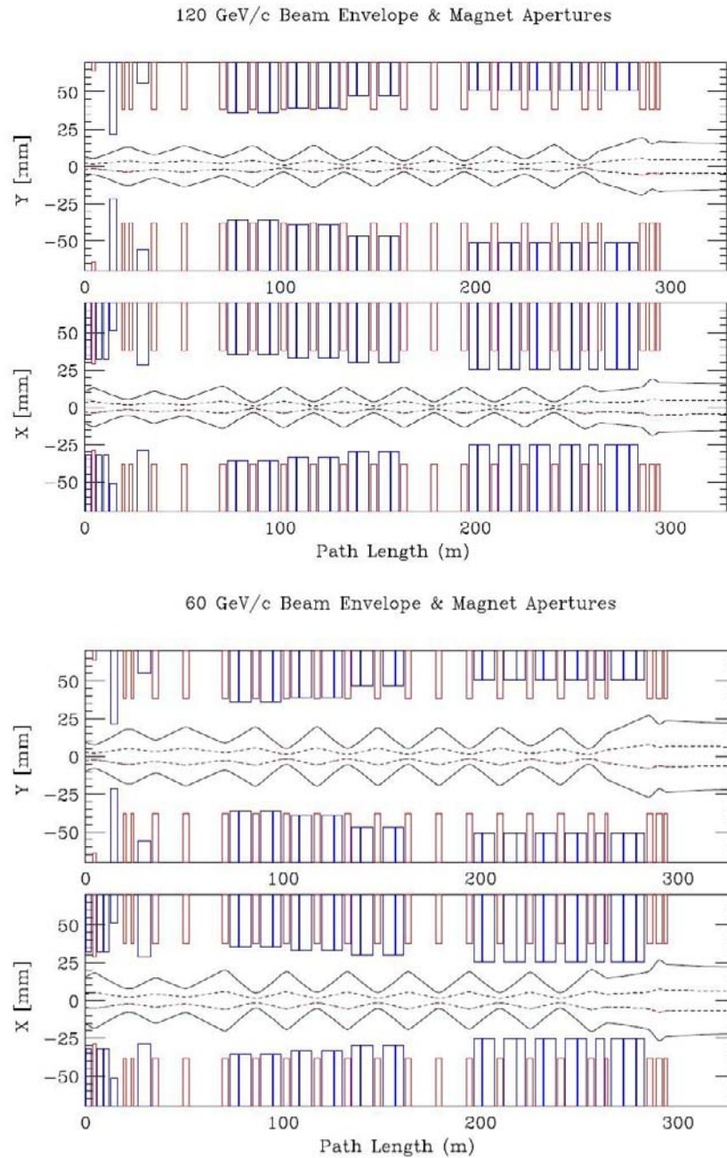
Figure 2-6: Magnet apertures and beam envelopes: The 99% contour (dashed) with nominal MI beam parameters, and the 100% envelope (solid) corresponding to the MI admittance at transition ( \gamma t = 21.600 ).
