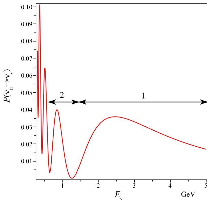
Figure 1-3: The energy range of the first and second oscillation peaks are denoted by the respective numerals. The beam design is optimized to produce neutrinos within this range. The true probability depends on a parameter, \theta_{13} .
