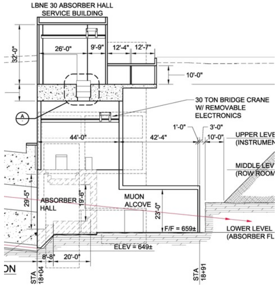
Figure 3-53: Absorber Hall section. The beam comes from the left. The downstream end of the decay pipe is bottom left.
