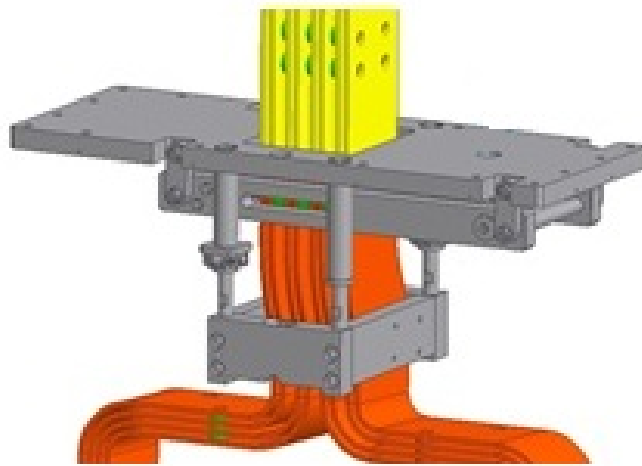
Figure 3–31: Stripline Block remote clamp assembly.
