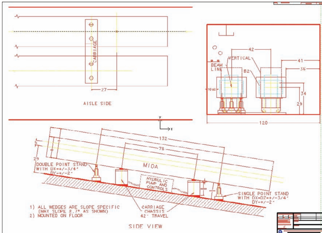
Figure 2-26: Magnet installation on sloping surfaces.
