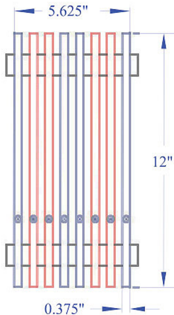
Figure 3–33: Stripline cross-section: 8 conductor (NuMI-style). Color indicates polarity of current. This design connects from the nine to eight layer transition to the horns.
