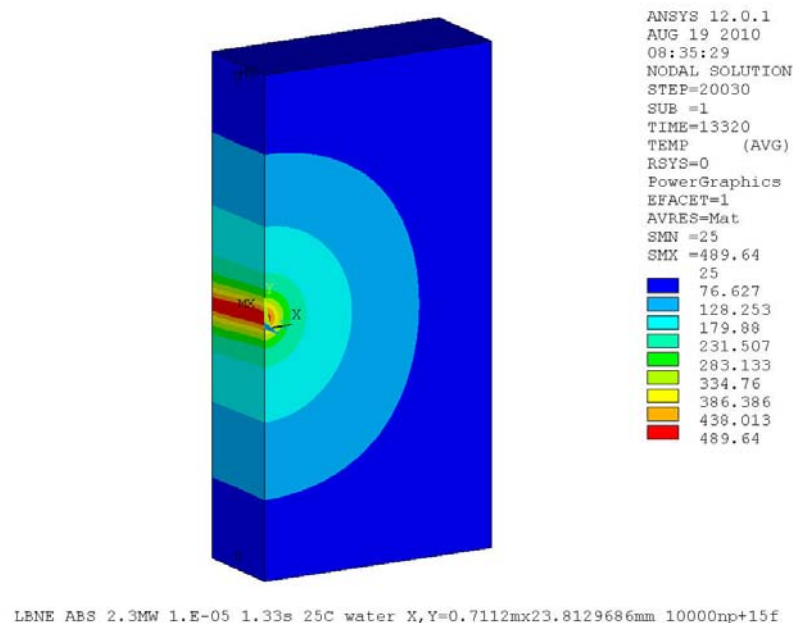
Figure 3-40: Temperature distribution in the Al absorber-core block. Fifteen beam pulses under the fault condition are superimposed on 10,000 normal ones. The maximum temperature in the center of the block is 490° C after 15 faulty pulses.
