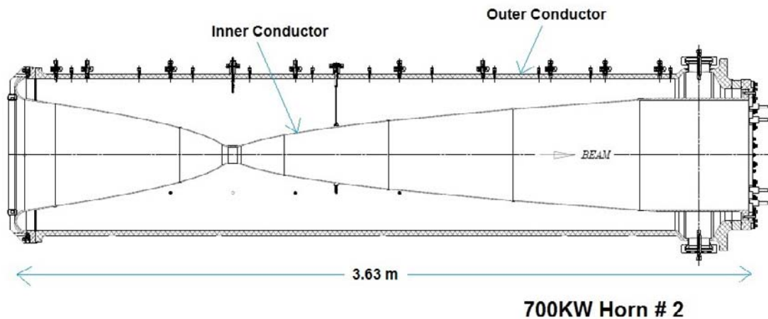
Figure 3-13: Horn 2 section. Horn 2 specifications are listed in Table 3-2.
