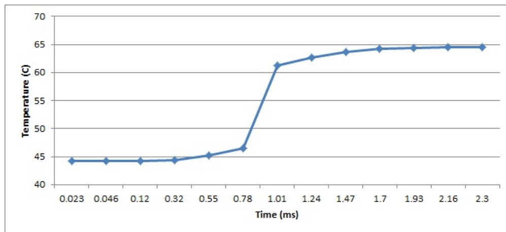
Figure 3-23: Temperature trends in the Horn 1 neck during a single pulse after equilibrium
