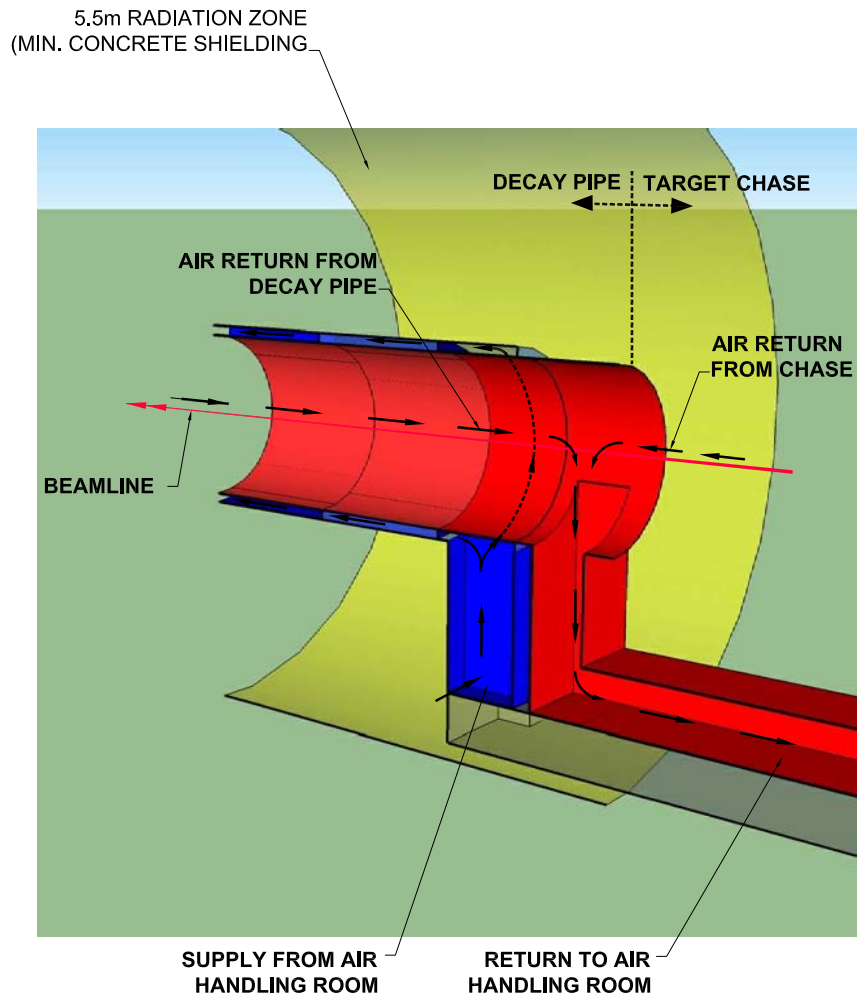
Figure 3-36: Section of the decay pipe at its upstream end. The airflow directions within the pipes are indicated.
