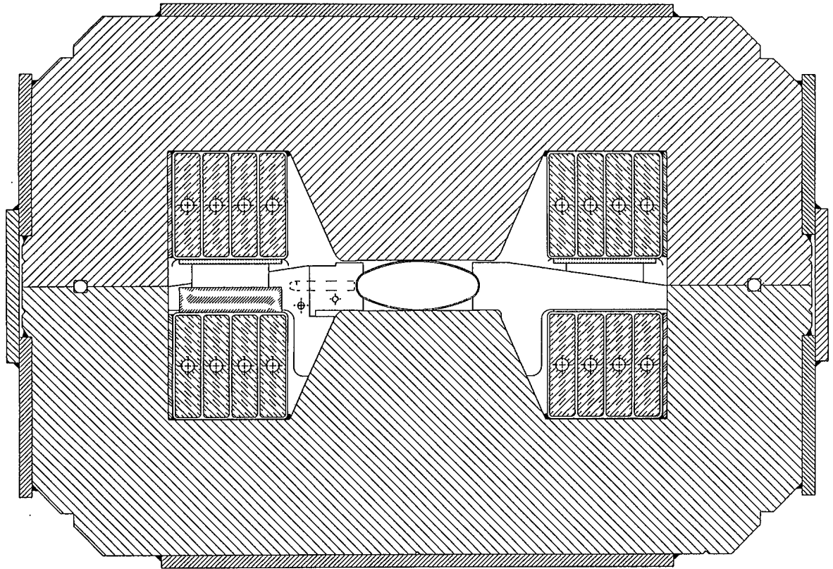
FMI DIPOLE TYPICAL CROSS SECTION
