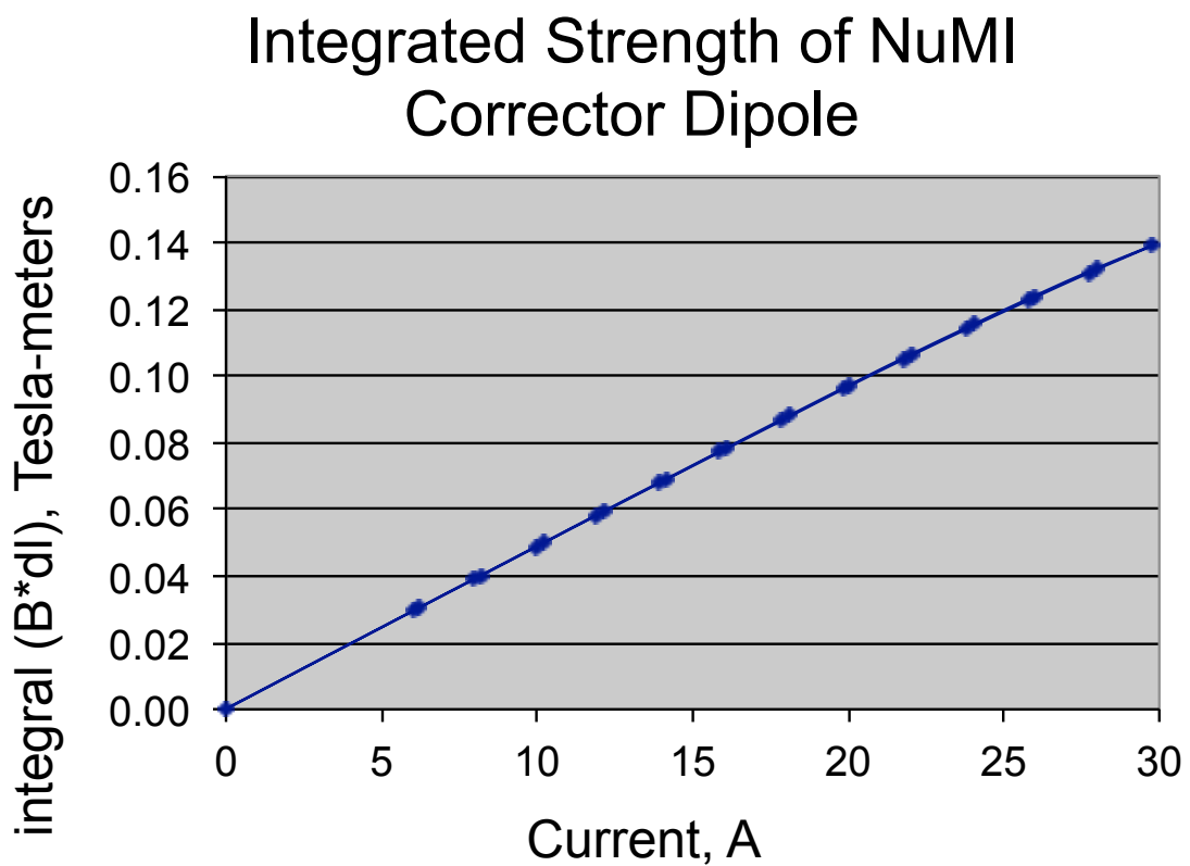
Figure 2-24: Integrated strength of NuMI dipole corrector.
