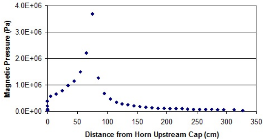
Figure 3–24: Magnetic pressure loading profile on the Horn 1 inner conductor at mid-pulse.
