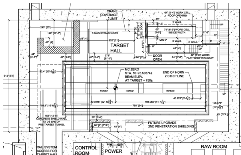
Figure 3-49: Target Complex Plan : expanded view of Figure 3-48
