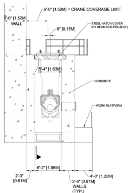
Figure 3-51: Target Hall work cell section, viewed from upstream
