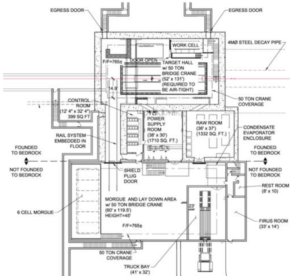
Figure 3-48: Target Complex Plan View
