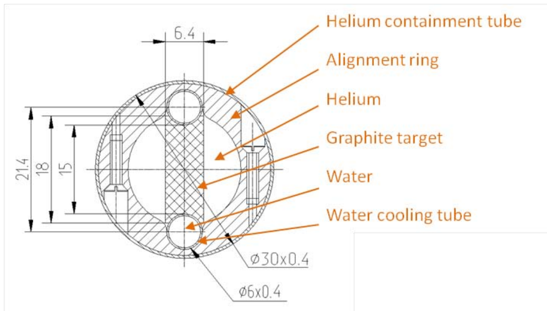
Figure 3–9: Cross-section of LT target for LBNE. Note the alignment rings do not run the full length of the target. Units are mm.
