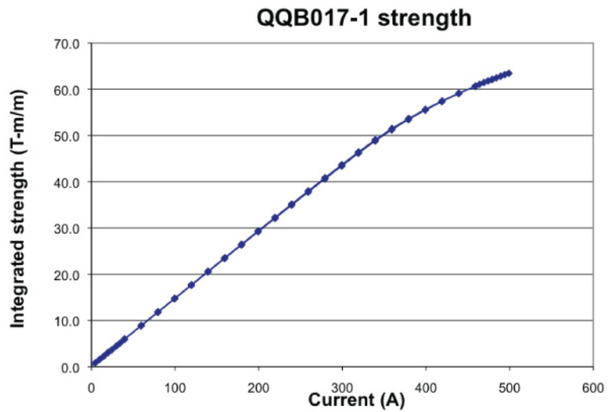
Figure 2–21: Typical QQB excitation curve.
