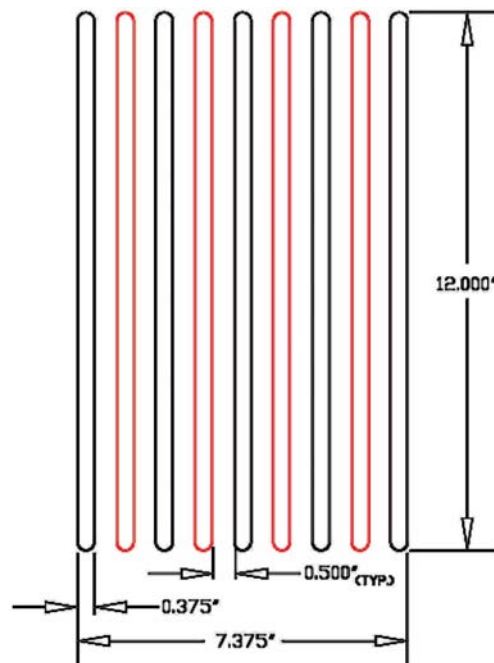
Figure 3-34: Stripline cross-section: 9 conductor. Color indicates polarity of current. This design will be installed from the power supply to the 8-conductor stripline transition in the chase.
