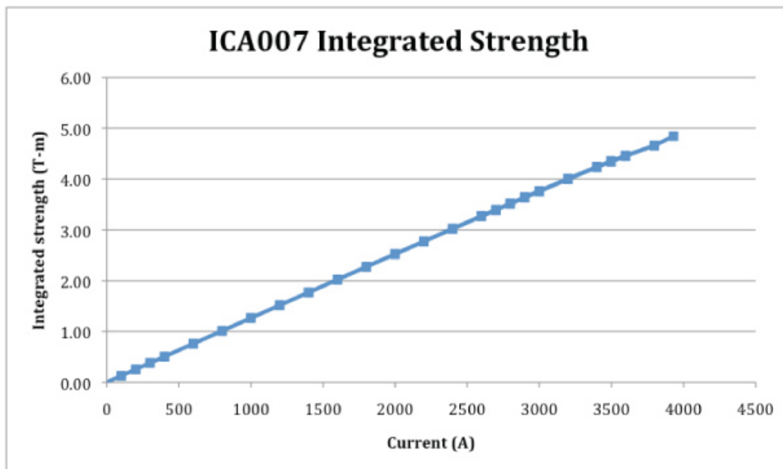
Figure 2-19: ICA integrated strength as a function of current.
