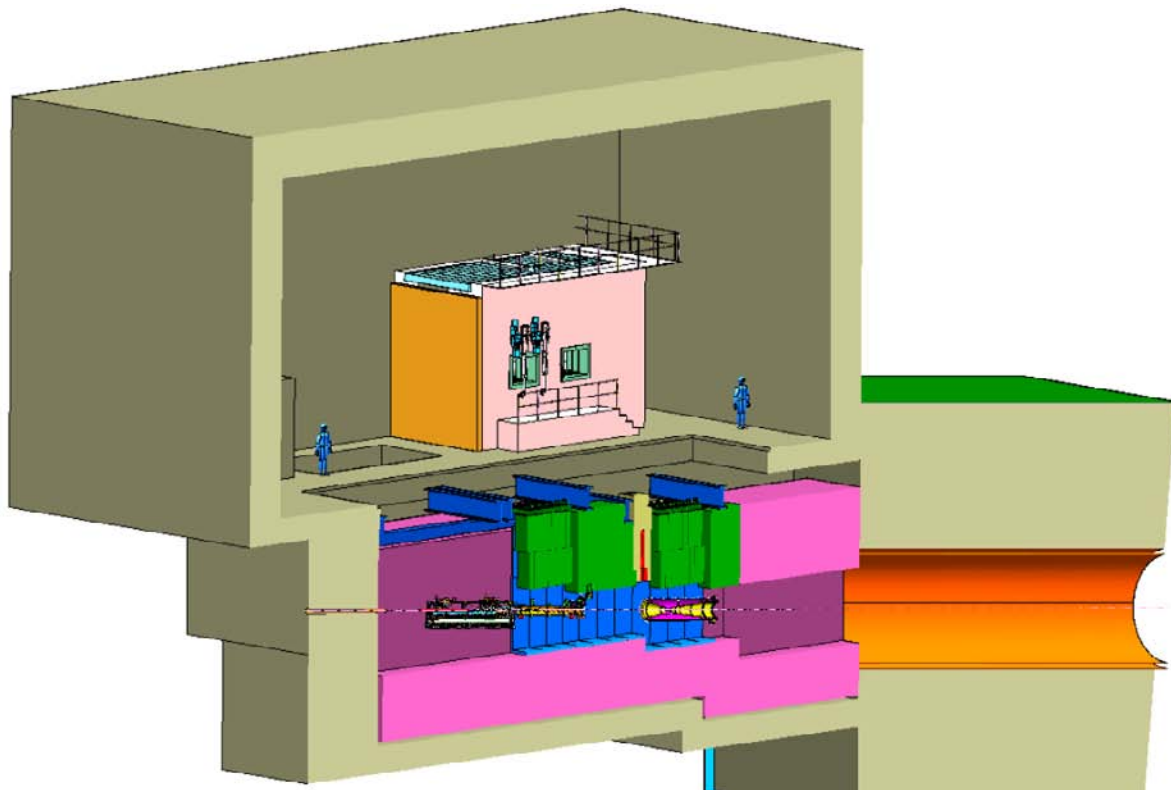
Figure 3-2: A cut view of an engineering model of part of the target complex, showing the relationship of the components depicted in Figure 3-1 to scale. The target chase shielding is shown by purple and green zones, the chase cooling panels are blue. The top of the chase shielding is removed. Above, and to the beam-left of the chase is the work cell. The start of the decay region is shown at the right. The absorber is not represented here.
