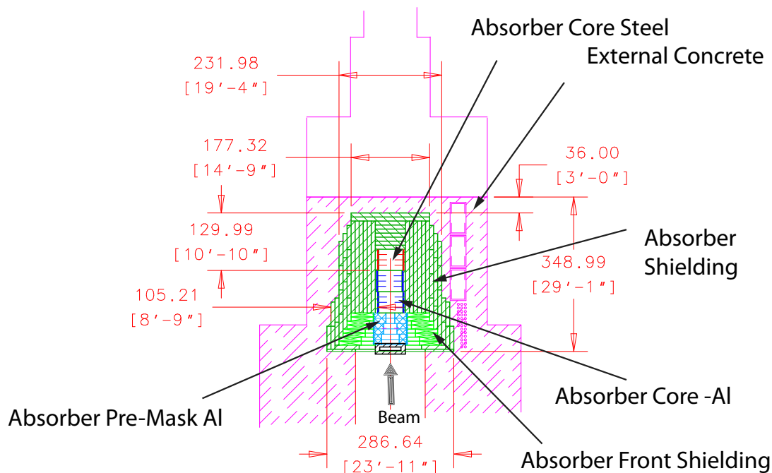
Figure 3-41: Model of the absorber conceptual design; top view. The core of water-cooled Al blocks is 96-in deep, followed by 130 in of steel (first 32 in are water-cooled) and 36 in of concrete at the rear. The routing of the cooling pipes is not shown.
