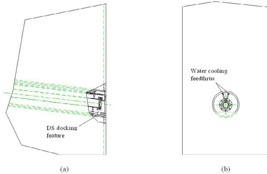
Figure 3-4: Section view of replacement window assembly. (b): End view of window assembly.
