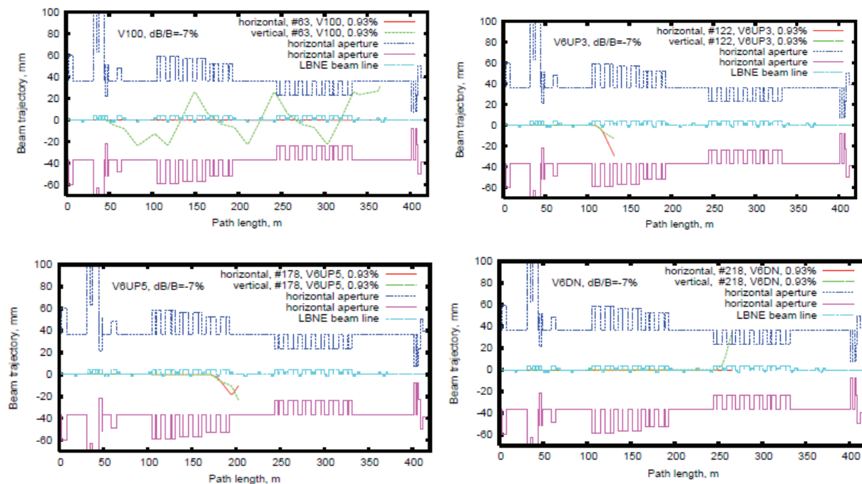
Figure 2-34: An example of beam trajectories along the beamline for a beam lost due to accidental degradation of bending magnet strength
