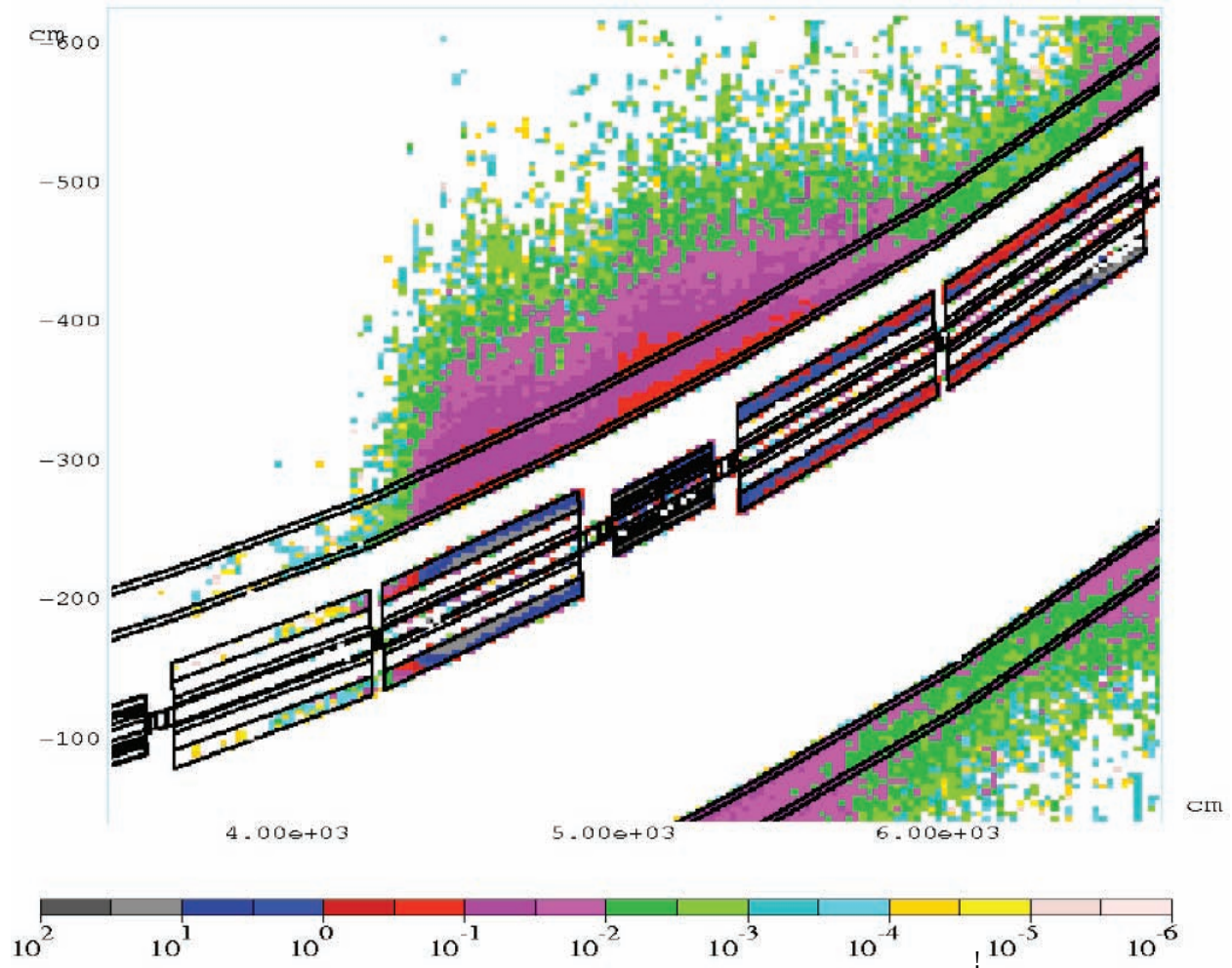
Figure 2-36: Residual dose rates along the beam line and magnets following a loss of 0.3% of the beam for 30 days followed by one day cool-down. The color-coded logarithmic scale has units of m-Sv/h (1 m-Sv/h is equivalent to 100 mrem/h)
