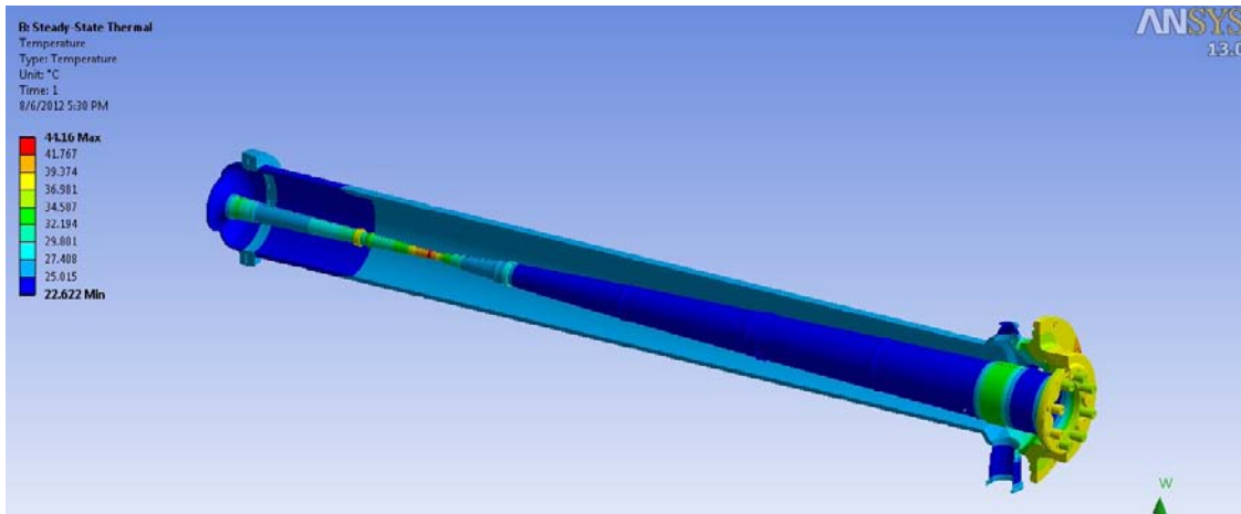
Figure 3-21: Temperature of Horn 1 at steady state
