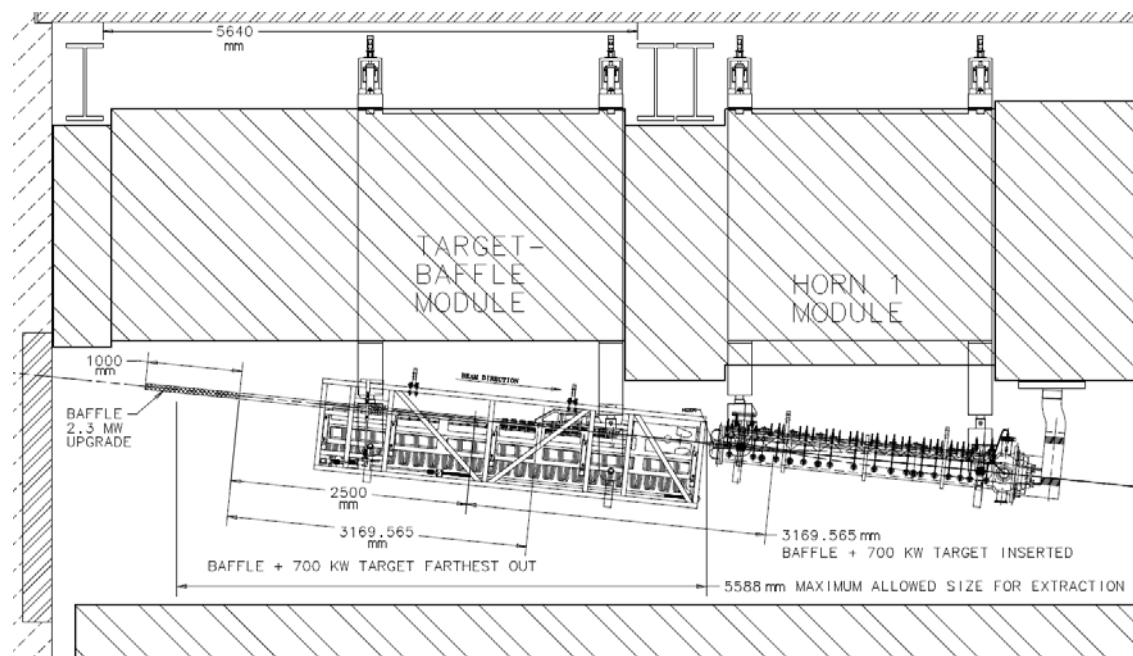
Figure 3-7: Target carrier in target pile shielding. The length of the baffle plus target assembly is shown in the fully inserted downstream position, and also in the furthest out position 2.5 m upstream of that. 5588 mm is taken as the maximum reasonable carrier length to extract between the carriage cross beams that are 5640 mm apart. The extra 1000 mm length of a baffle for 2.3 MW operation is also sketched in, showing that the usable range of target motion may be modestly reduced by that upgrade.
