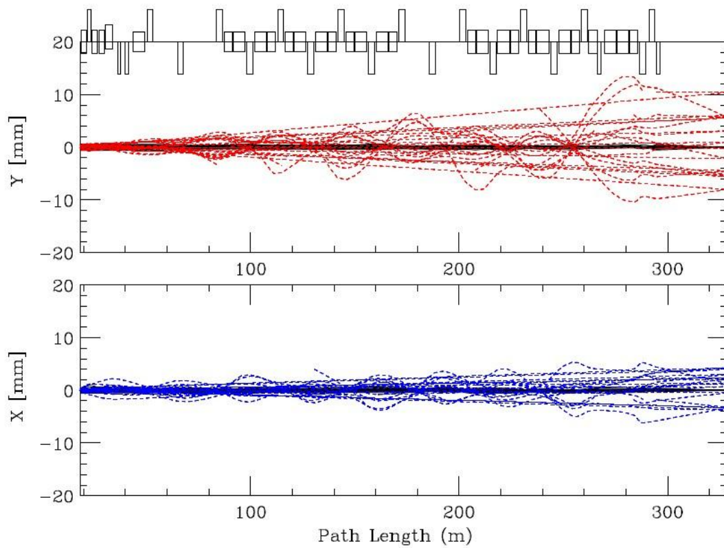
Figure 2-9: Uncorrected/corrected trajectories with random misalignments and dipole field errors; the plot begins at the upstream end of the first extraction Lambertson at MI-Q102
