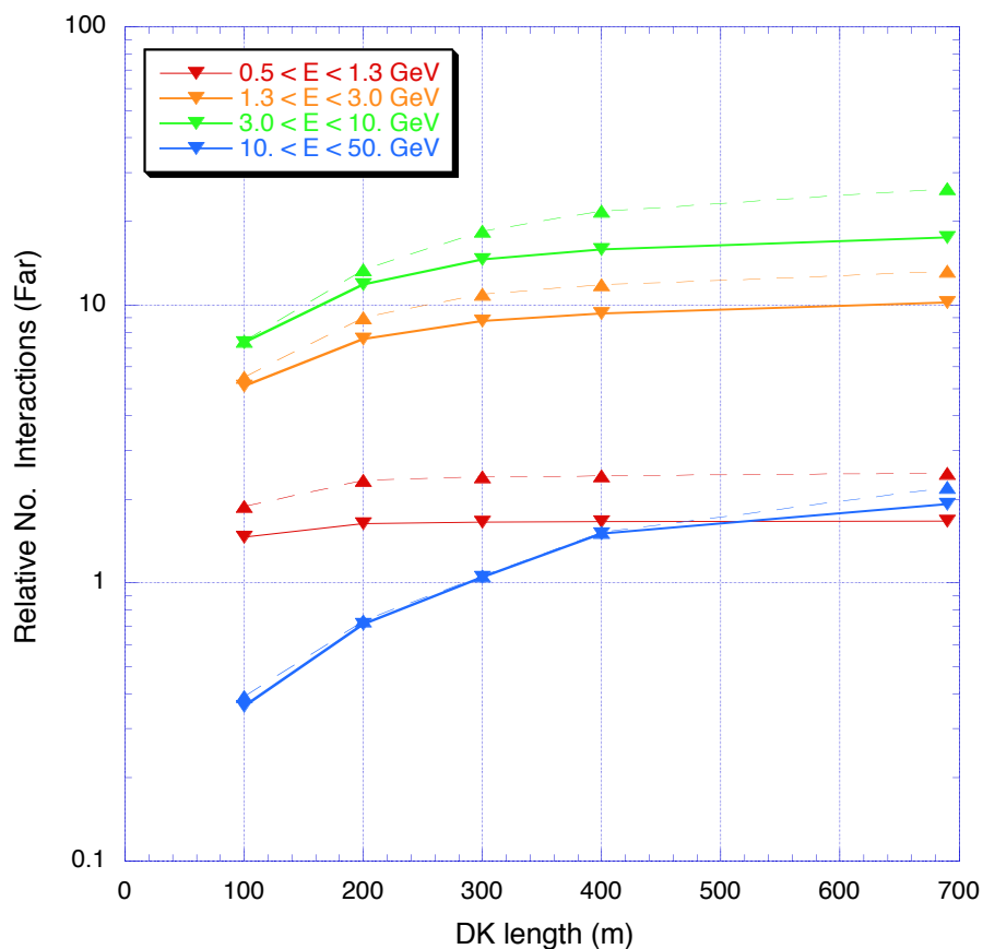
Figure 1-7: The number of neutrino interactions in the Far Detector depends on the length and diameter of the decay pipe. Here, the number of events is plotted as a function of length, with two curves for each colored energy range: solid is for a diameter of 2 m and dashed is for a diameter of 4 m. The reference design is a pipe 4 m in diameter and 203.7 m long.
