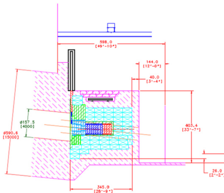
Figure 3-54: Absorber Hall section showing details of the absorber core and shielding arrangement. The aluminum core is colored dark blue. The shielding is shown in cyan and magenta. The beam comes from the left.
