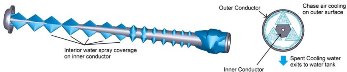
Figure 3–16: Horn 1 inner conductor water spray coverage.
