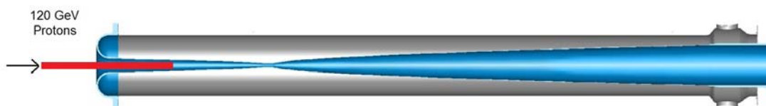
Figure 1-4: The first horn magnet. The conductor of the horn is shaded blue, and the graphite target (red) is inserted into the horn. The beam is incident from the left and the magnetic field region is between the shaped inner conductor and the cylindrical outer conductor (gray). Horn 1 is 336 cm long. The target is shown in the fully inserted position.
