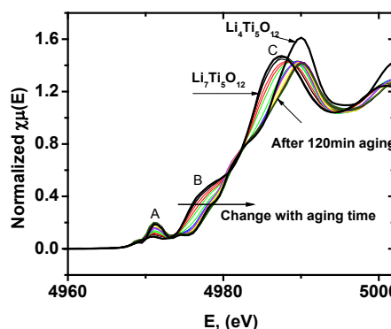
Figure IV - 106: Evolution of XANES spectra of Ti K-edge during aging at 60°C. The spectra were taken every 5 minutes.
