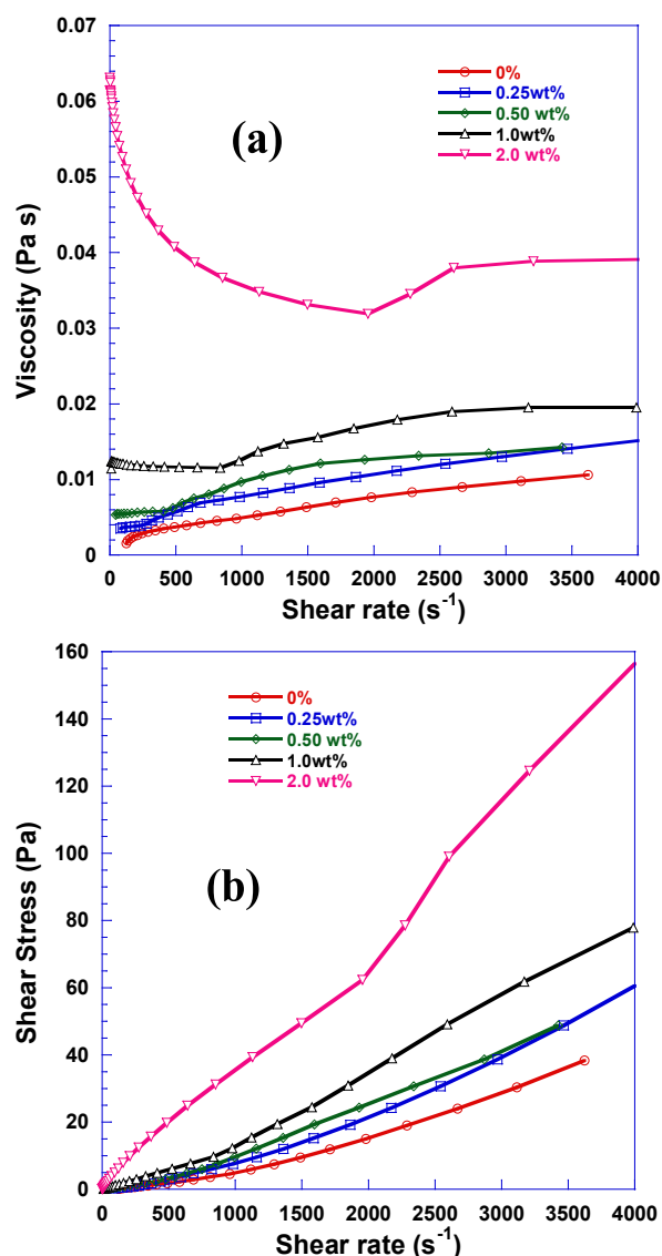
Figure IV - 80: Rheologic properties of aqueous NCM 523 suspensions with various CMC concentrations a) viscosity vs shear rate and b) shear stress vs shear rate.
