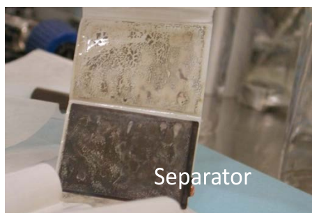
Figure IV - 252: A pouch cell being taken apart in the PTF.
