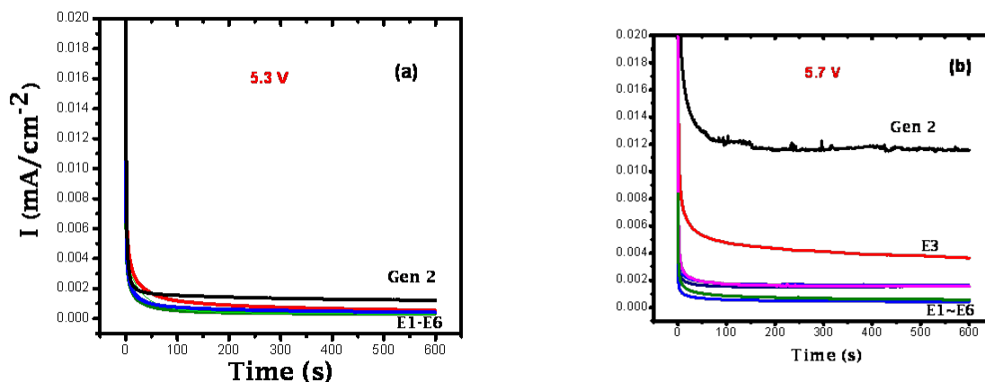
Figure IV - 152: Gen2 electrolyte and fluorinated electrolyte leakage currents at various potentials with Pt/Li/Li cell.
