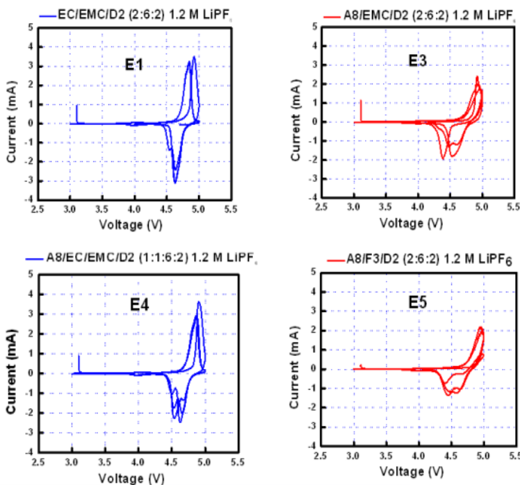
Figure IV - 154: Cyclic voltammetry profiles of LNMO/graphite cells using fluorinated electrolytes.
