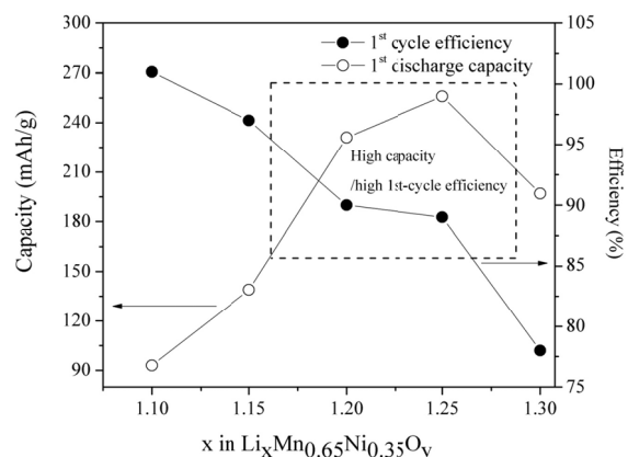
Figure IV - 139: Variation in capacity (mAh/g) and first-cycle efficiency (%) as a function of x in \text{Li}_x\text{Mn}_{0.65}\text{Ni}_{0.35}\text{O}_y electrodes.
