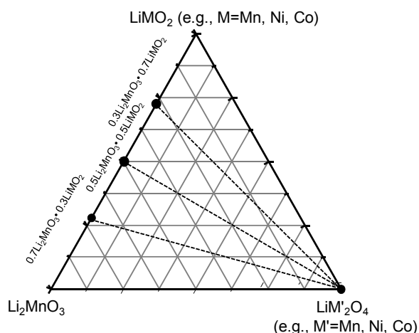
Figure IV - 30: A compositional phase diagram of a ‘layered-layered-spinel’ system with \text{Li}_2\text{MnO}_3 \cdot (1-x)\text{LiMO}_2 (‘layered-layered’) and \text{LiM}'_2\text{O}_4 (spinel) components.
