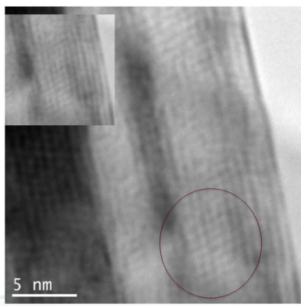
Figure IV - 137: TEM of IE-LNMO showing the spinel regions in the marked circle.
