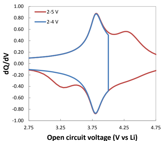
Figure IV - 185: Initial simulation of hysteresis in LMR-NMC OCV curves.
