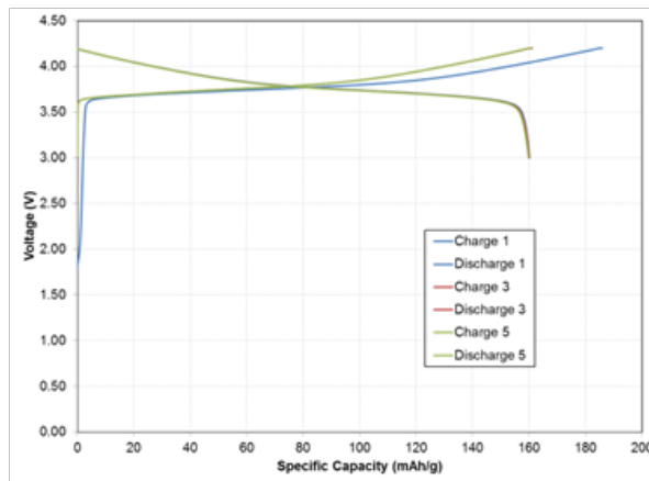
Figure IV - 223: Round robin NMC 523 cathode performance during formation cycling.
