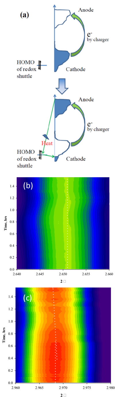
Figure IV - 222: (a) Schematic energy diagram illustrating the potential heat generation at the anode side. In situ HEXRD profiles of a \text{Li}_4\text{Ti}_5\text{O}_{12}/\text{LiMn}_2\text{O}_4 cell during overcharge test showing the lattice variation of (b) Al and (c) Cu. The electrolyte was 0.4 M \text{Li}_2\text{B}_{12}\text{F}_9\text{H}_3 in EC/EMC (3:7, by weight). The current was 0.2 A ( \sim 1\text{C} ).
