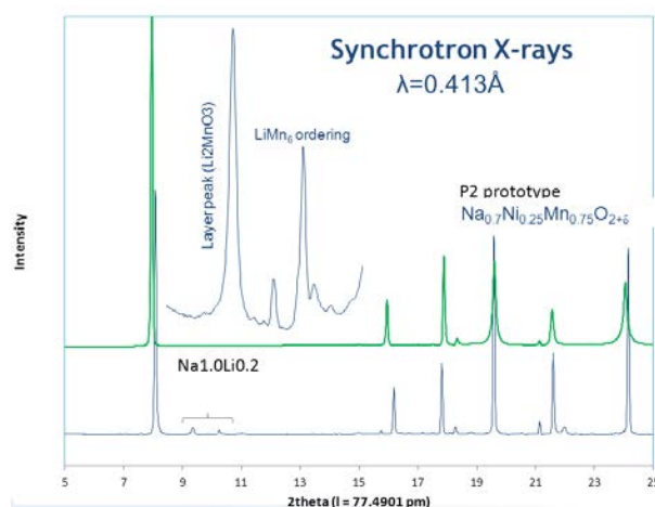
Figure IV - 127: X-ray powder diffraction patterns measured using a synchrotron source. Bottom pattern is \text{Na}_{1.0}\text{Li}_{0.2}\text{Ni}_{0.25}\text{Mn}_{0.75}\text{O}_y and the top is synthesized \text{Na}_{0.7}\text{Ni}_{0.25}\text{Mn}_{0.75}\text{O}_y to show the clean pattern for non-Li P2 precursor.
