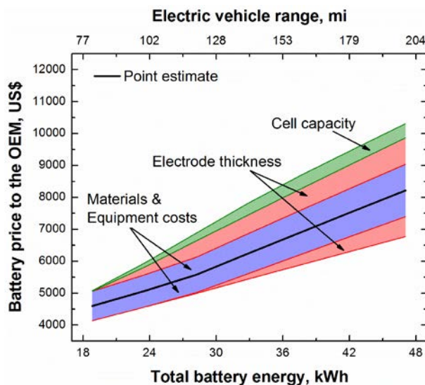
Figure IV - 188: Effects of electric-vehicle range on price and error bars for battery pack with NMC441-Gr cell chemistry, 120-kW 360 V.
