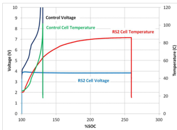
Figure IV - 227: Overcharge abuse behavior of control cells (18650, nom. 1 Ah) as well as cells containing 0.2 M RS2 overcharge shuttle additive.
