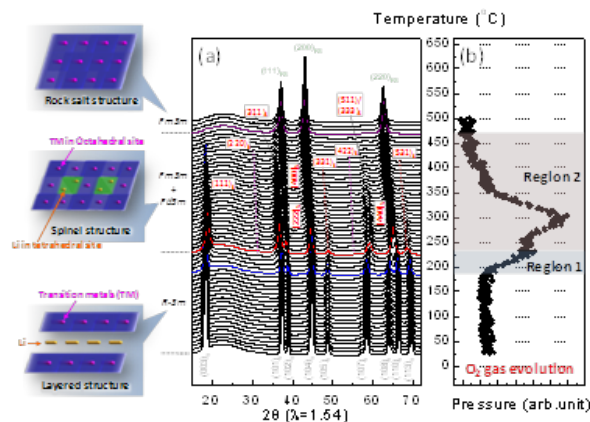
Figure IV - 210: (a) Time-resolved (TR) XRD patterns, and, (b) results from simultaneously measured mass spectroscopy (MS) that trace oxygen gas released from the overcharged \text{Li}_{0.33}\text{Ni}_{0.8}\text{Co}_{0.15}\text{Al}_{0.05}\text{O}_2 during heating up to 500 °C. The cathode sample in a glass tube was heated from 25- to 500-°C for 4 h during the TR-XRD and MS measurements (heating rate = 2.0 °C min -1 ). Left panel shows the ideal crystal-structure models for rhombohedral-, spinel-, and rock-salt-structures.
