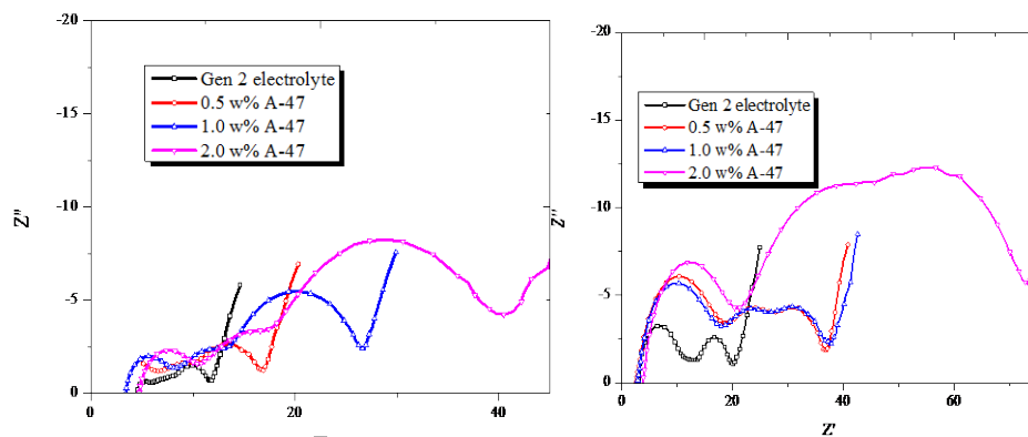
Figure IV - 148: AC impedance profiles of MCMB/NCM coin cells in 3E7EMC/PF12 with none or various amount of TPP (A-47) before (left) and after (right) 200 cycles under 55 °C at 1C rate. The cells were charged to 3.8 V. The charge rate was 1C.
