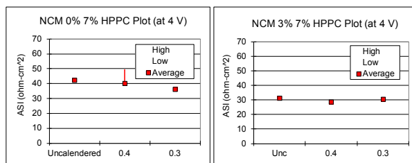
Figure IV - 57: ASI of NCM electrode with and without carbon coating.
