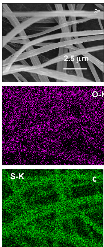
Figure IV - 236: SEM image a) and EDS maps of oxygen b) and sulfur c) of a P3BT and PEO composite prepared by electrospinning.
