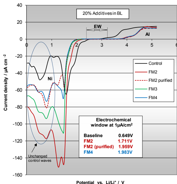
Figure IV - 176: The effect of INL FM-series phosphazene additives on the electrochemical window of the baseline electrolyte.
