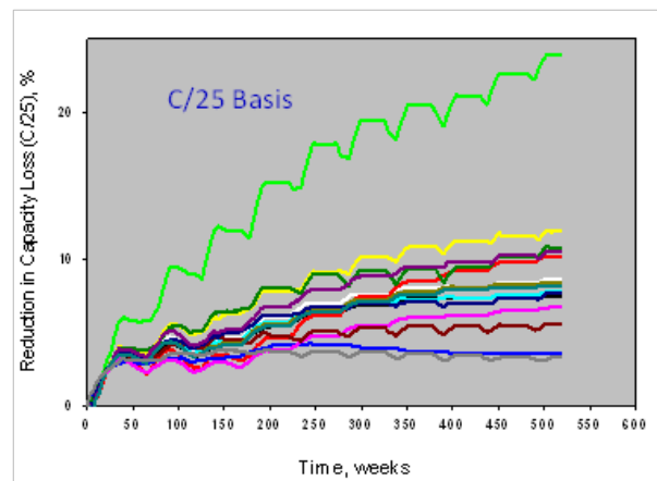
Figure IV - 208: Reductions in Capacity Loss with more aggressive thermal management.
