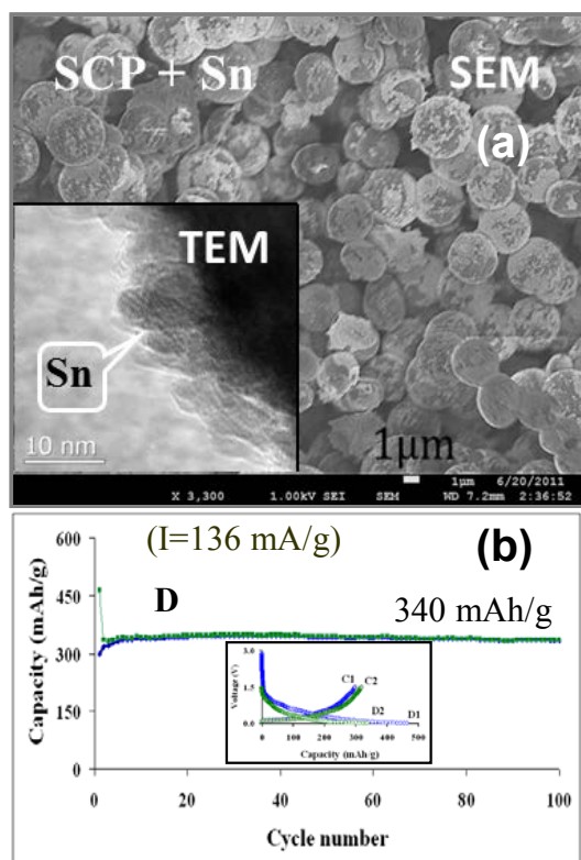
Figure IV - 102: a) SEM and TEM (inset) of Sn-coated carbon spheres and b) First and second discharge-charge- profiles (inset) and capacity vs. cycle number plot of a lithium half-cell with Sn-carbon sphere electrodes between 1.5 V and 0.01 V at a C/2.7 rate.
