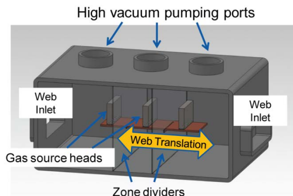
Figure IV - 64: Initial design of an in-line ALD reactor for deposition on porous substrates.
