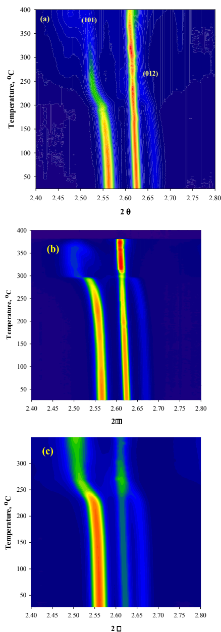
Figure IV - 219: Contour plot of in situ HEXRD data during thermal decomposition of delithiated NMC with the presence of (a) 1.2 M \text{LiPF}_6 in EC/EMC (3:7, by weight), (b) EC/EMC (3:7, by weight), and (c) 1.0 M LiTFSI in EC/EMC (3:7, by weight).
