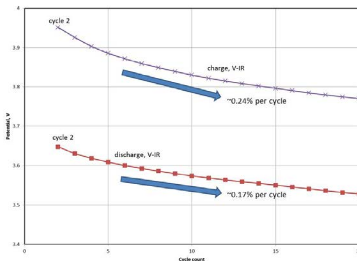
Figure IV - 3: Resistance-corrected average cell potentials plotted versus cycle number. A continuous drop in average potential exceeding 0.1V is apparent during charging and discharging. The drop in average charge potential is larger than the drop in the average discharge potential. The average potential is calculated by dividing the measured total energy (current x time x voltage) by the measured cell capacity (current x time).
