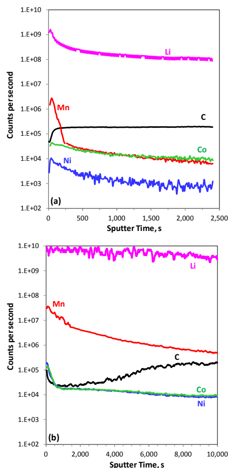
Figure IV - 196: SIMS sputter depth profiles from negative electrodes after (a) characterization cycles, and (b) 1500 cycles. Data for carbon, manganese, nickel, cobalt and lithium are shown. The Y-axis scales are the same for (a) and (b), but the X-axis scales are different.
