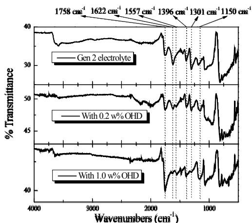
Figure IV - 144: FTIR spectra of MCMB electrodes obtained from MCMB/NCM coin cells containing different amounts of OHD in electrolyte of 1.2M LiPF 6 with EC/DEC (3:7 weight ratio) after formation cycles.
