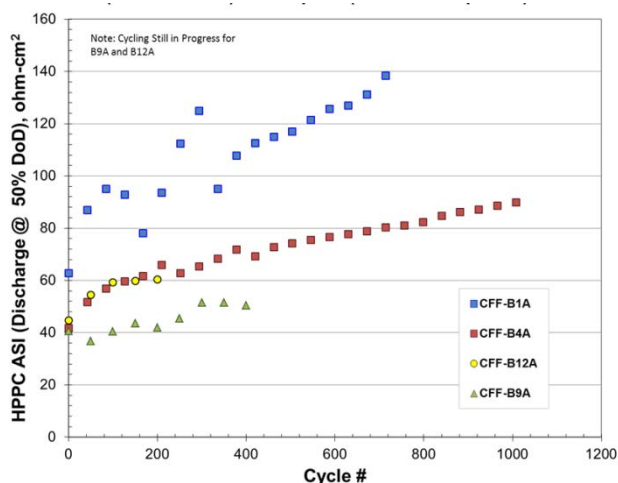
Figure IV - 271: HPPC impedance summary of cell builds based on Toda HE5050 high energy cathode materials vs. ConocoPhillips A12 graphite.
