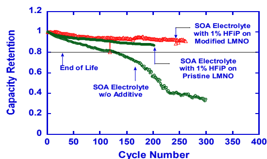
Figure IV - 158: Capacity as a function of cycle number plots at room temperature LMNO half cells in 1 M LiPF 6 /EC:EMC (30:70) with HFiP. Baseline electrolyte was also used as benchmark.
