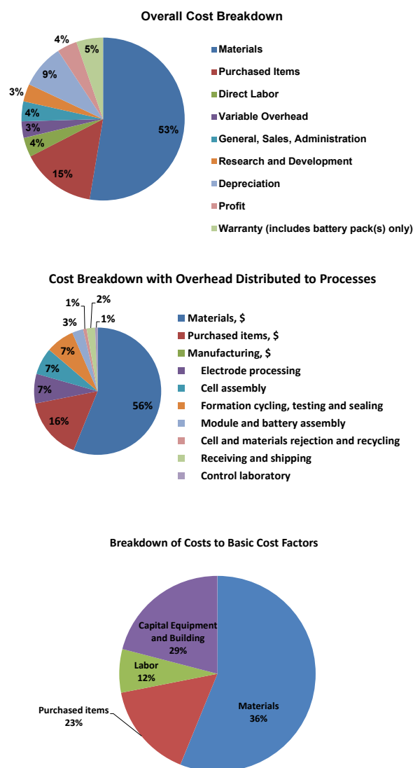
Figure IV - 189: a) Cost breakdown for a PHEV40, b) overhead distributed to processes, and c) summarized in basic cost factors.
