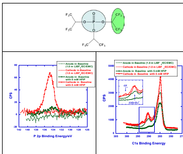
Figure IV - 160: Sub-structures of HFiP (a), and HR-XPS of cycled anode (b) and cathode (c) surfaces in baseline and HFiP-based electrolytes.
