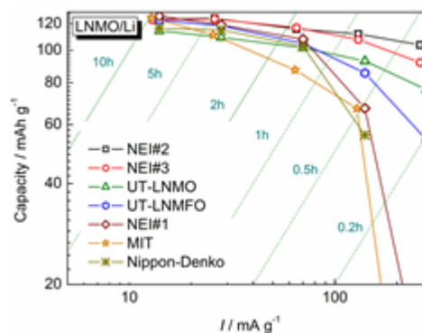
Figure IV - 40: Rate performance of \text{LiNi}_{1/2}\text{Mn}_{3/2}\text{O}_4 materials.
