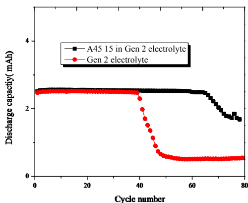
Figure IV - 151: Capacity retention of Li/LNMO coin cells in 3E7EMC/PF12 with none or 1 wt % additives. The cells were cycled at room temperature. The charge rate was C/5 (1mA). The cut-off voltages were 3.5 ~ 4.95 V.
