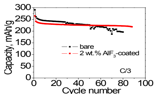
Figure IV - 112: Cycling performance of \text{AlF}_3 coated and uncoated (bare) high energy cathode at 55 ^{\circ}\text{C} .
