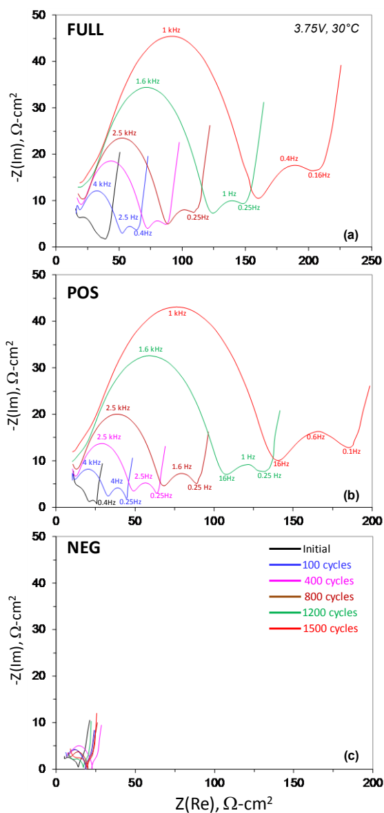
Figure IV - 191: AC impedance data from (a) the full cell, and from the (b), (c) positive and negative electrodes showing changes that result from cell cycling. The data were obtained at 30\text{ }iC , at a full cell voltage of 3.75\text{ V} , in the 100\text{ kHz} to 0.01\text{ Hz} frequency range.
