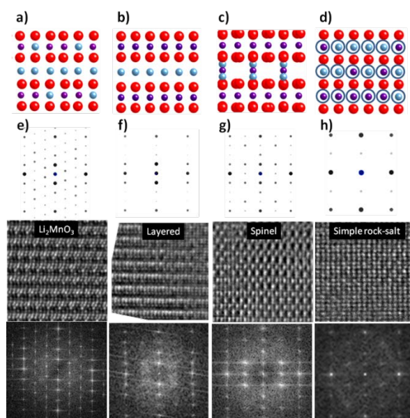
Figure IV - 21: Crystal structure models for \text{Li}_x\text{TMO}_2 phases; (a) \text{Li}_2\text{TMO}_3 (110 plane), (b) layered (1-100), (c) spinel (112) and (d) simple rock-salt (112). Oxygen is drawn as red, TM as purple, and Li as blue. The atom columns with circles represent randomly mixed Li/TM columns. The corresponding experimental electron diffraction patterns, high resolution images, and Fourier Transform patterns from the high resolution images are shown under each crystal model (e-h).
