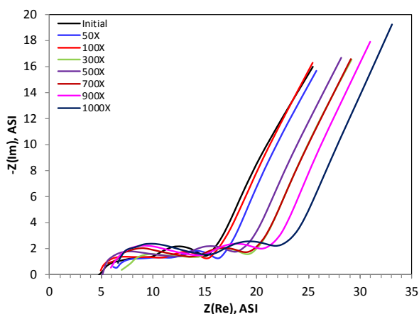
Figure IV - 197: EIS data from a \text{Li}_{1.2}\text{Ni}_{0.15}\text{Mn}_{0.55}\text{Co}_{0.1}\text{O}_2 /Graphite cells containing the LiDFOB electrolyte additive.
