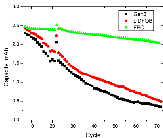
Figure IV - 264: Cycle performance of Silicon half cell with and without additives.
