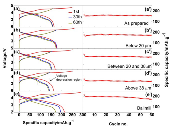
Figure IV - 49: Electrochemical performance of cells prepared with cathodes with different particle sizes: left, voltage-capacity profile; right, cycling performance.
