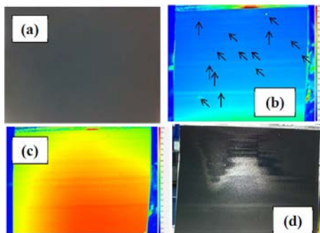
Figure IV - 86: Homogeneity and defect analysis of \text{LiFePO}_4 electrode coating: visual digital image (a), IR image (b), temperature profile (c), and image taken when quartz lamp is viewed through the electrode (d).
