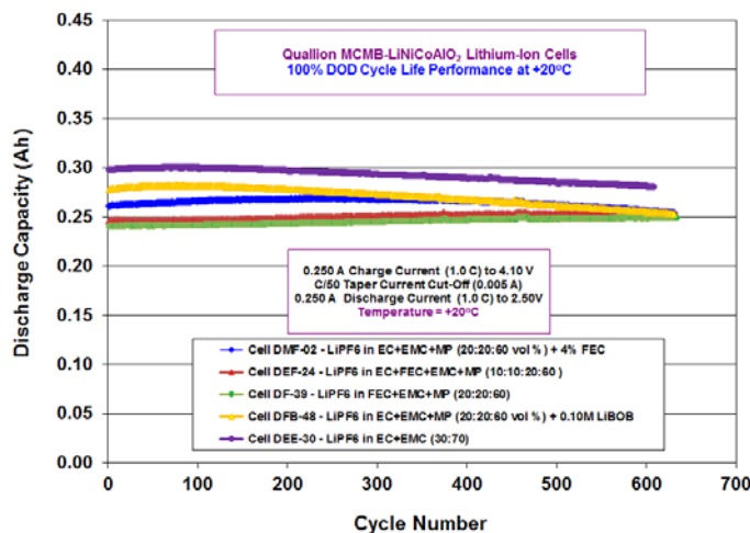
Figure IV - 171: Cycle life performance of 0.25Ah MCMB-LiNiCoAlO 2 cells (Quallion, LCC) containing various electrolytes at 20°C, using C rate charge and discharge over a voltage range of 2.50V to 4.10V.
