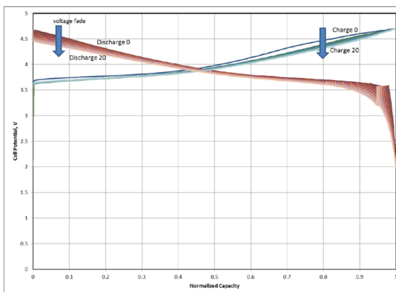
Figure IV - 5: Capacity-normalized voltage profiles for NCM333. Some voltage fade is apparent over all charge states and discharge depths.
