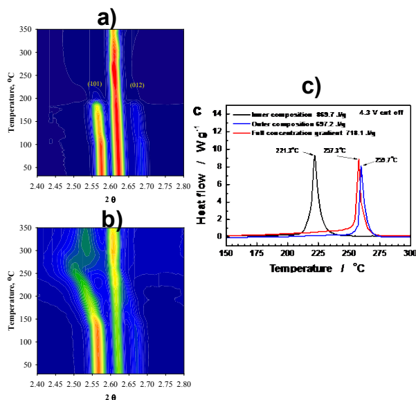
Figure IV - 124: a) Contour plots of in situ high energy X-ray diffraction profile. a, delithiated inner composition material [Li 1-x Ni 0.86 Co 0.10 Mn 0.04 O 2 ] and b), delithiated full concentration gradient material during thermal ramping from room temperature to 375 °C with a scanning rate of 10 °C min -1 . c), differential scanning calorimetry profiles of the delithiated full concentration gradient material, the delithiated inner composition [Li 1-x Ni 0.86 Co 0.10 Mn 0.04 O 2 ], and the delithiated outer composition [Li 1-x Ni 0.70 Co 0.10 Mn 0.20 O 2 ] with a scanning rate of 1 °C min -1 . The cells were constant-voltage charged to 4.3 V vs. Li + /Li before disassembling.
