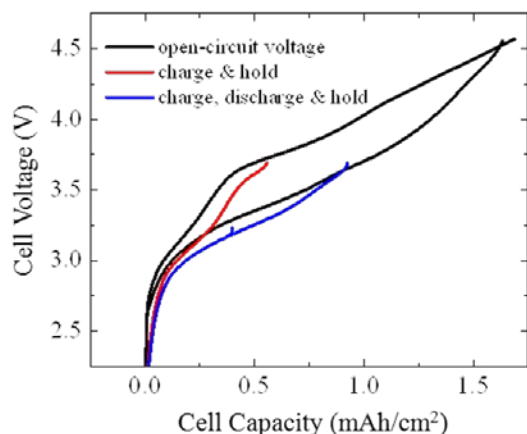
Figure IV - 16: Measured open circuit voltages at 3.7V on charge (red) and discharge (blue) after a 7 day potentiostatic hold for \text{Li}_{1.25}\text{Ni}_{0.33}\text{Mg}_{0.02}\text{Mn}_{0.65}\text{O}_y .
