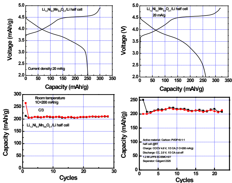
Figure IV - 118: First charge and discharge cycle and capacity vs cycling of cells based on cathodes made by the hydroxide and the carbonate process.
