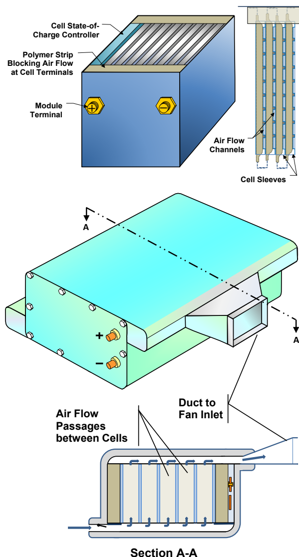
Figure IV - 187: New module (top) and pack (bottom) design for batteries utilizing air thermal management in BatPaC.
