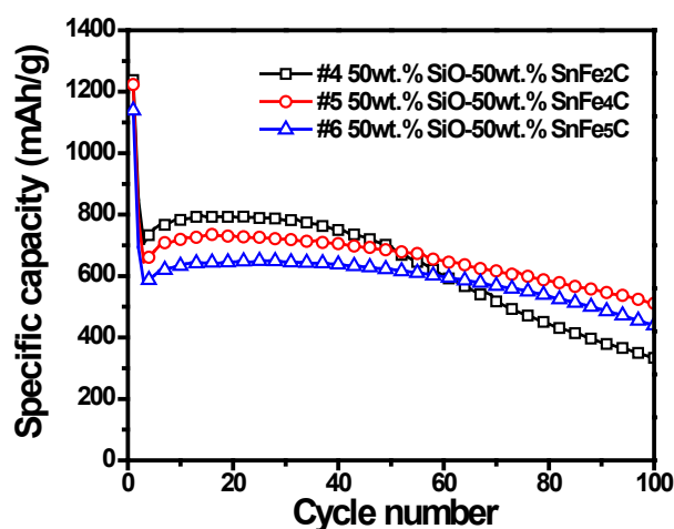
Figure IV - 99: Cycle performance of different compositions.
