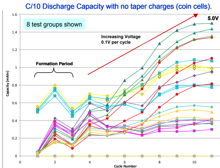
Figure IV - 175: Coin cell capacity data for the first generation INL alternative anode formulations based on phosphazene polymer host.
