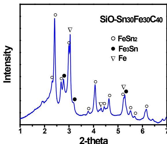
Figure IV - 100: XRD pattern of SiO-Sn 30 Fe 30 C 40 .
