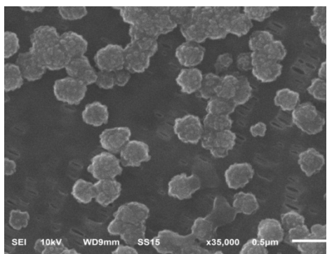
Figure IV - 257: SEM micrograph of the anode side of the separator.
