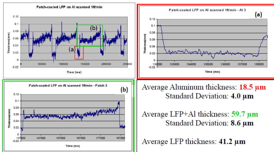
Figure IV - 84: Thickness measurement of \text{LiFePO}_4 electrode on Al foil.
