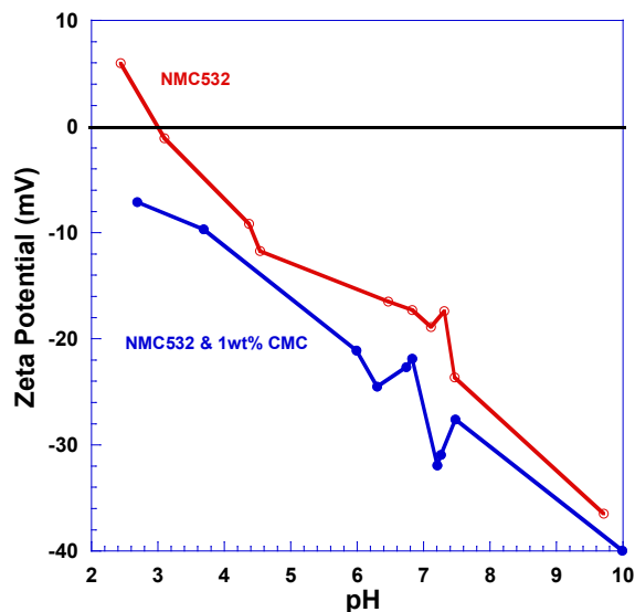
Figure IV - 79: Zeta potential of NCM 523 with and without CMC; the addition of 1 wt% CMC resulted in a more negative charge on the NCM 523 surface.
