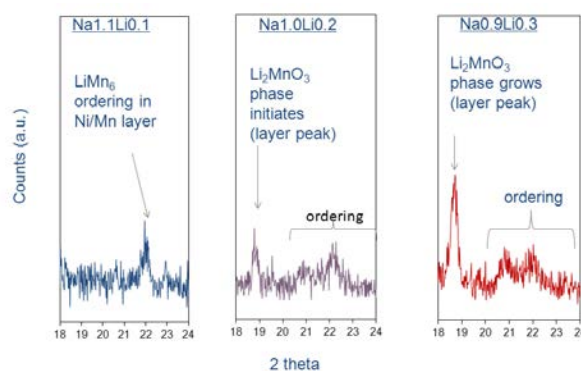
Figure IV - 126: X-ray powder diffraction patterns magnified between 18 and 24 degrees \text{CuK}\alpha 2-theta of \text{Na}_a\text{Li}_b\text{Ni}_{0.25}\text{Mn}_{0.75}\text{O}_y precursor.
