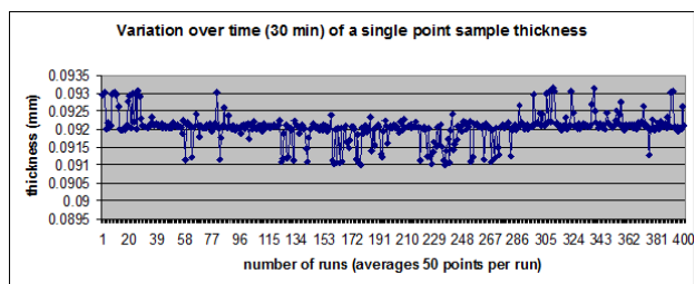
Figure IV - 83: Baseline noise determination from using calibration shim.
