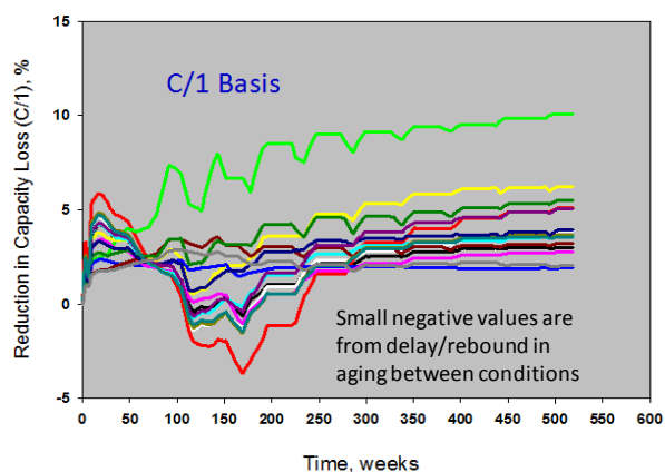
Figure IV - 209: Reductions in Capacity Loss with more aggressive thermal management (cont'd).
