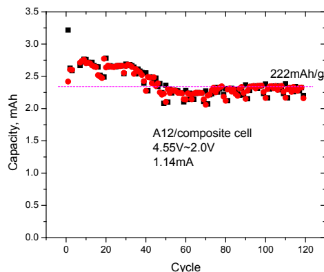
Figure IV - 259: Cycle performance of HE5050 full cell.
