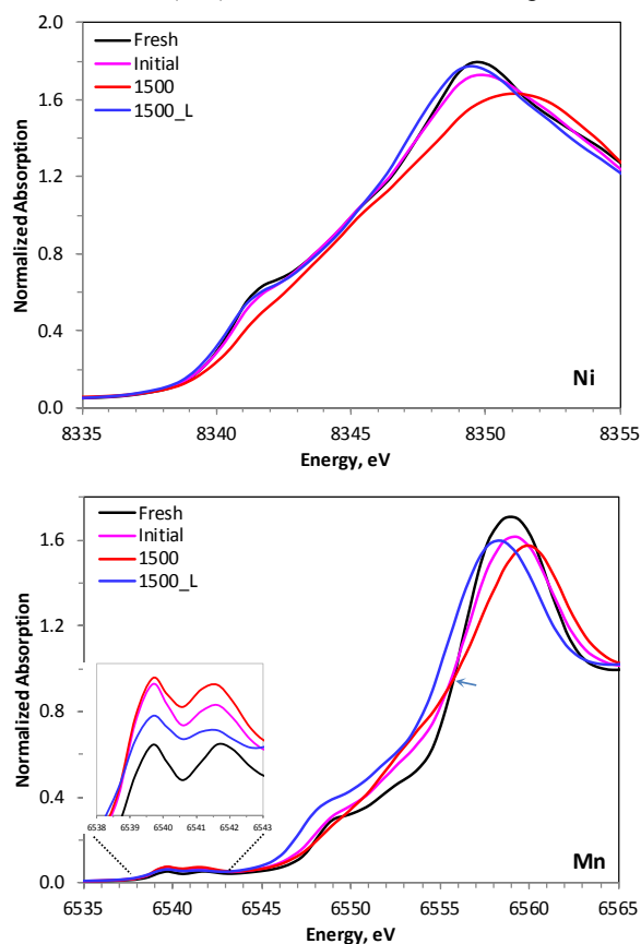
Figure IV - 194: XAS data at the Ni K-edge and Mn K-edge for a fresh positive electrode and for electrodes harvested from cells after initial cycles and after 1500 cycles. The 1500_L data is from a "relithiated" 1500_cycle electrode.
