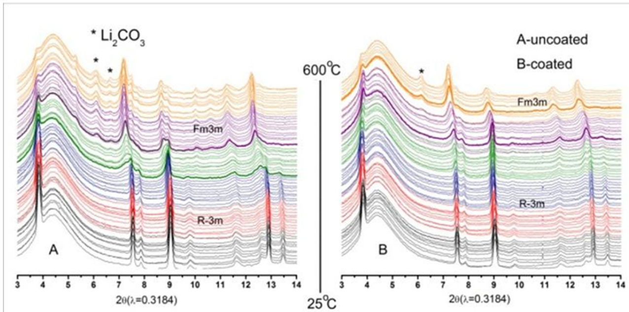
Figure IV - 213: Crystal structure changes of fully charged cathode material \text{Li}_{1.2}\text{Ni}_{0.17}\text{Co}_{0.07}\text{Mn}_{0.56}\text{O}_2 with (B) and without (A) \text{Al}_2\text{O}_3 ALD coating studied by TR-XRD during heating from 25 °C to 600 °C.
