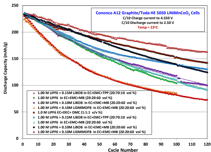
Figure IV - 172: Cycle life performance of Cononco A12 graphite/Toda HE 5050 LiNiCoMnO 2 cells containing containing various electrolytes (Fig. 2B).
