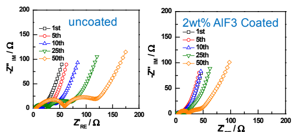
Figure IV - 113: AC Impedance of cells based on coated and uncoated high energy cathode material.
