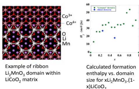
Figure IV - 12: Example \text{Li}_2\text{MnO}_3 Domain within \text{LiCoO}_2 Matrix.
