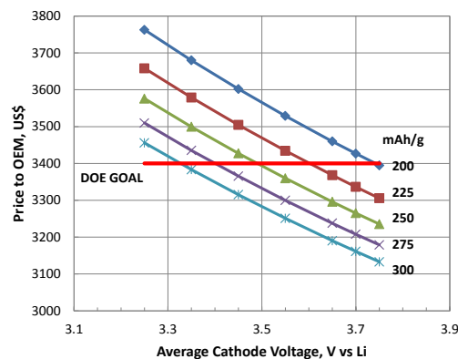
Figure IV - 8: Battery Price to OEM for an advanced Li-ion anode with LMR-NMC cathodes with varying capacities as a function of cathode OCV for (left) an EV150 compared against the next best Li-ion cathode option and (right) a PHEV40 compared against DOE goals.
