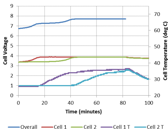
Figure IV - 228: Imbalance charging of a 2-cell series string at 200 mA. Cell 1 was initially at 100% SOC while Cell 2 was initially at 90% SOC.
