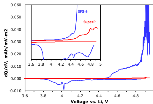
Figure IV - 192: dQ/dV plots from SFG-6 graphite- and SuperP- based electrodes. Inset is an expanded view along the Y-axis.
