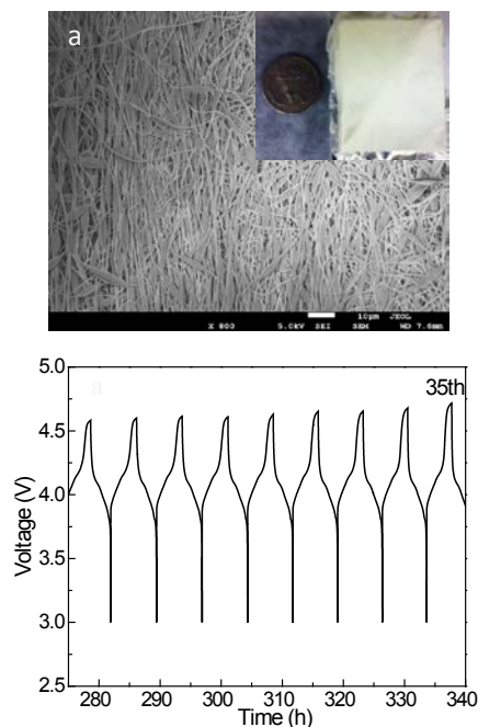
Figure IV - 237: a) SEM and digital (inset) images of the PFO and PEO composite separator and b) cycling voltage profiles of a protected \text{Li}_{1.05}\text{Mn}_{1.95}\text{O}_4 half-cell.
