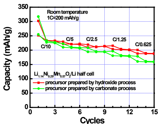
Figure IV - 119: Rate performance of cells based on cathodes made by hydroxide and carbonate process.
