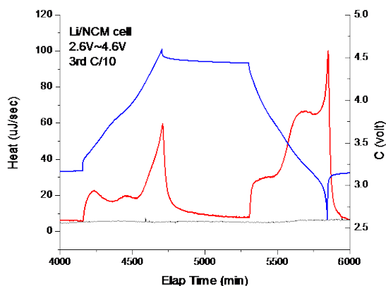
Figure IV - 14: Voltage and heat profile of HE5050 during charge and discharge.
