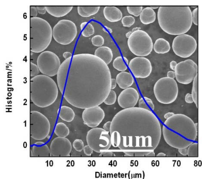
Figure IV - 44: Particle size distribution superimposed on SEM image of synthesized carbonate precursor.
