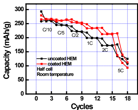
Figure IV - 114: Rate capability of cells based on coated and uncoated high energy cathode material.
