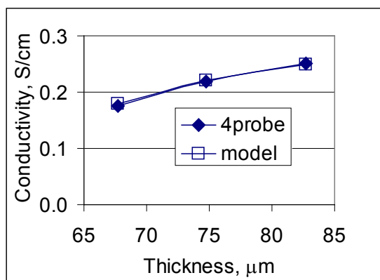
Figure IV - 56: Electrode conductivity of coating using polyester as substrate.
