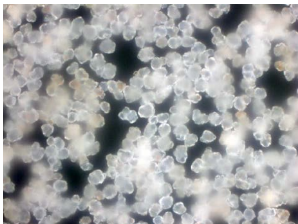
Figure IV - 246: Synthesized \text{MnCO}_3 precursors.
