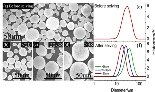
Figure IV - 45: Cathode morphologies and particle size distributions before and after sieving.
