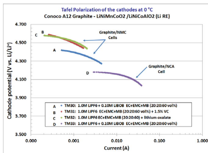
Figure IV - 173: Tafel polarization measurements at 0°C of three electrode cells consisting of Cononco A12 graphite/Toda HE 5050 LiNiCoMnO 2 or LiNiCoAlO 2 and containing various MB-based electrolytes.
