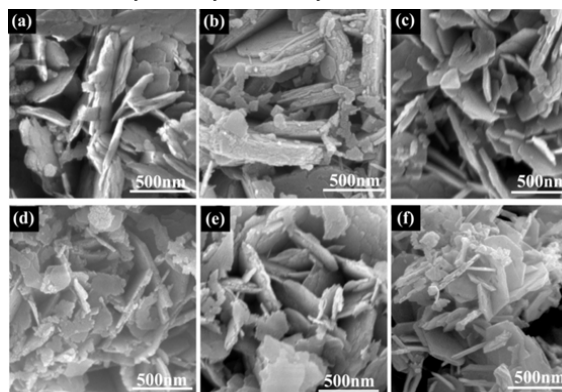
Figure IV - 37: SEM images of \text{Ni}_{0.25}\text{Mn}_{0.75}(\text{OH})_2 primary particles synthesized with different M_S/M_A in the base solutions (a) 0.667, (b) 1.5, (c) 1.8, (d) 2, (e) 2.5, (f) 4.
