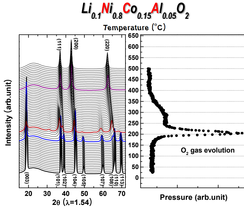
Figure IV - 212: TR-XRD of \text{Li}_{0.1}\text{Ni}_{0.8}\text{Co}_{0.15}\text{Al}_{0.05}\text{O}_2 (G2) with released oxygen MS during heating.
