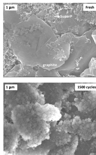
Figure IV - 195: SEM images of the fresh and aged (1500 cycles) negative electrodes.
