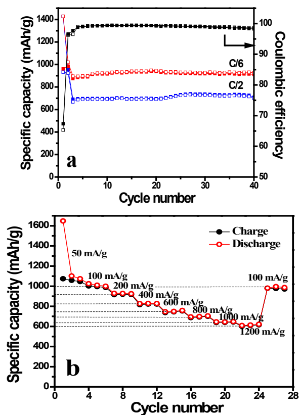
Figure IV - 98: Cycle performance and rate capability of 50wt.%SiO-50wt.% \text{Sn}_{30}\text{Fe}_{30}\text{C}_{40} prepared by spex-milling.
