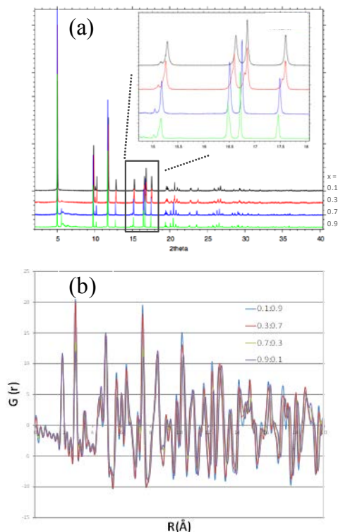
Figure IV - 142: a) XRD patterns and b) PDF spectra of x\text{Li}_2\text{MnO}_3 \cdot (1-x)\text{LiCoO}_2 , for x=0.1, 0.3, 0.7, and 0.9 annealed at 850^\circ\text{C} .
