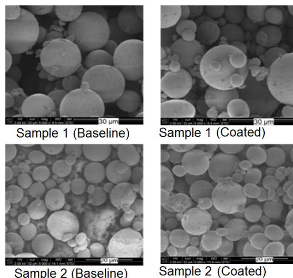
Figure IV - 70: SEM images of two different batches of Mn-rich cathode powders coated with alumina: the coatings are uniform and conformal over a range of baseline particle sizes.
