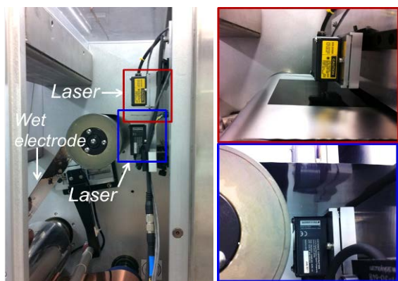
Figure IV - 82: In-line laser caliper set-up inside slot-die coater for wet thickness measurement.
