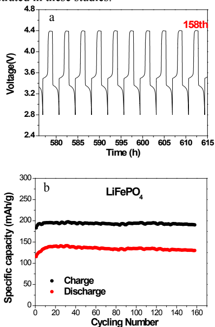
Figure IV - 233: (a) Voltage profile and b) cycling capacities of the polymer-protected cell with a \text{LiFePO}_4 cathode.
