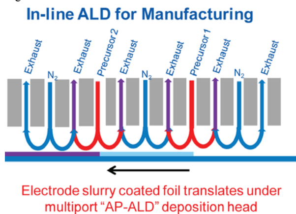
Figure IV - 61: A simplified schematic demonstrating the in-line spatial ALD concept.
