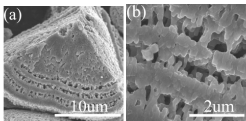
Figure IV - 47: SEM images of cathode materials with core-shell like features: (a) low magnification image and (b) higher magnification image of local area.
