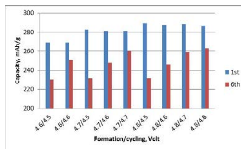
Figure IV - 9: Discharge capacity after 1st and 6th cycles under various testing conditions.
