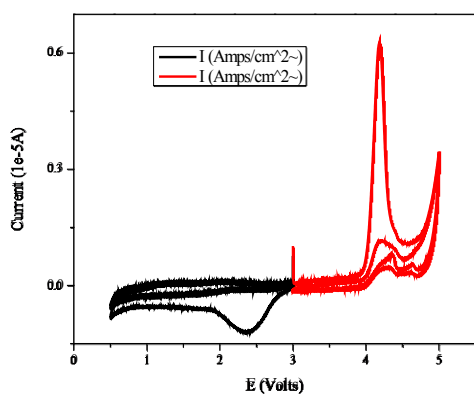
Figure IV - 149: Cyclic voltammogram profile 10mM TPP in Gen 2 electrolyte using Pt/Li/Li three electrode system. Scan rate is 100 mV/s.
