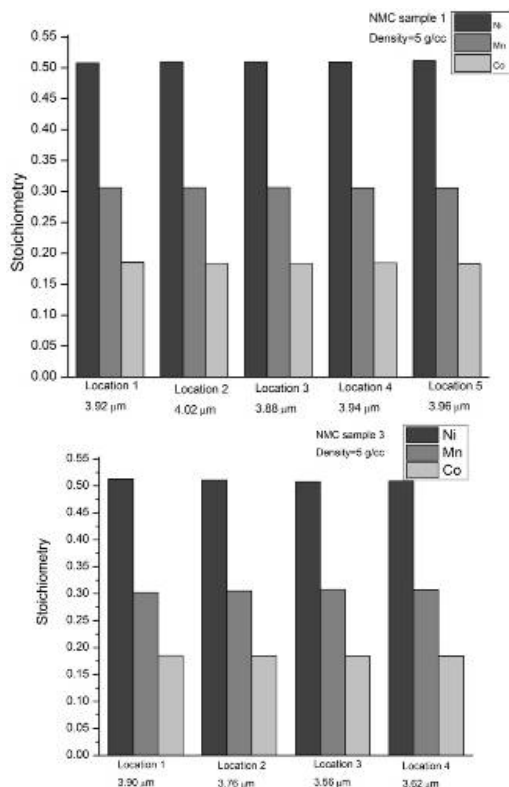
Figure IV - 89: Stoichiometry and thickness uniformity of Ni, Co, and Mn at different locations of a NCM 523 electrode coating.
