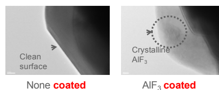
Figure IV - 111: TEM images of high energy cathode coated and uncoated with \text{AlF}_3 .
