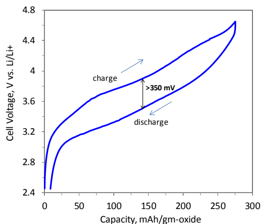
Figure IV - 190: Capacity-voltage plot, at a \sim C/35 rate and 30^\circ\text{C} , from a \text{Li}_{1.2}\text{Ni}_{0.15}\text{Mn}_{0.55}\text{Co}_{0.1}\text{O}_2/\text{Li} cell.
