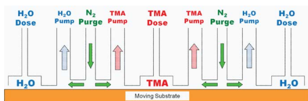
Figure IV - 62: A preliminary design from the George Group for demonstration of in-line AP-ALD.
