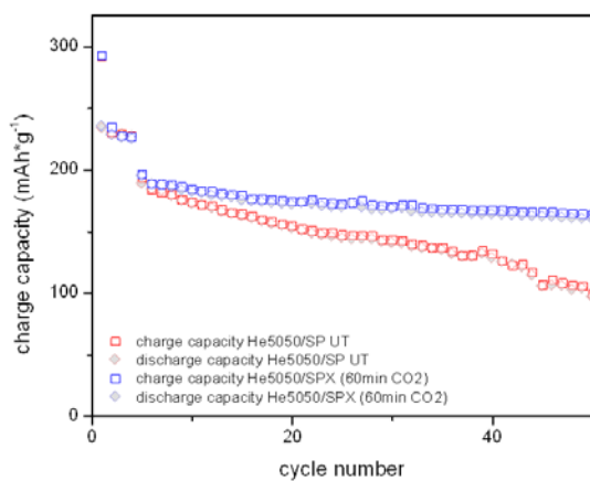
Figure IV - 201: Charge/Discharge capacity vs. cycle number of coin cells utilizing Toda He5050 and pristine (red) or heat treated (blue) carbon black.
