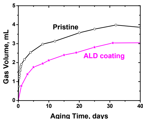
Figure IV - 109: Gas volume change for the LTO/LMO pouch cells with and without ALD coating on the LTO particle surface. The pouch cells have capacity of 100 mAh which is different from the ones used in the previous figure.
