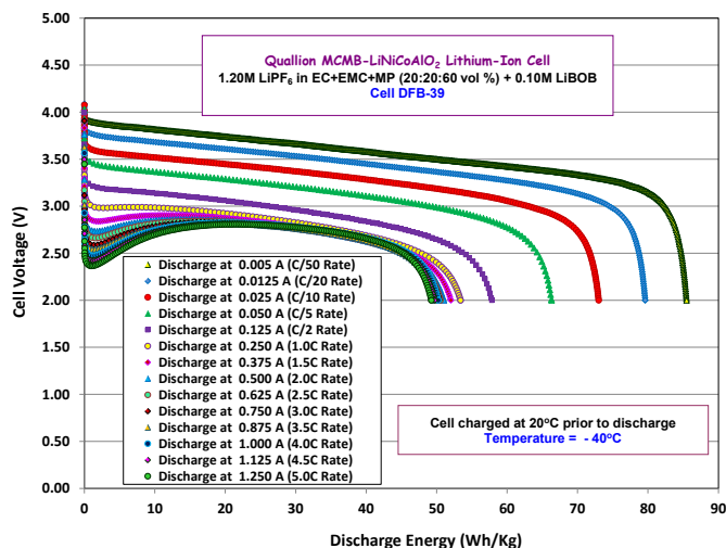
Figure IV - 169: Discharge performance of a 0.25Ah MCMB-LiNiCoAlO 2 cell containing a methyl propionate-based electrolyte with LiBOB at -40°C
