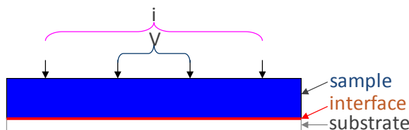
Figure IV - 55: Four point probe electrode conductivity geometry.
