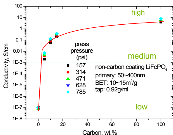
Figure IV - 53: Carbon Additive Effect on Conductivity of LiFePO 4 /Carbon Blend.
