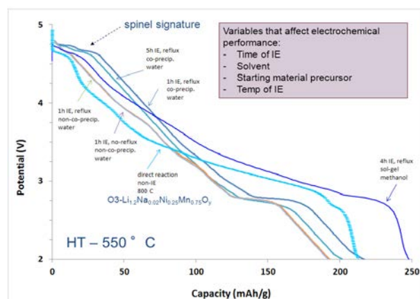
Figure IV - 133: Discharge voltage profiles of various IE cathode materials.
