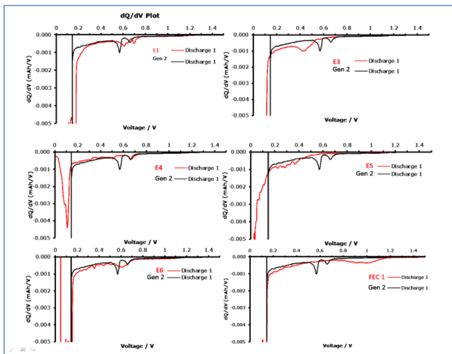
Figure IV - 157: dQ/dV plots of Gen2 electrolyte compared with fluorinated electrolytes.
