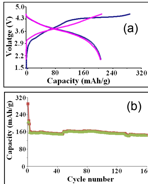
Figure IV - 101: a) First and second charge-discharge profiles, and b) cathode capacity vs. cycle number plot of a lithium-ion cell with a heat-treated (2800 °C) carbon sphere anode and a lithium manganese rich cathode between 4.6 and 2.0 V at a C/3 rate. (Note: the capacity refers to the cathode only).
