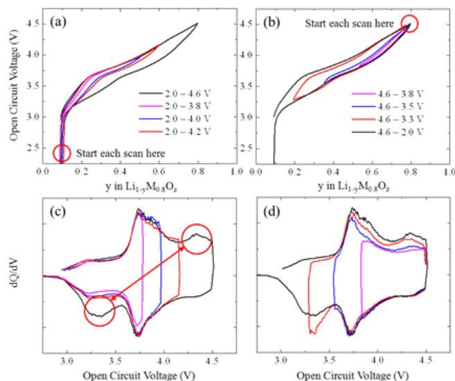
Figure IV - 15: Measured Open Circuit Voltages (a) and (b), and the corresponding dQ/dV (c) and (d) for \text{Li}_{1.25}\text{Ni}_{0.33}\text{Mg}_{0.02}\text{Mn}_{0.65}\text{O}_y .
