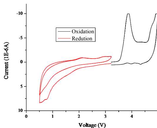
Figure IV - 150: Cyclic voltammogram profile 10mM PDP in Gen 2 electrolyte using Pt/Li/Li three electrode system. Scan rate is 100 mV/s.
