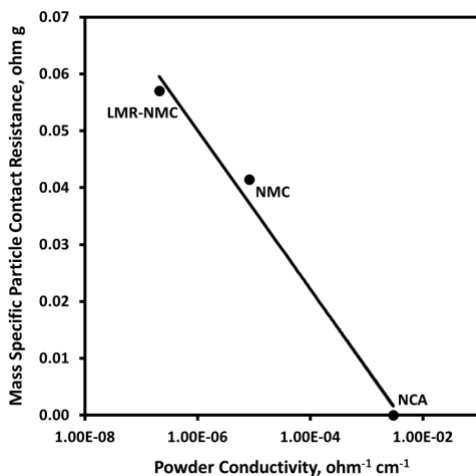
Figure IV - 182: Mass specific particle contact resistance determined by electrochemical model for NCA, NMC333 and LMR-NMC electrodes compared to the dry powder's particle conductivity.
