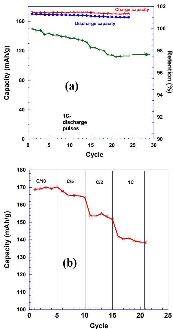
Figure IV - 77: Initial performance of NCM 523 cathodes; a) 25 cycles discharged at C/5 and b) rate performance.
