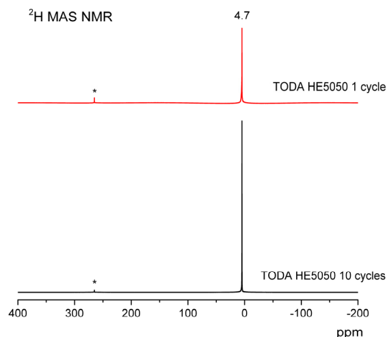
Figure IV - 29: ^2\text{H} MAS NMR of cycled TODA HE5050 material at a spinning speed of 20 kHz at 11.7 Tesla magnetic field. * indicates spinning side bands.
