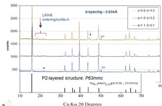
Figure IV - 125: X-ray powder diffraction patterns of \text{Na}_a\text{Li}_b\text{Ni}_{0.25}\text{Mn}_{0.75}\text{O}_y precursor. The asterisk indicates a superlattice peak, and the additional peaks in the top pattern indicate the formation of \text{LiMn}_6 sites within the \text{Na}(\text{Li},\text{M})\text{O}_2 structure.
