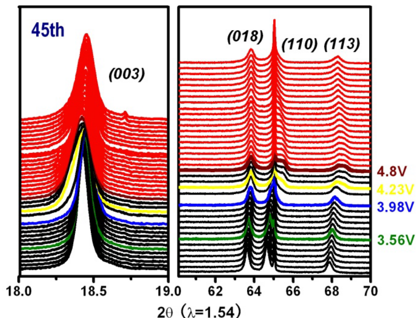
Figure IV - 215: Crystal structure changes of Li-rich cathode material \text{Li}_{1.2}\text{Ni}_{0.15}\text{Co}_{0.1}\text{Mn}_{0.55}\text{O}_2 during 46th charge-discharge cycle.
