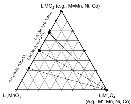
Figure IV - 138: A compositional phase diagram of a 'layered-layered-spinel' system with \text{Li}_2\text{MnO}_3 \cdot (1-x)\text{LiMO}_2 ('layered-layered') and \text{LiM}'_2\text{O}_4 (spinel) components.
