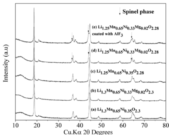
Figure IV - 32: XRD patterns of various materials derived from the ‘layered-layered-spinel’ \text{Li}_x\text{Mn}_{0.65}\text{Ni}_{0.35}\text{O}_y system.
