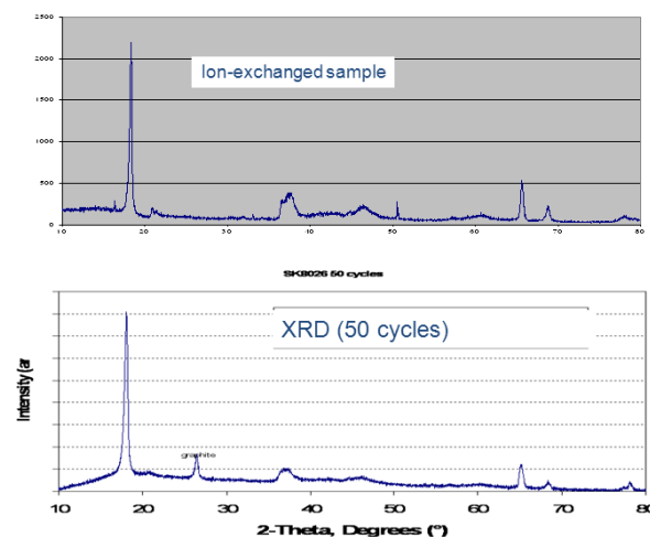
Figure IV - 135: XRD pattern of IE material electrode laminate before (top) and after (bottom) 50 cycles.
