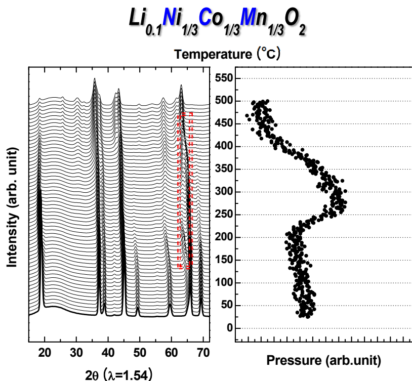
Figure IV - 211: TR-XRD of \text{Li}_{0.1}\text{Ni}_{1/3}\text{Co}_{1/3}\text{Mn}_{1/3}\text{O}_2 (G3) with released oxygen MS during heating.
