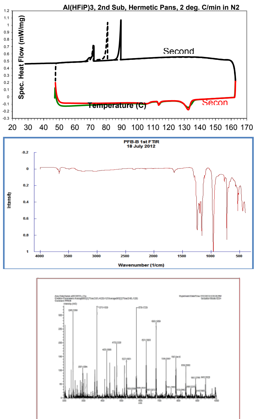
Figure IV - 161: DSC traces of Al(HFiP) 3 (a); FTIR (b) and MS (c) of B(PFB) 3 .
