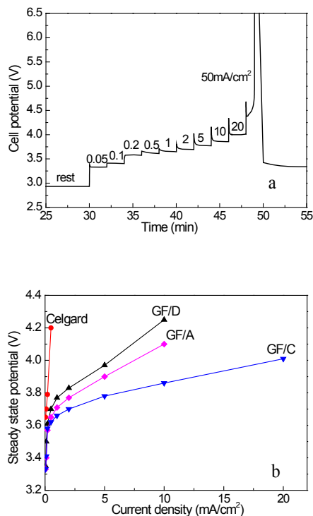
Figure IV - 232: (a) Voltage profile of the P3BT-GF/C composite at the indicated current densities and (b) comparison of the sustainable current densities achieved by the P3BT composites on various substrates.
