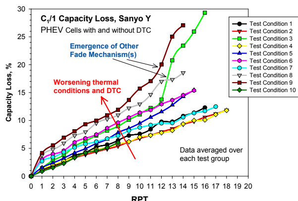
Figure IV - 203: C/1 Capacity Loss, Sanyo Y.
