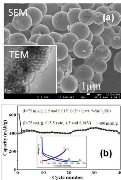
Figure IV - 103: (a) SEM and TEM (inset) images of SnO 2 /Sb-coated carbon spheres, (b) First and second discharge-charge-profiles (inset) and capacity vs. cycle number plot of a lithium half-cell with a SnO 2 /Sb-carbon sphere electrode cycled between 1.5 and 0.01 V at a C/5.5 rate.
