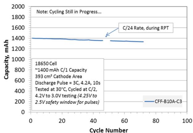
Figure IV - 269: Cycling data of cell from first 18650 cell build in Cell Fabrication Facility, ConocoPhillips A12 Graphite vs. Toda NCM523 cathode.
