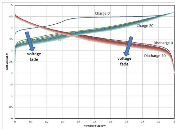
Figure IV - 2: LMR-NMC voltage profiles during charge and discharge versus normalized capacity. Voltage fade is clearly evident.
