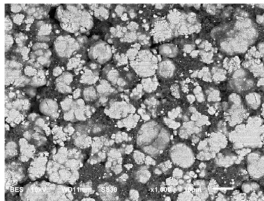
Figure IV - 240: Fractured cathode particles from calendaring from lot#2012-02-22.
