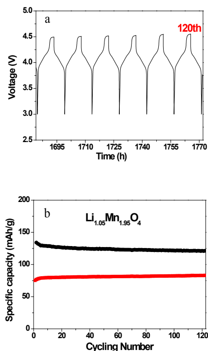
Figure IV - 234: (a) Voltage profile and b) cycling capacities of the polymer-protected cell with a spinel \text{Li}_{1.05}\text{Mn}_{1.95}\text{O}_4 cathode.
