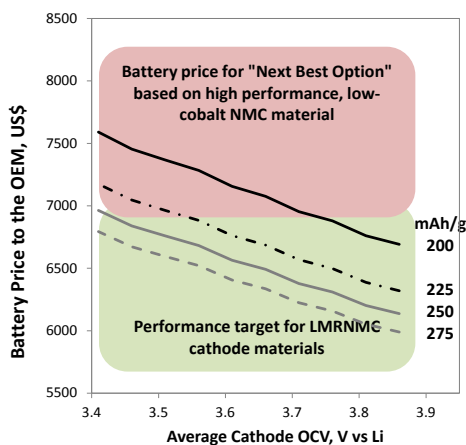
Figure IV - 8: Battery Price to OEM for an advanced Li-ion anode with LMR-NMC cathodes with varying capacities as a function of cathode OCV for (left) an EV150 compared against the next best Li-ion cathode option and (right) a PHEV40 compared against DOE goals.
