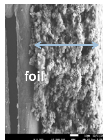
Figure IV - 117: SEM images of high energy electrode made by carbonate process.
