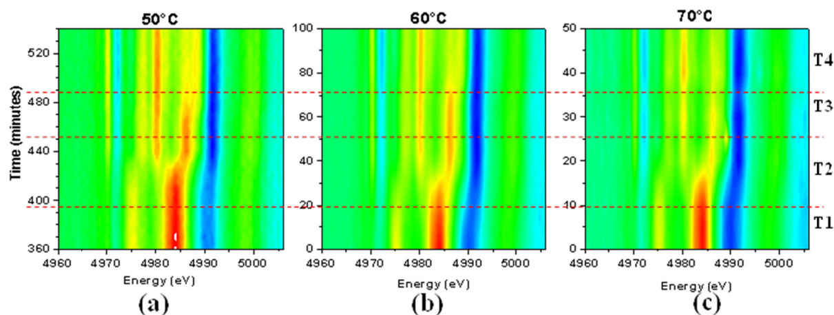
Figure IV - 107: Contour plots of the derivatives of the normalized energy for three temperature settings, (a) 50°C, (b) 60°C and (c) 70°C.
