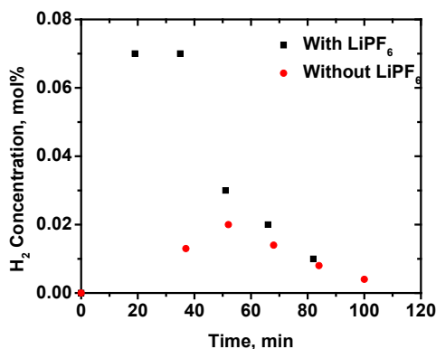
Figure IV - 105: Hydrogen concentration change with reaction time measured by in situ GC. The supporting Ar flow rate is 14 mL/min. Black squares represent condition with LiPF 6 in the electrolyte; red circles, no LiPF 6 in the electrolyte.
