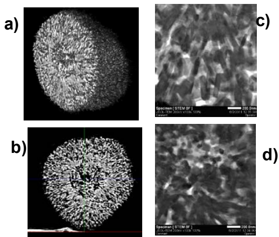
Figure IV - 122: (a) 3D presentation of nickel distribution in a single lithiated full concentration gradient lithium transition metal oxide particle; (b) 2D distribution of nickel on a plane going through the center of the particle; (c) transmission electron microscopy image of local structural feature near the edge of the particle; and (d) transmission electron microscopy image of local structural feature at the center of the particle.
