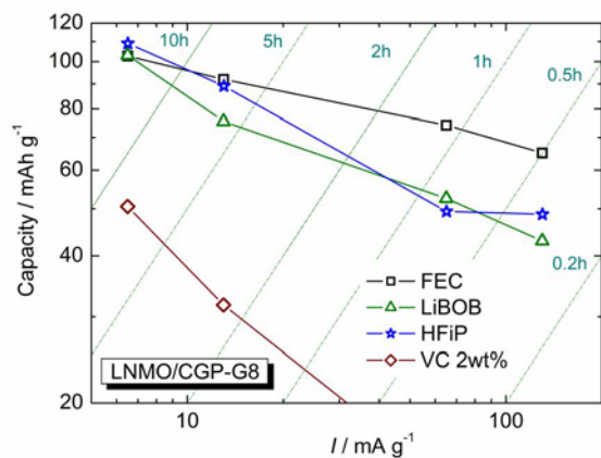
Figure IV - 41: The effect of electrolyte additives on full-cell rate performance.
