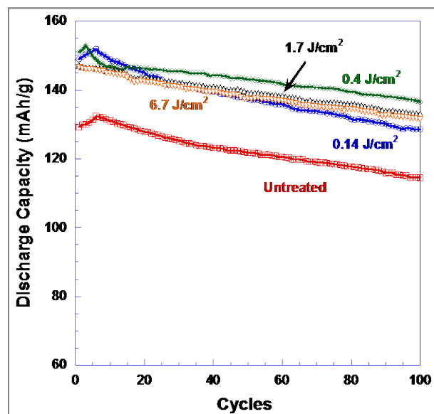
Figure IV - 75: Cycling of LiFePO 4 cathodes at 0.5C/0.5C (0.34 mA/cm 2 ) confirming 0.4 J/cm 2 as the best corona treatment energy density for long term performance.
