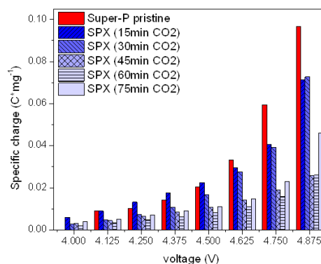
Figure IV - 200: Specific charge of potentiostatic step investigation of pristine and heat-treated Super-P samples.
