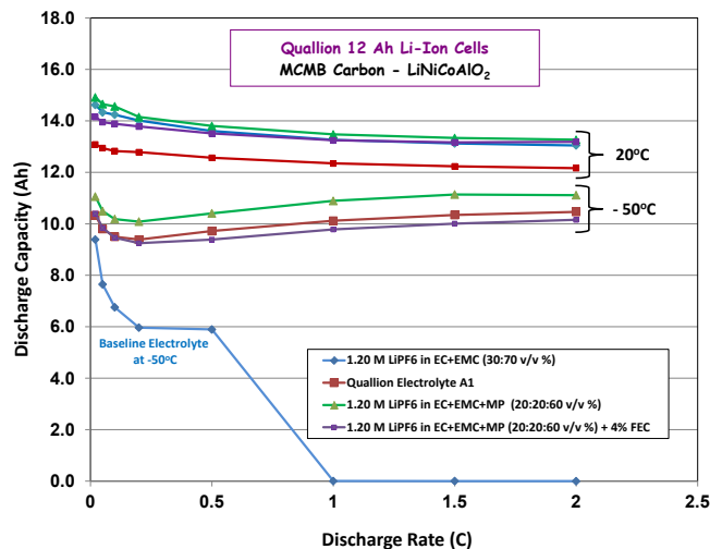
Figure IV - 166: Discharge rate capability of 12 Ah MCMB-LiNiCoAlO 2 cells (Quallion, LCC) containing various electrolytes at +20^{\circ}\text{C} and -50^{\circ}\text{C} (See first figure, A).
