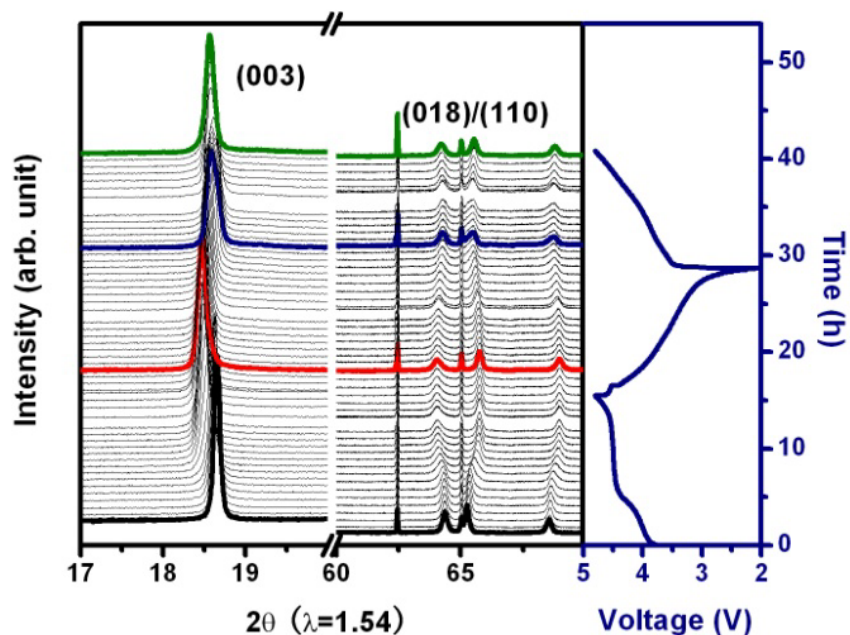
Figure IV - 214: Crystal structure changes of Li-rich cathode material \text{Li}_{1.2}\text{Ni}_{0.15}\text{Co}_{0.1}\text{Mn}_{0.55}\text{O}_2 during first one and half charge-discharge cycle.
