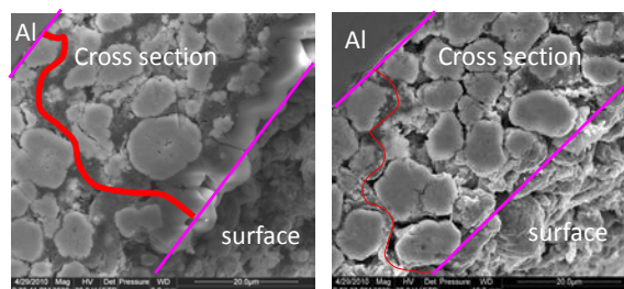
Figure IV - 54: SEM images of electrode with no carbon coating (left) and with 3% carbon coating on the particles.
