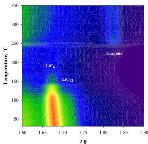
Figure IV - 218: Contour plot of in situ HEXRD data during thermal decomposition of lithiated graphite.
