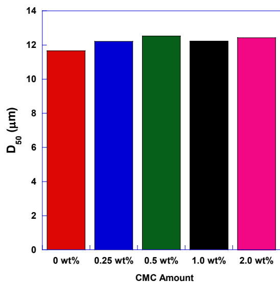
Figure IV - 81: Agglomerate size of aqueous NCM523 suspension with various CMC concentrations.
