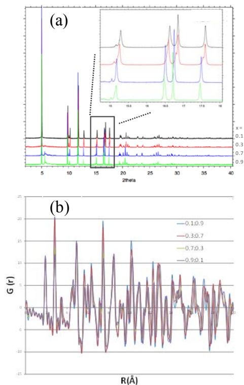
Figure IV - 34: a) XRD patterns and b) PDF spectra of x\text{Li}_2\text{MnO}_3 \cdot (1-x)\text{LiCoO}_2 , for x=0.1, 0.3, 0.7, and 0.9 annealed at 850^\circ\text{C} .
