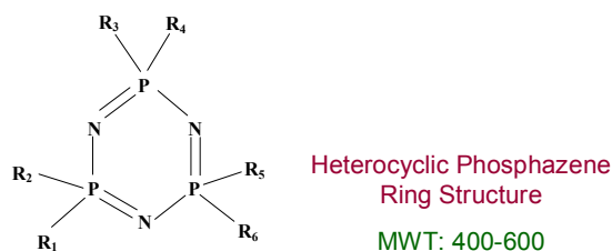
Figure IV - 174: General heterocyclic phosphazene structure.
