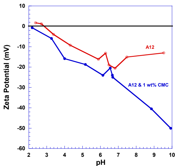
Figure IV - 78: Zeta potential of A12 graphite with and without CMC; the addition of 1 wt% CMC resulted in a more negative charge on the A12 surface.
