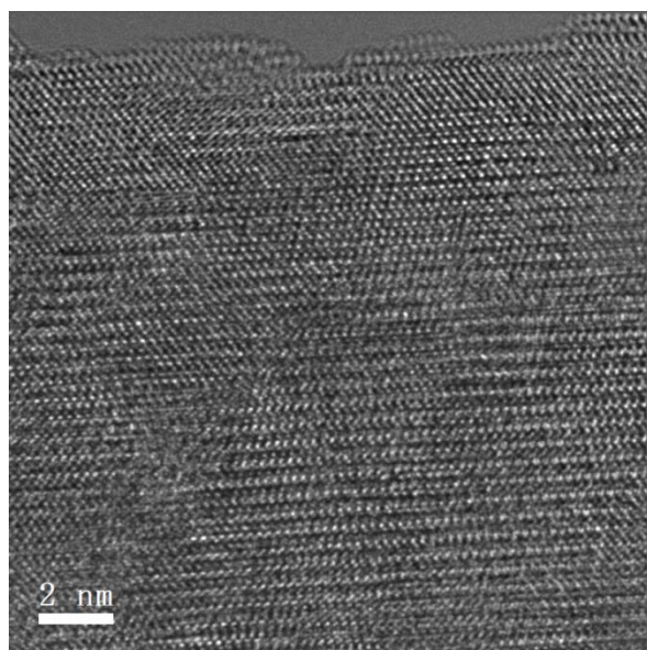
Figure IV - 23: High resolution image of \text{Li}_{1.2}\text{Ni}_{0.15}\text{Mn}_{0.55}\text{CO}_{0.1}\text{O}_2 after cycling (1500x) showing the uniform transformation to spinel-like phase.
