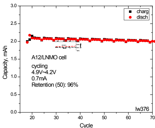
Figure IV - 261: Cycle performance of graphite/LNMO cell.
