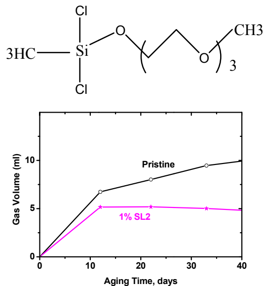
Figure IV - 108: Gas evolution in pouch cells LTO/LMO with /without 1% SL2 as the additive in the electrolyte of 1.2M \text{LiPF}_6 in EC/EMC in 3:7 in weight.
