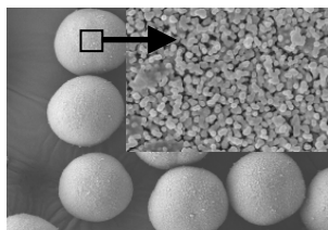
Figure IV - 110: SEM images of \text{Li}_{1.2}\text{Ni}_{0.3}\text{Mn}_{0.6}\text{O}_{2.1} showing spherical secondary particle and dense nano-primary particles.
