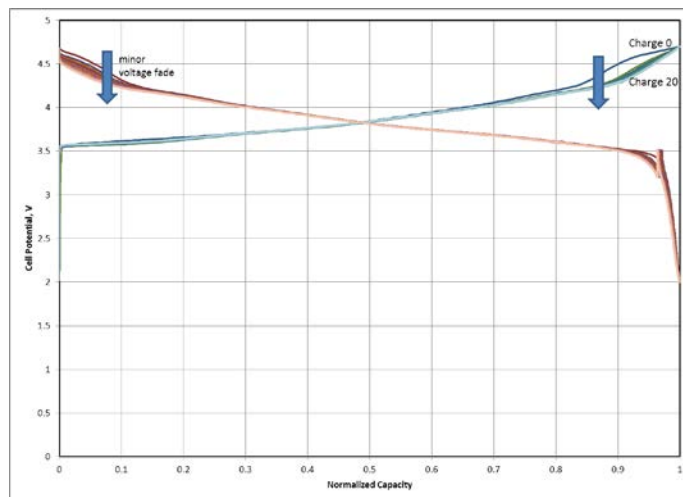
Figure IV - 4: Capacity-normalized voltage profiles for NCA. Some minor voltage fade is apparent at the end of charge and beginning of discharge.
