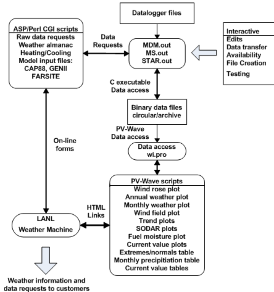
Figure 3. Main software components that control the flow of raw data from raw data files to the formatted products.
