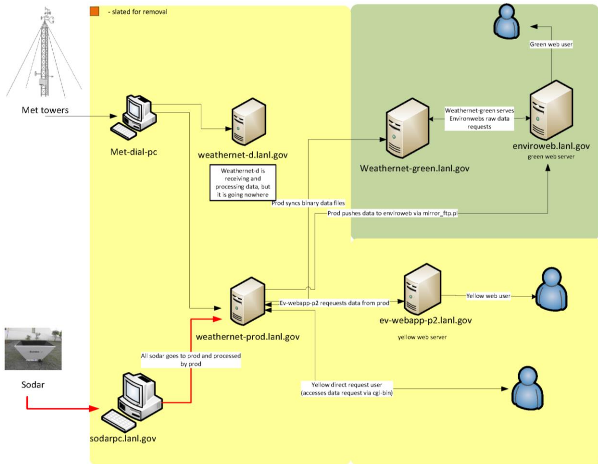
Figure 2. Main hardware components used in acquiring and processing meteorological data.
