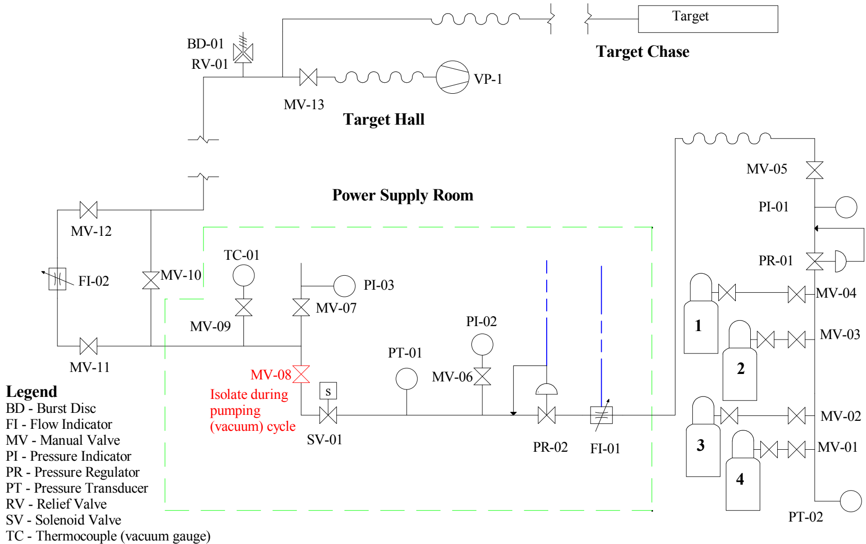
Figure A-1: Target helium system schematic.
