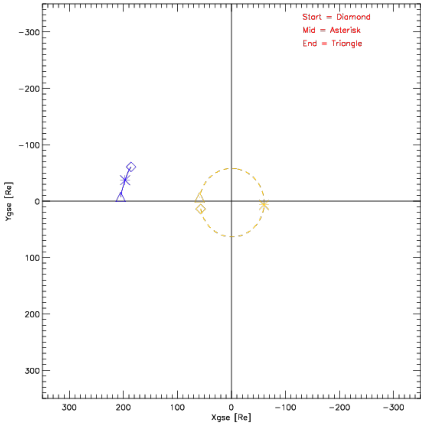
Wind and Lunar Orbits from 1995-02-01 to 1995-02-28
