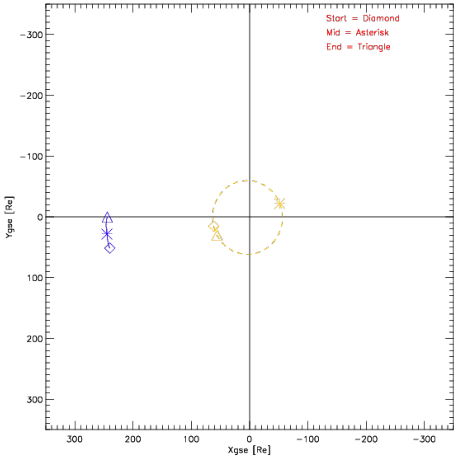
Wind and Lunar Orbits from 1995-05-01 to 1995-05-31
