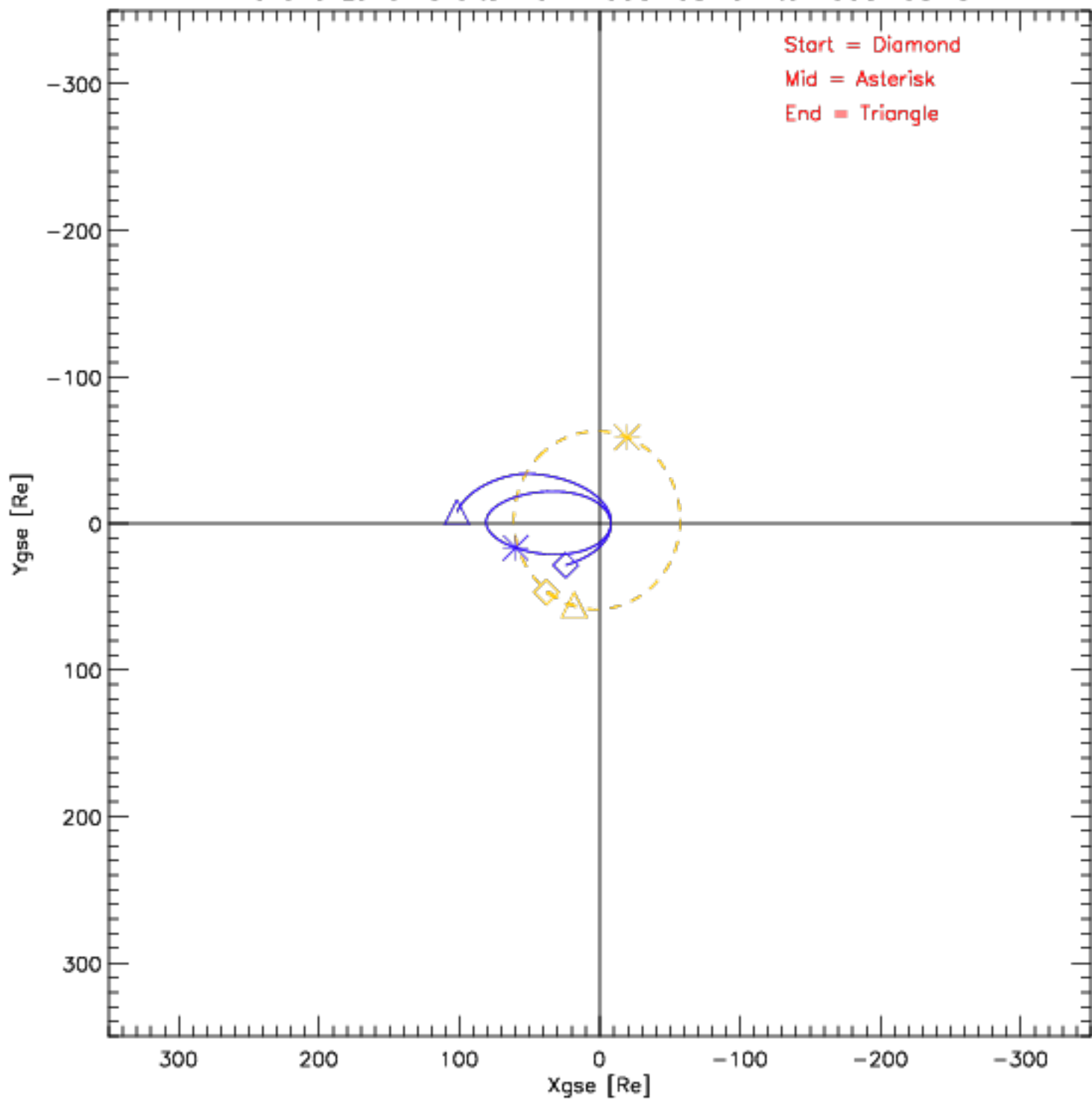
Wind and Lunar Orbits from 1995-08-01 to 1995-08-31
