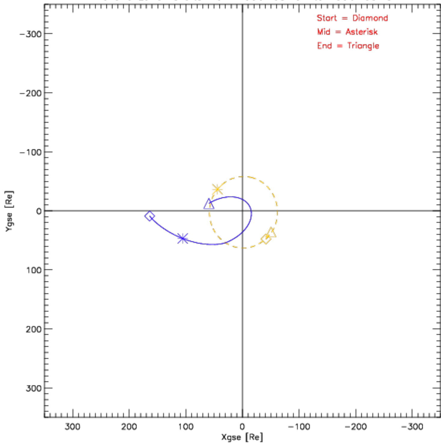
Wind and Lunar Orbits from 1996-03-01 to 1996-03-31
