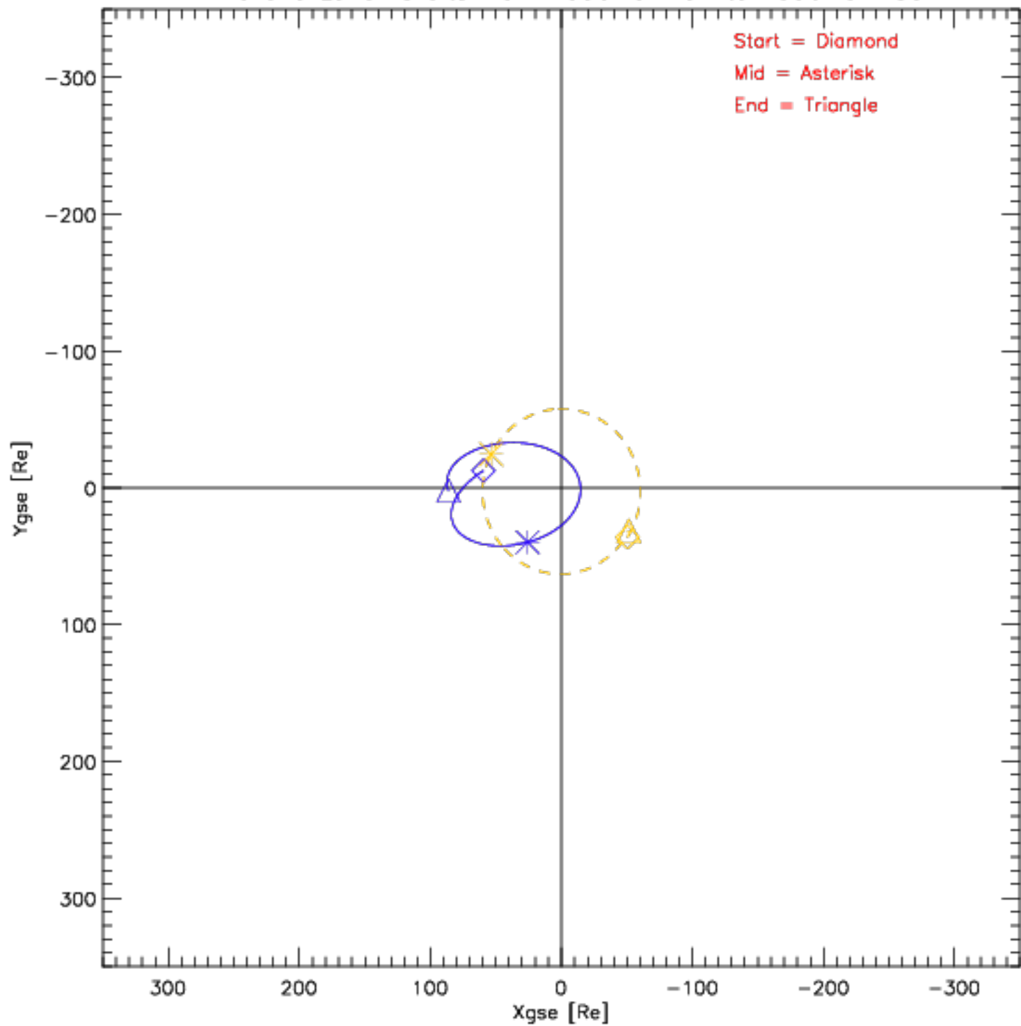
Wind and Lunar Orbits from 1996-04-01 to 1996-04-30
