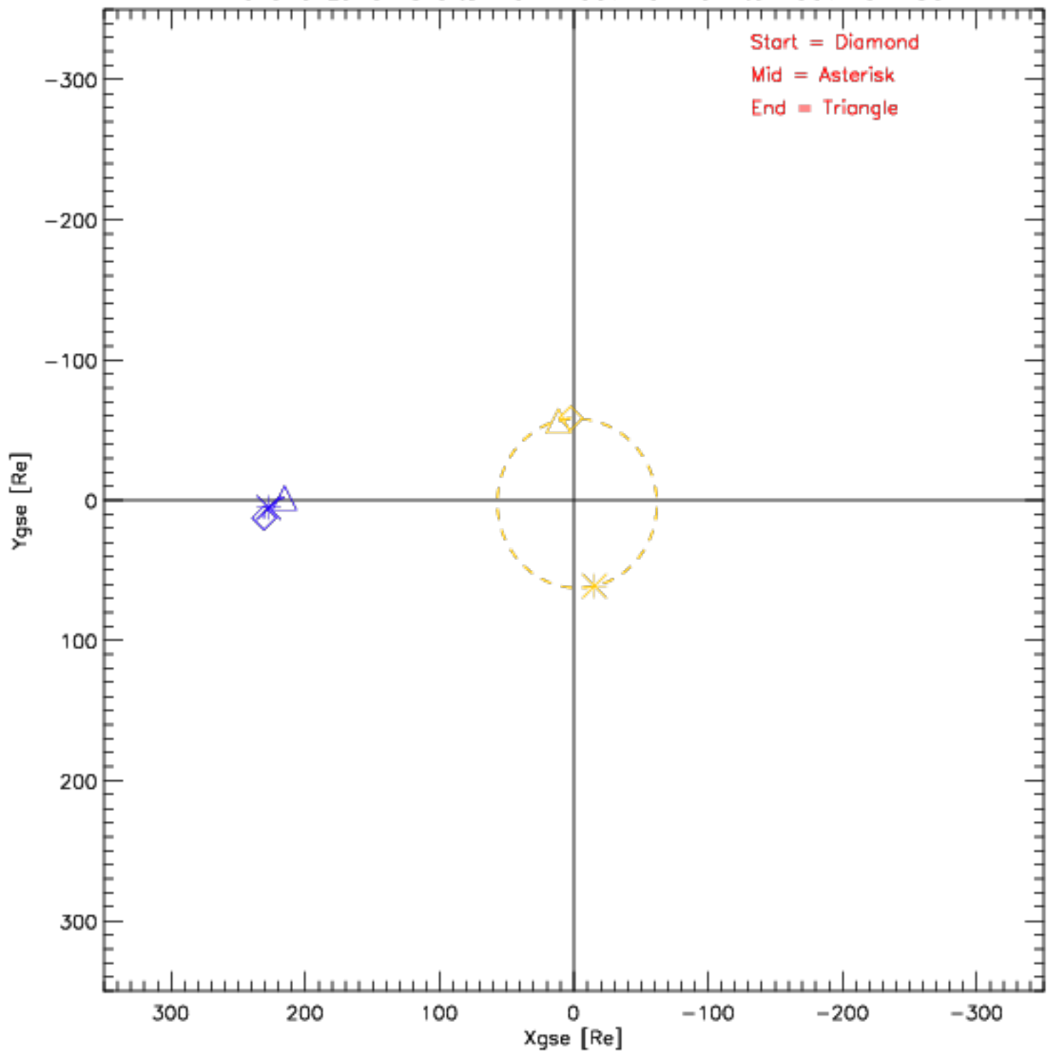
Wind and Lunar Orbits from 1997-04-01 to 1997-04-30
