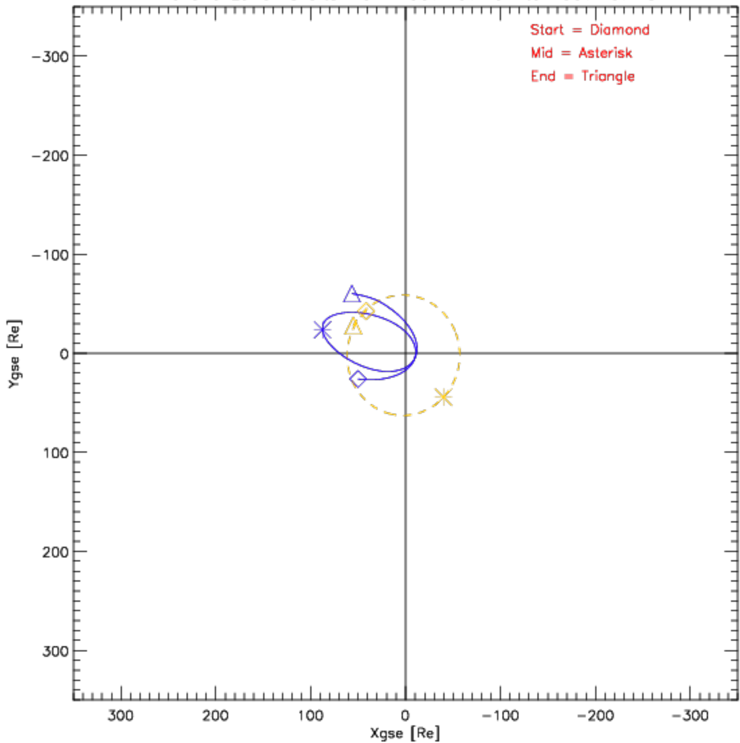
Wind and Lunar Orbits from 1997-07-01 to 1997-07-31
