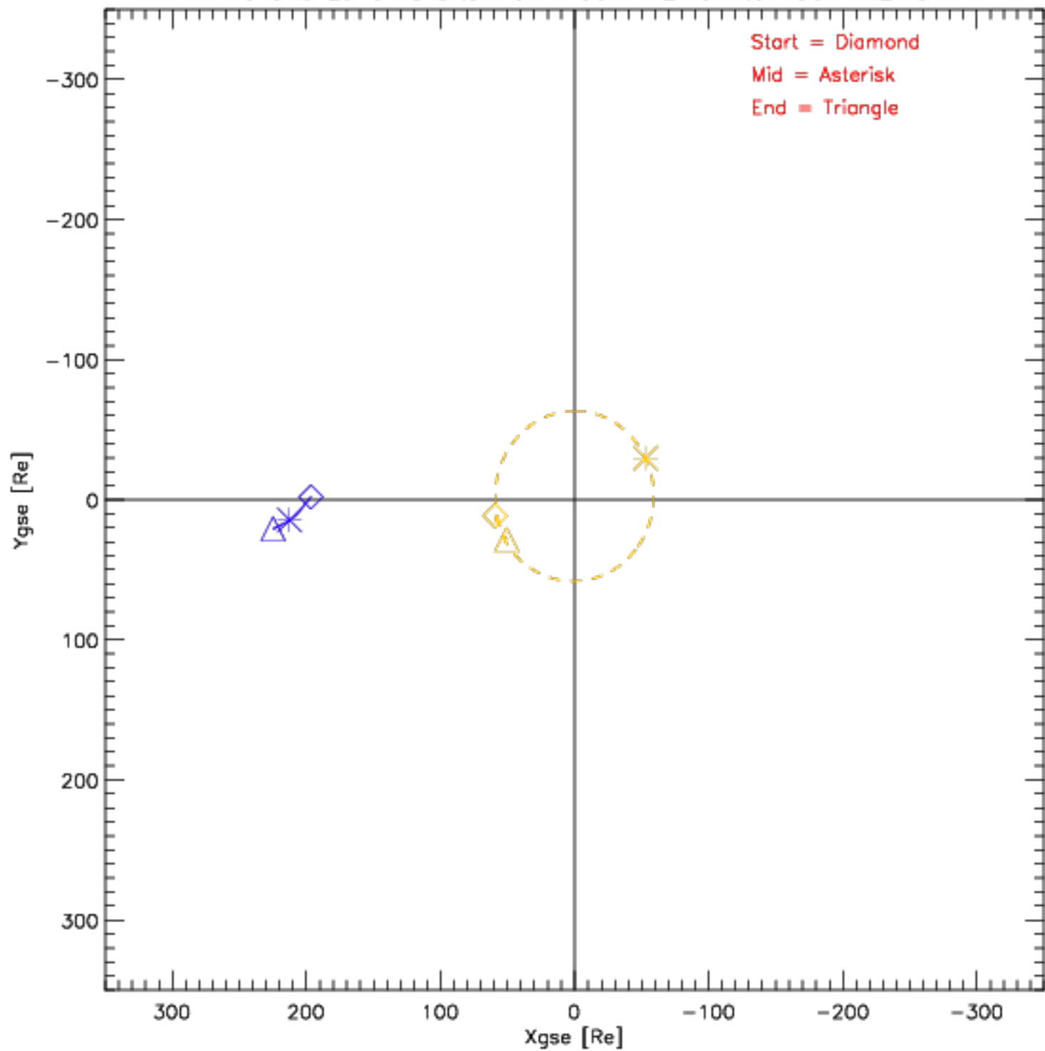
Wind and Lunar Orbits from 1997-12-01 to 1997-12-31
