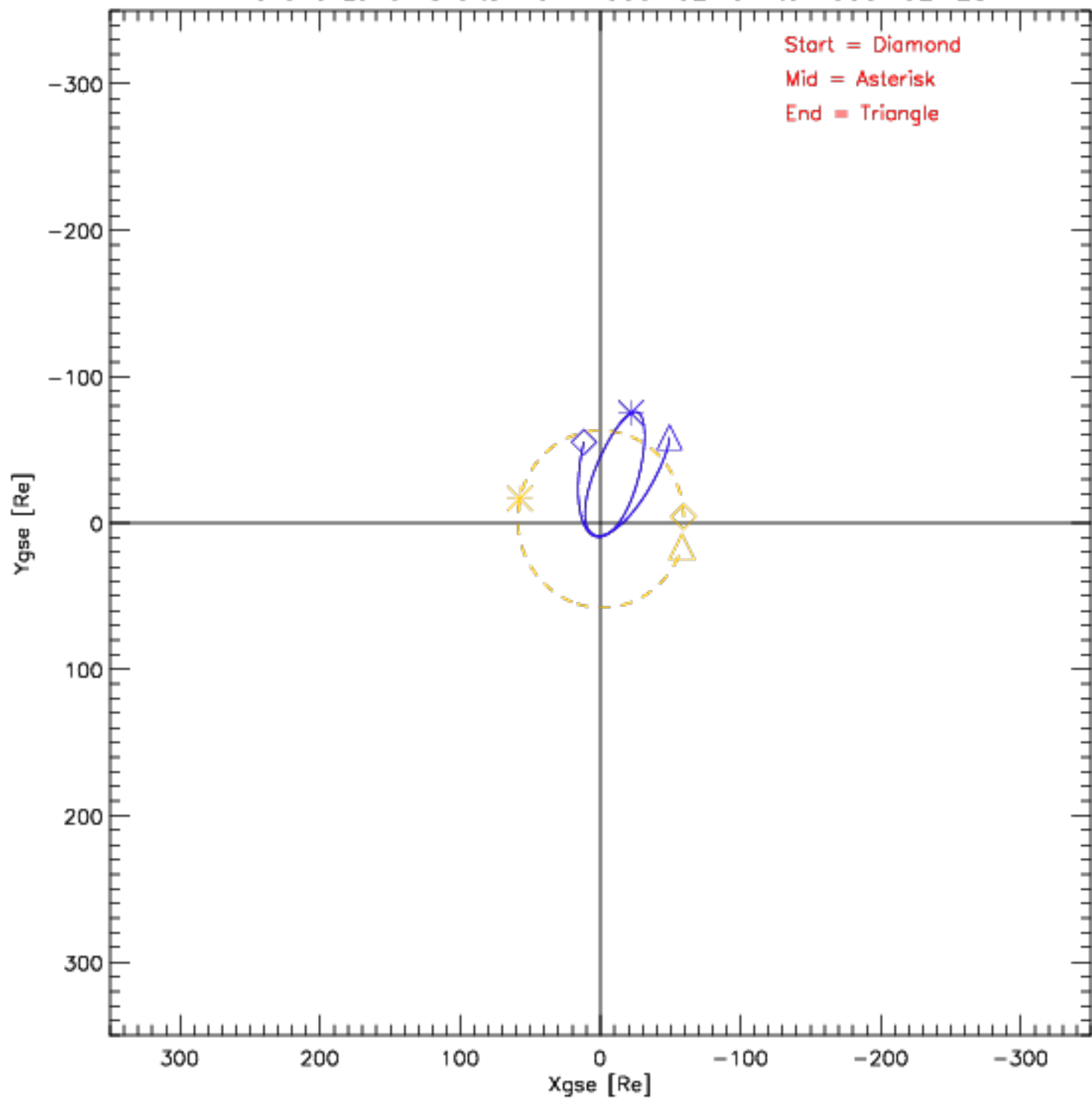
Wind and Lunar Orbits from 1999-02-01 to 1999-02-28
