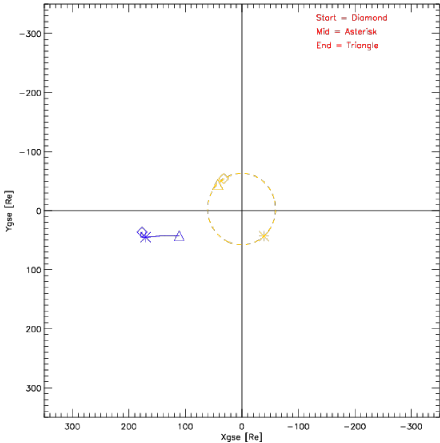
Wind and Lunar Orbits from 2000-03-01 to 2000-03-31
