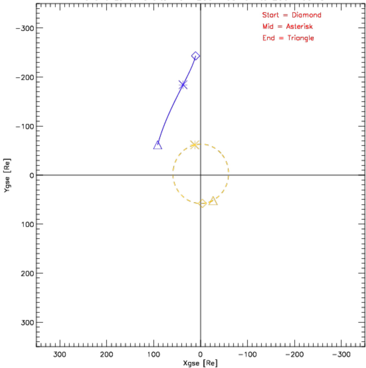
Wind and Lunar Orbits from 2001-05-01 to 2001-05-31
