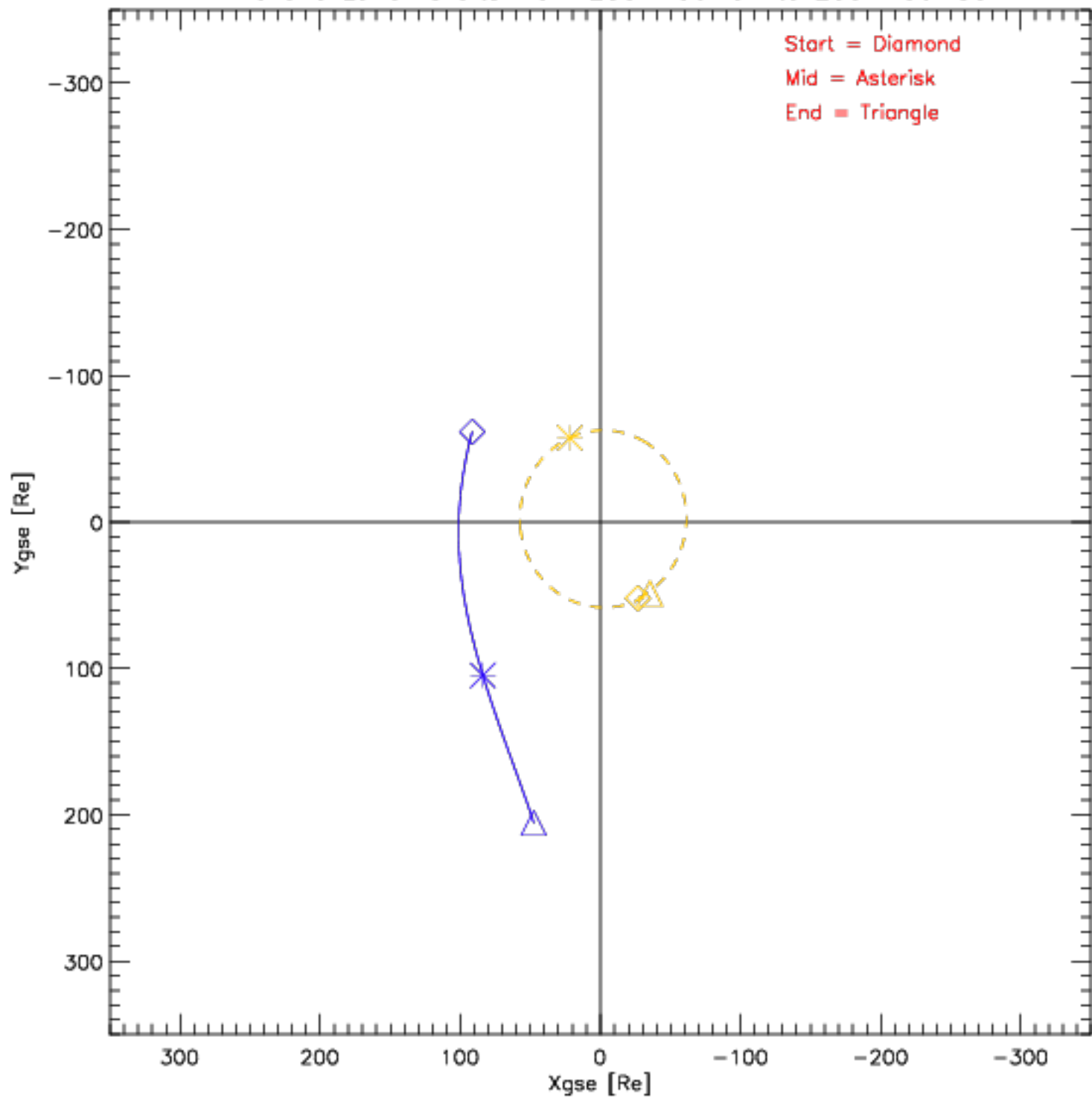
Wind and Lunar Orbits from 2001-06-01 to 2001-06-30
