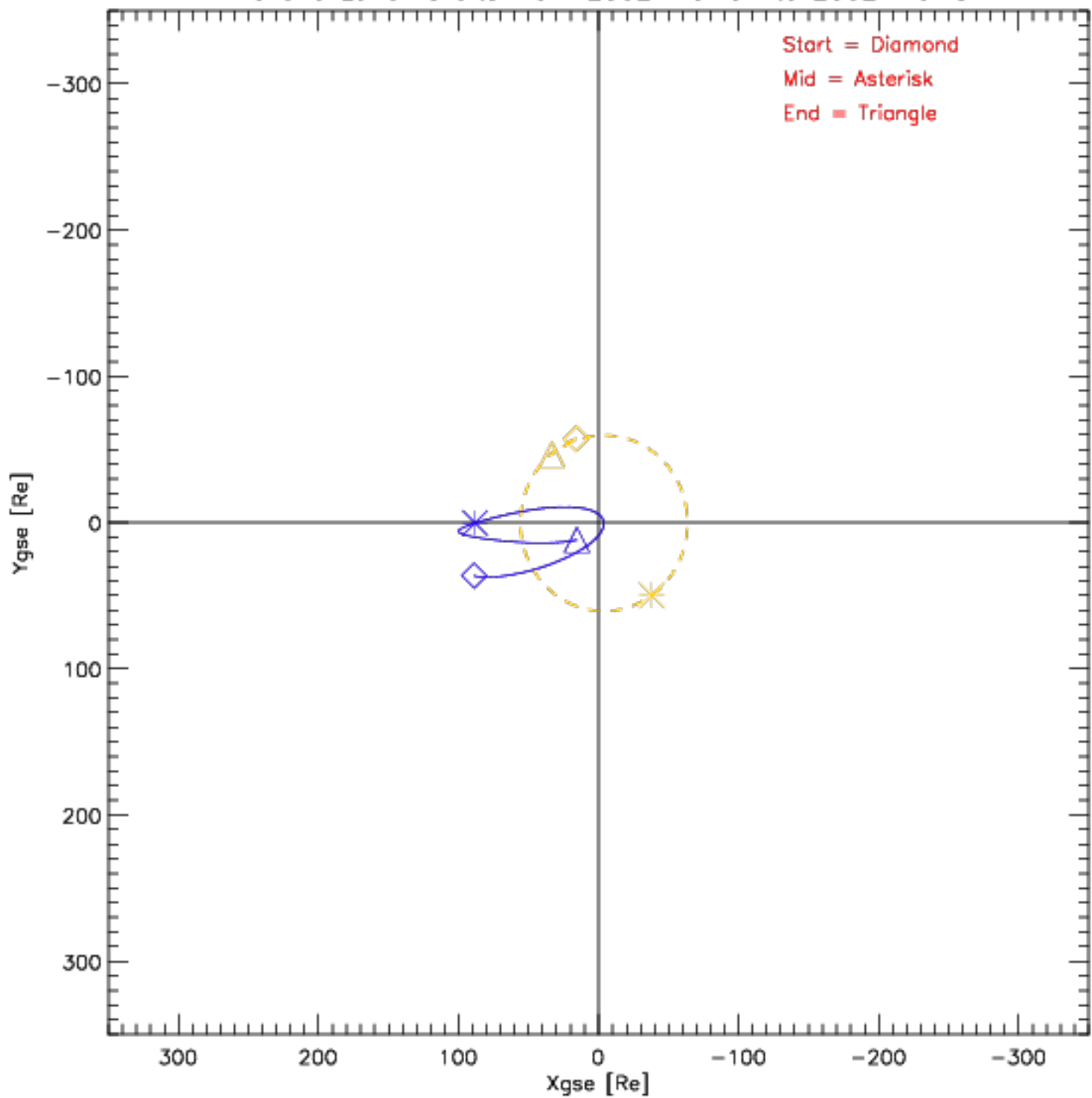
Wind and Lunar Orbits from 2002-10-01 to 2002-10-31
