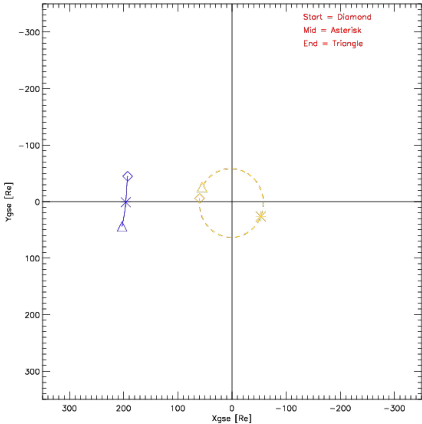
Wind and Lunar Orbits from 2003-02-01 to 2003-02-28
