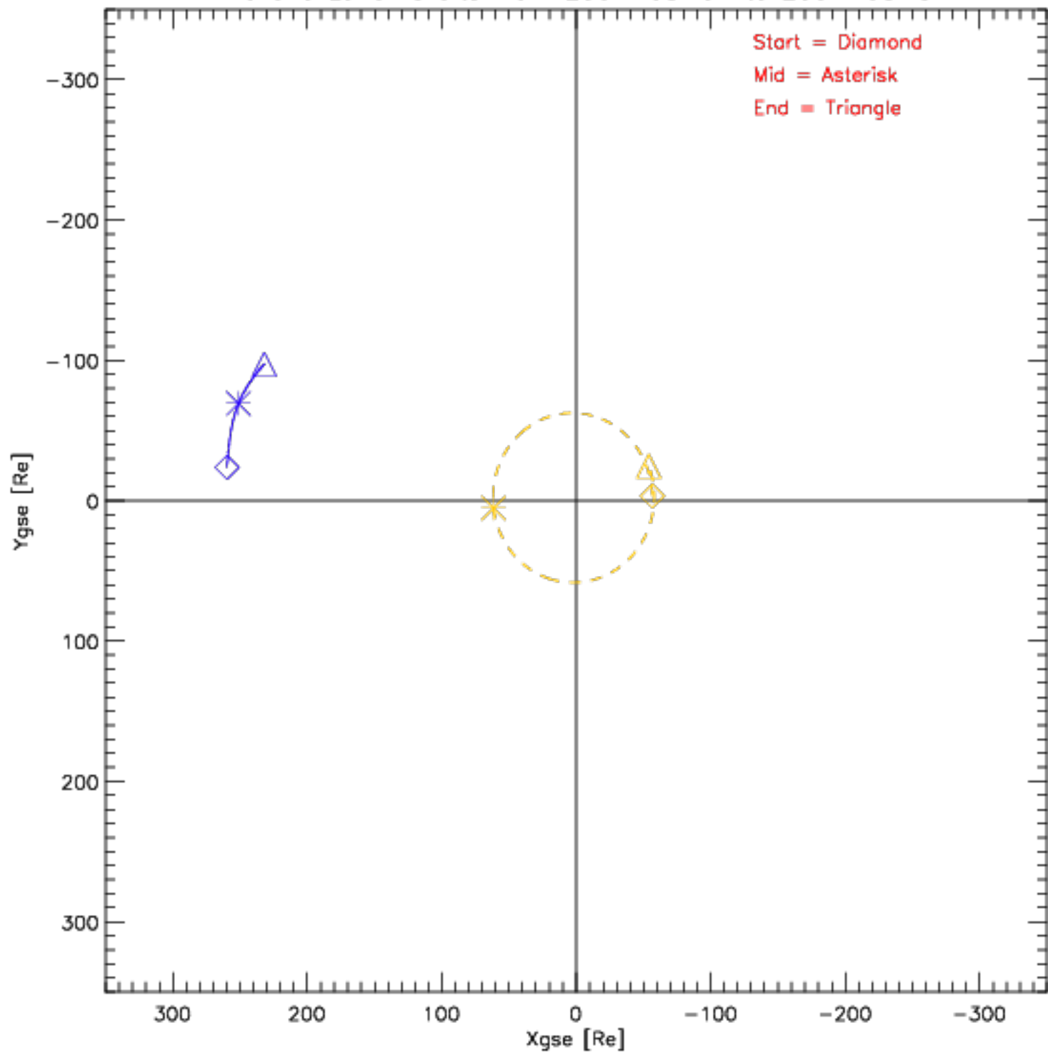
Wind and Lunar Orbits from 2004-08-01 to 2004-08-31
