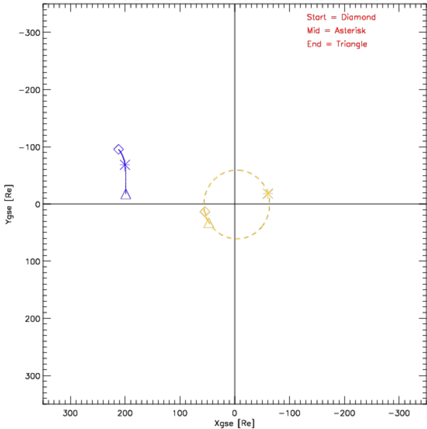
Wind and Lunar Orbits from 2006-03-01 to 2006-03-31
