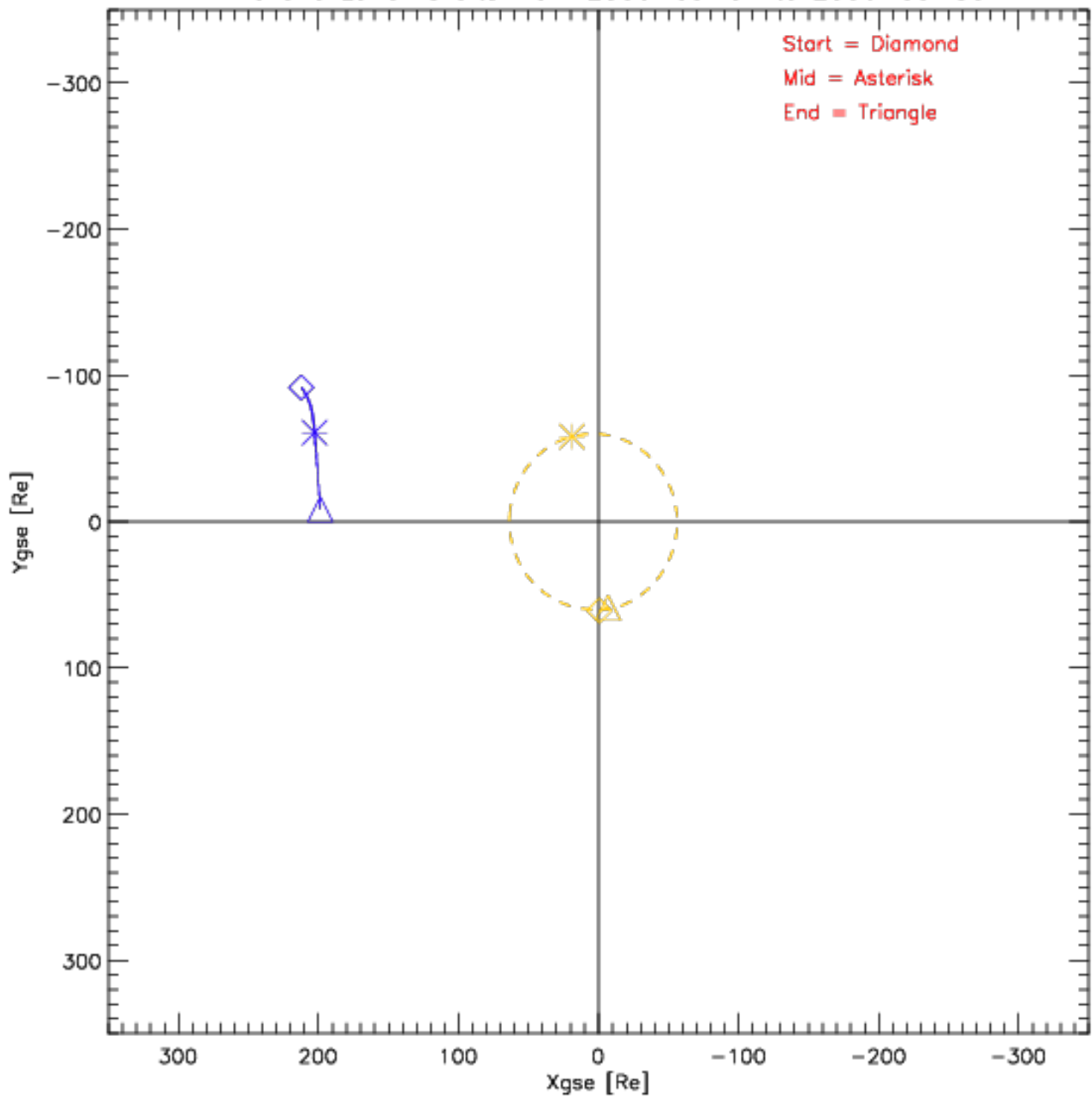
Wind and Lunar Orbits from 2006-09-01 to 2006-09-30
