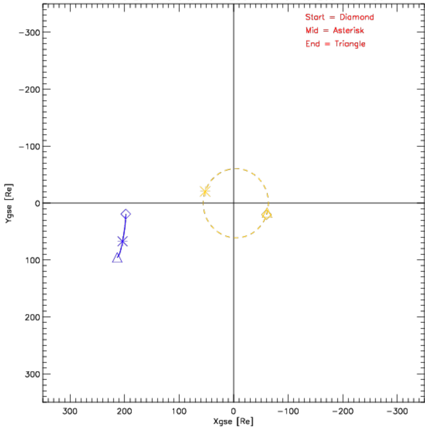
Wind and Lunar Orbits from 2007-04-01 to 2007-04-30
