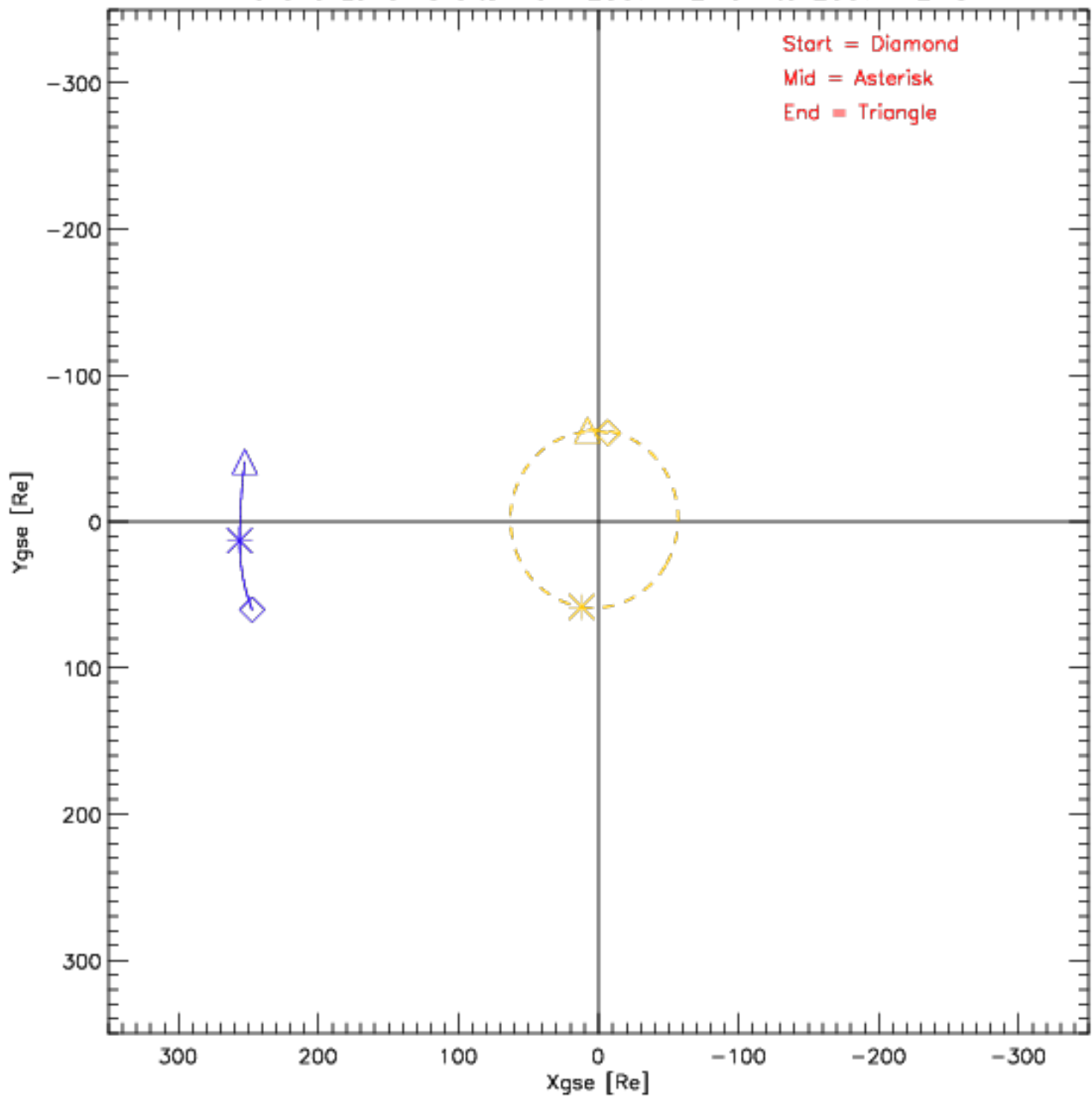
Wind and Lunar Orbits from 2007-12-01 to 2007-12-31
