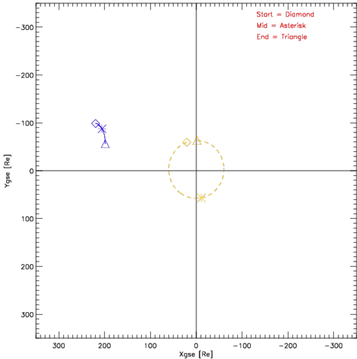
Wind and Lunar Orbits from 2008-02-01 to 2008-02-28
