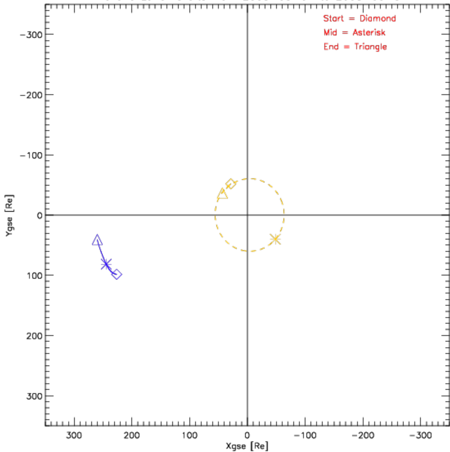
Wind and Lunar Orbits from 2008-05-01 to 2008-05-31
