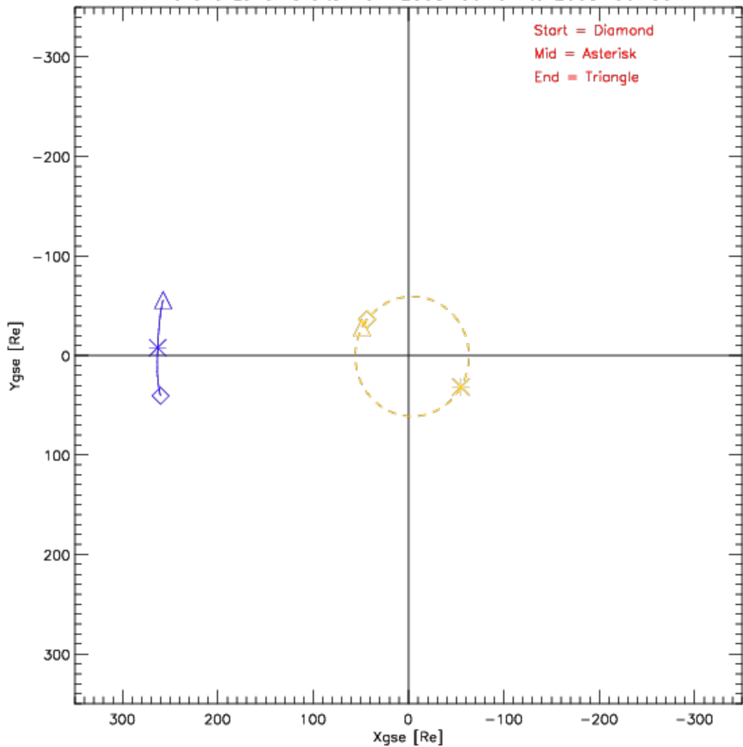
Wind and Lunar Orbits from 2008-06-01 to 2008-06-30
