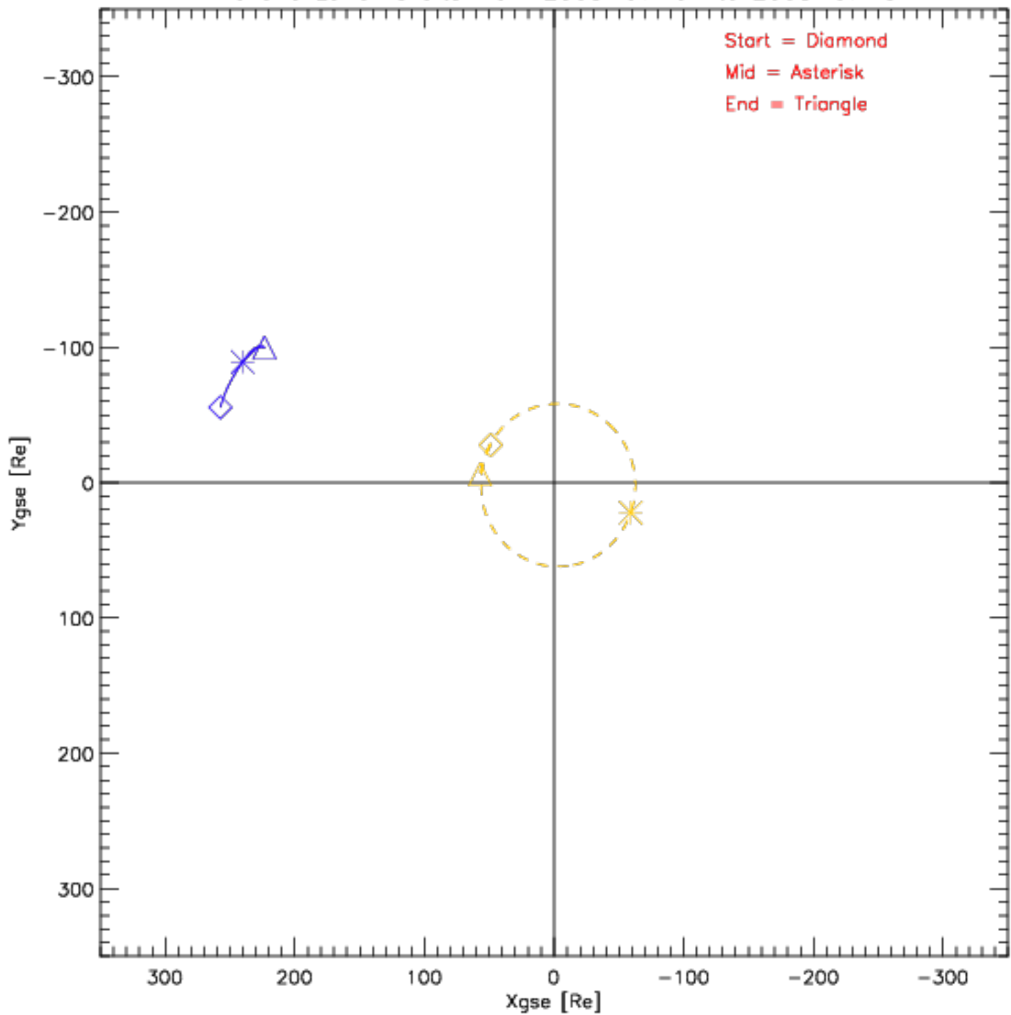
Wind and Lunar Orbits from 2008-07-01 to 2008-07-31
