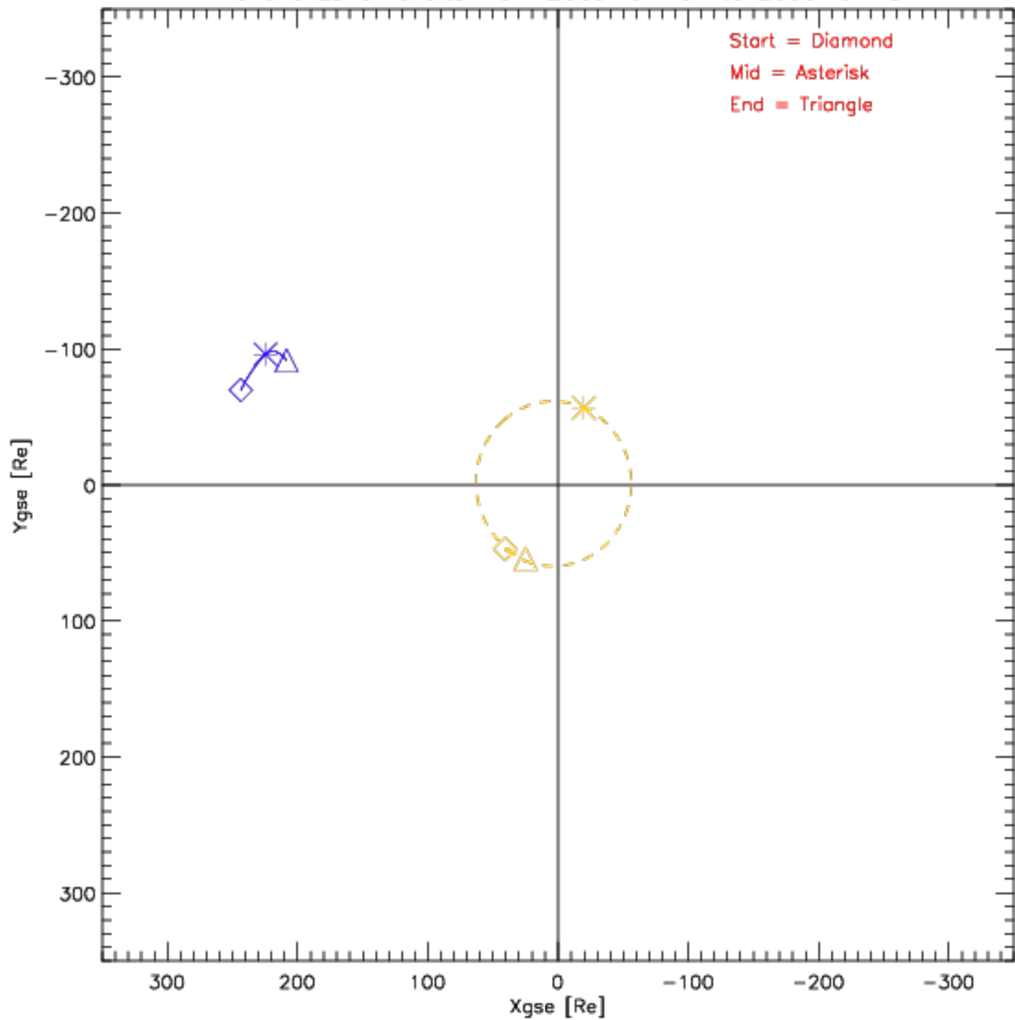
Wind and Lunar Orbits from 2009-01-01 to 2009-01-31
