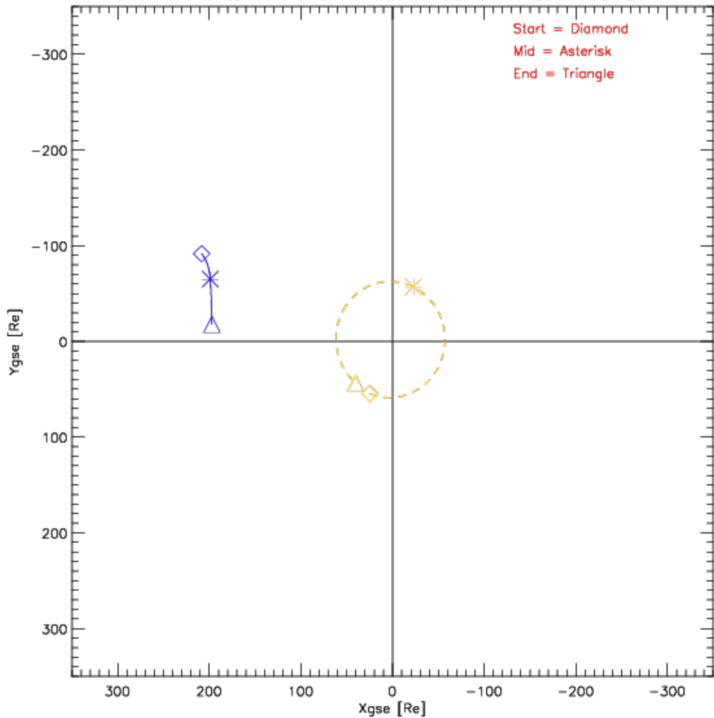
Wind and Lunar Orbits from 2009-02-01 to 2009-02-28
