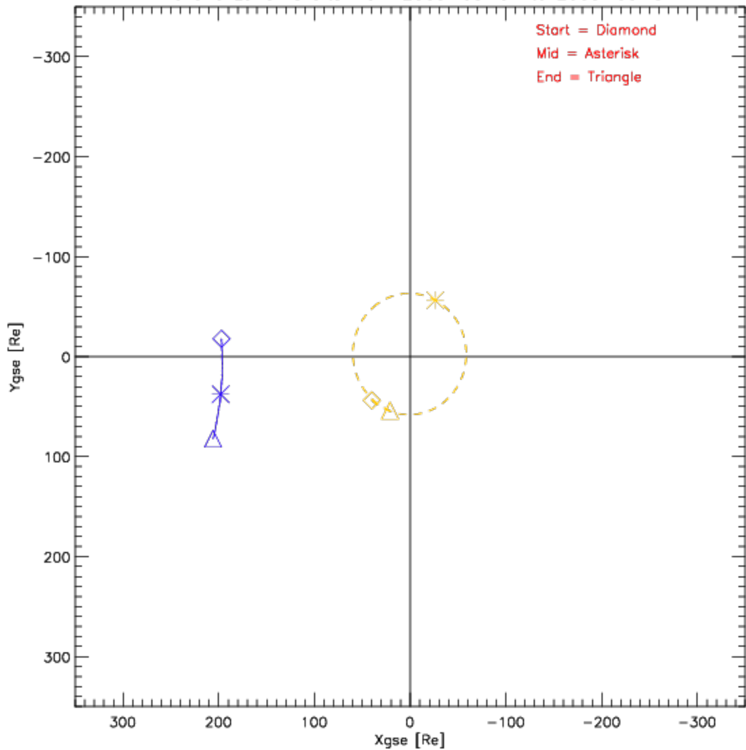
Wind and Lunar Orbits from 2009-03-01 to 2009-03-31
