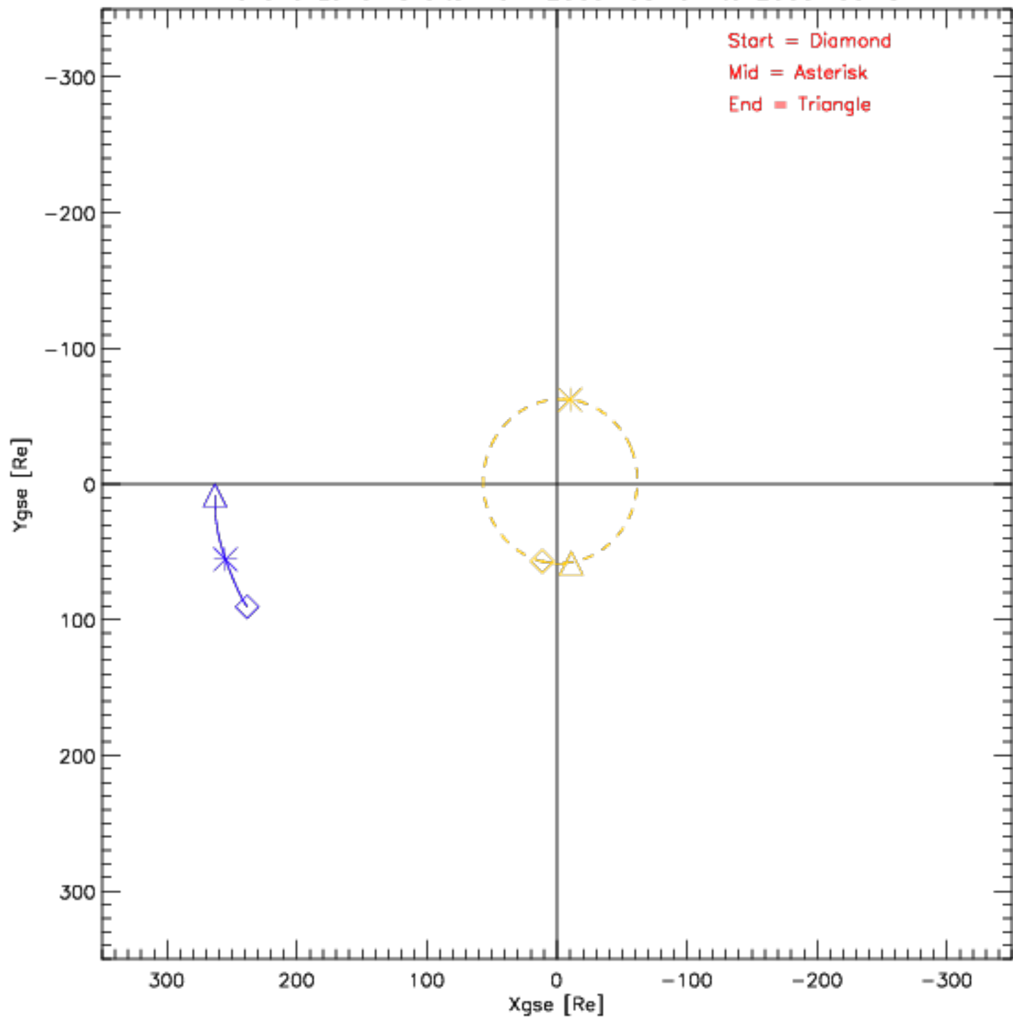
Wind and Lunar Orbits from 2009-05-01 to 2009-05-31
