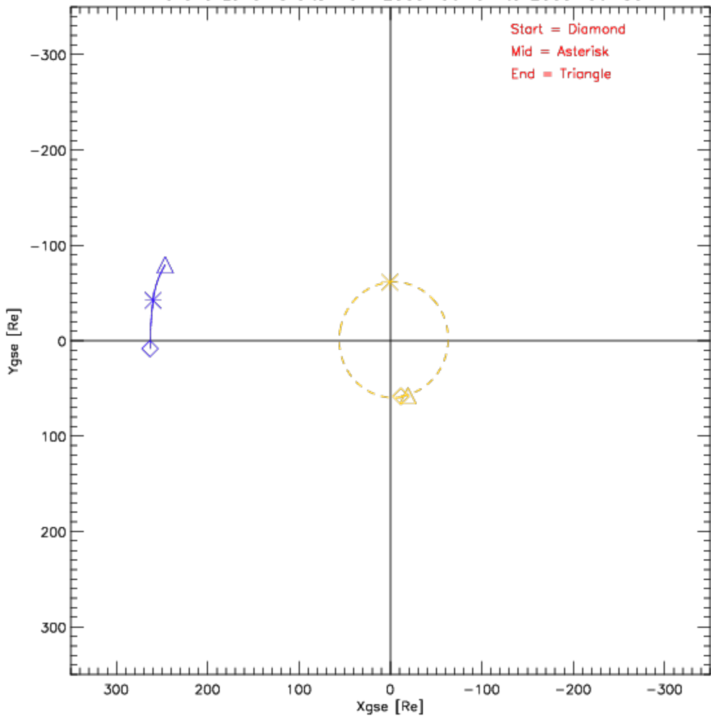
Wind and Lunar Orbits from 2009-06-01 to 2009-06-30
