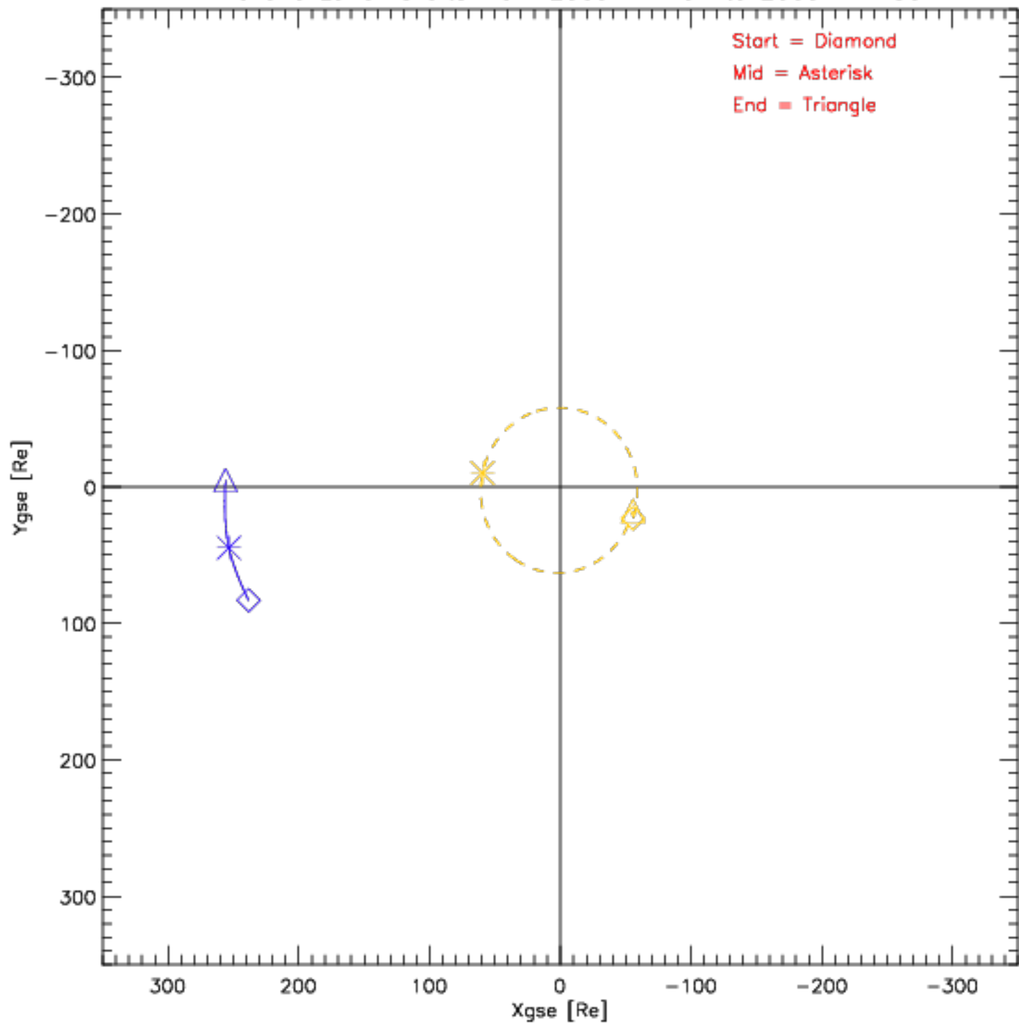
Wind and Lunar Orbits from 2009-11-01 to 2009-11-30
