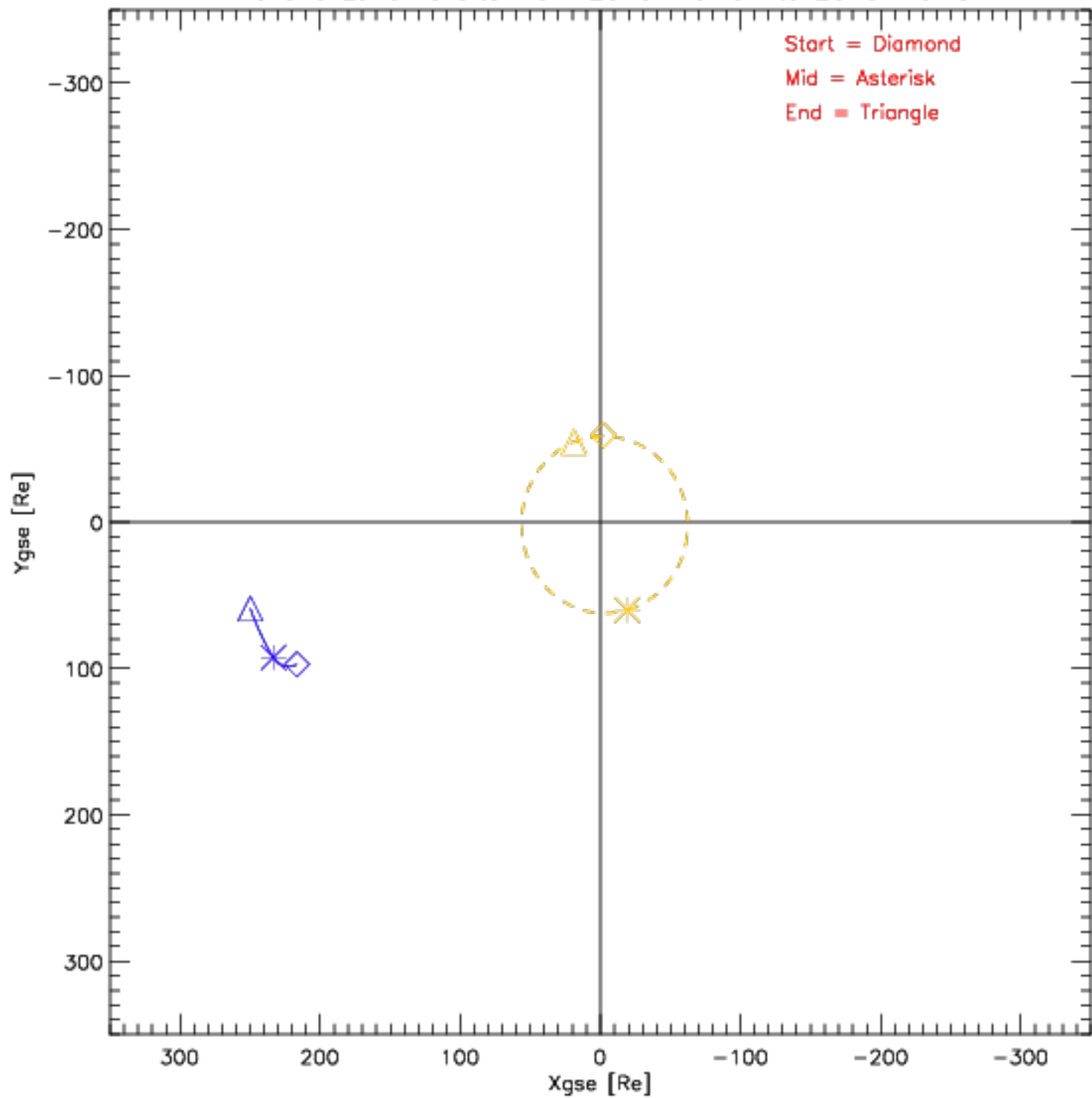
Wind and Lunar Orbits from 2010-10-01 to 2010-10-31
