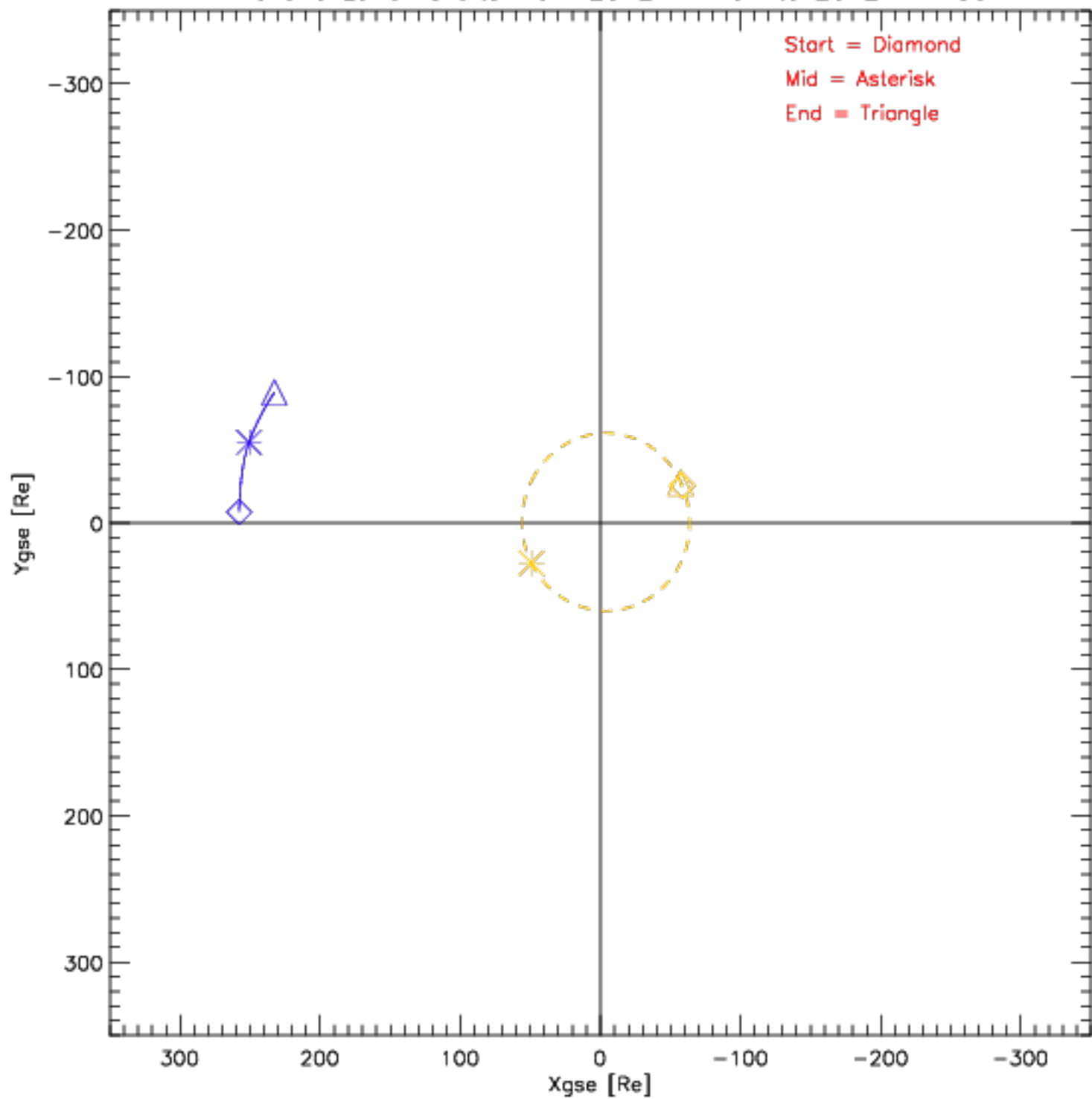
Wind and Lunar Orbits from 2012-11-01 to 2012-11-30
