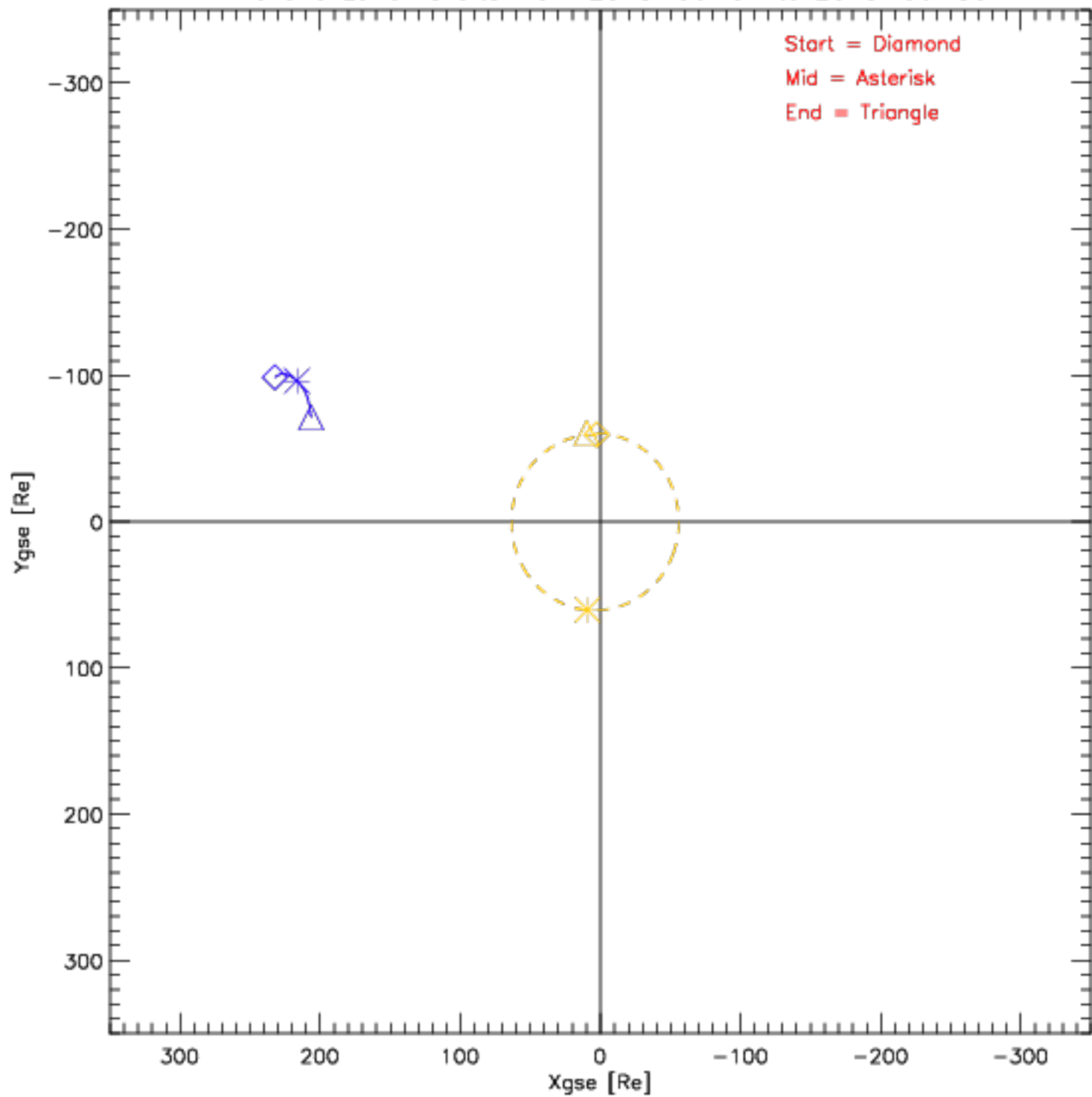
Wind and Lunar Orbits from 2013-06-01 to 2013-06-30
