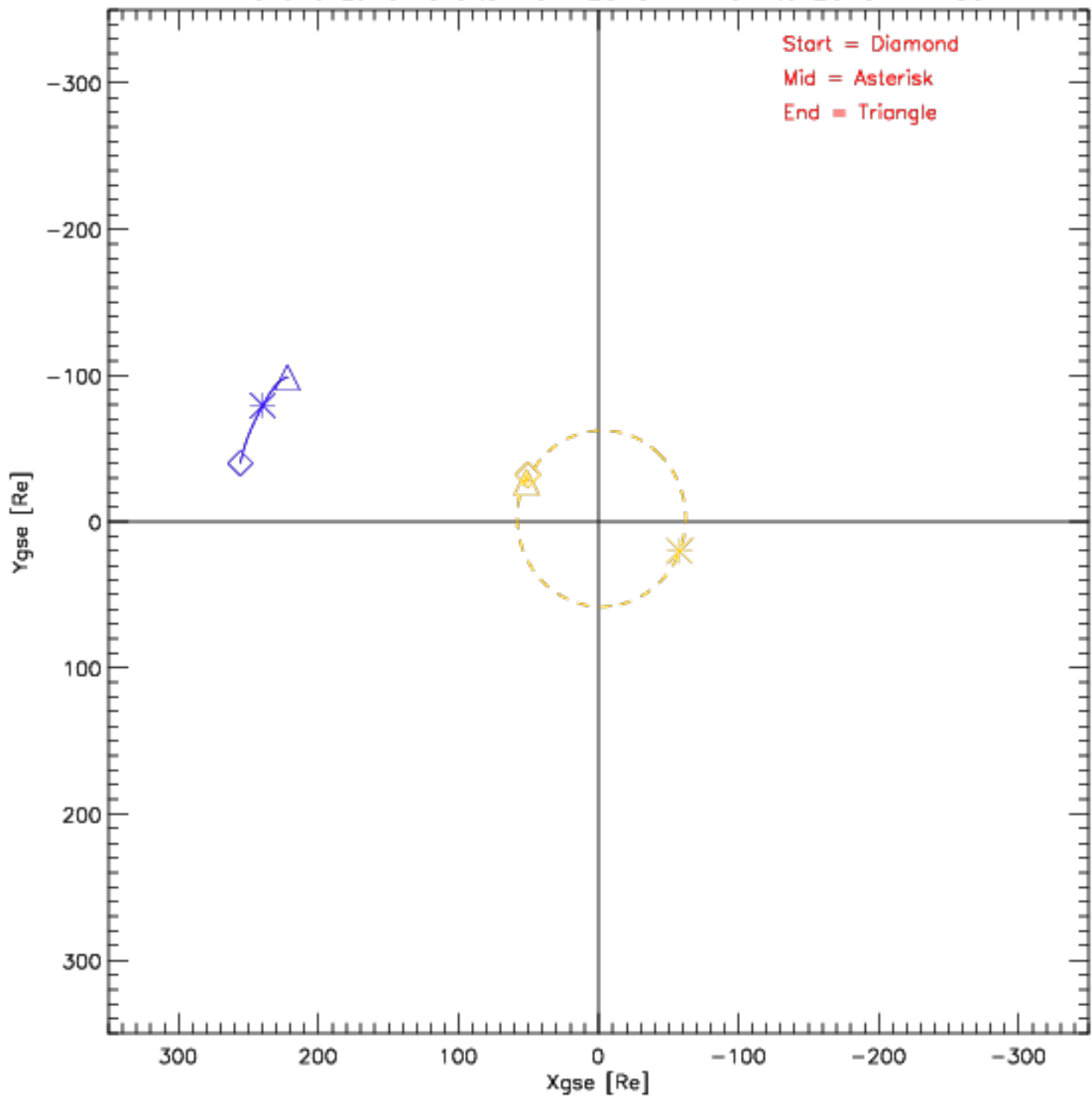
Wind and Lunar Orbits from 2013-11-01 to 2013-11-30
