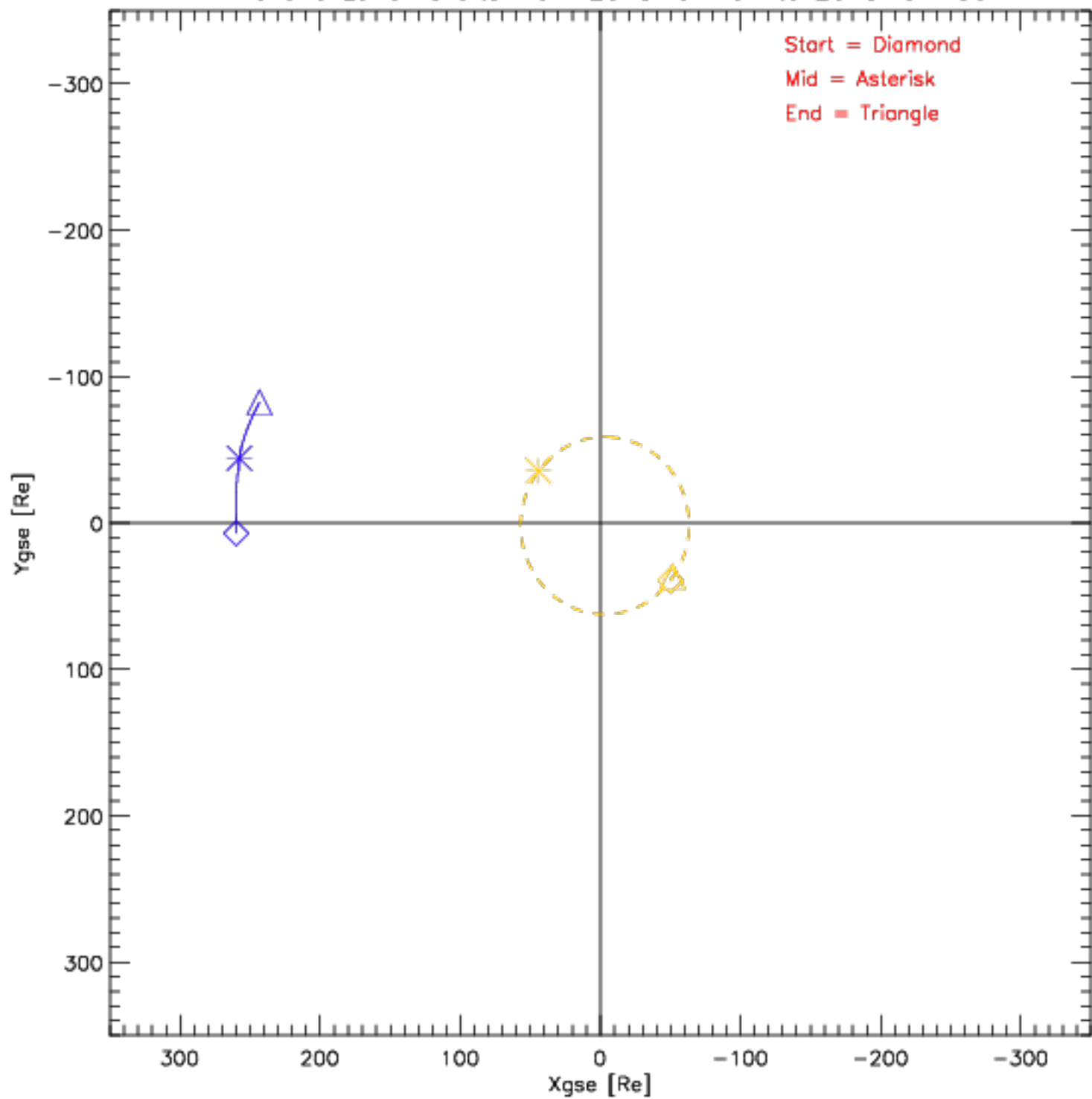
Wind and Lunar Orbits from 2015-04-01 to 2015-04-30
