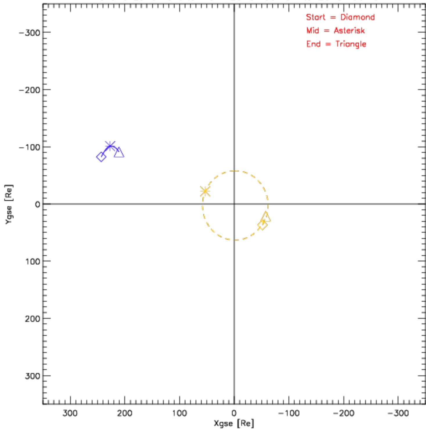
Wind and Lunar Orbits from 2015-05-01 to 2015-05-31
