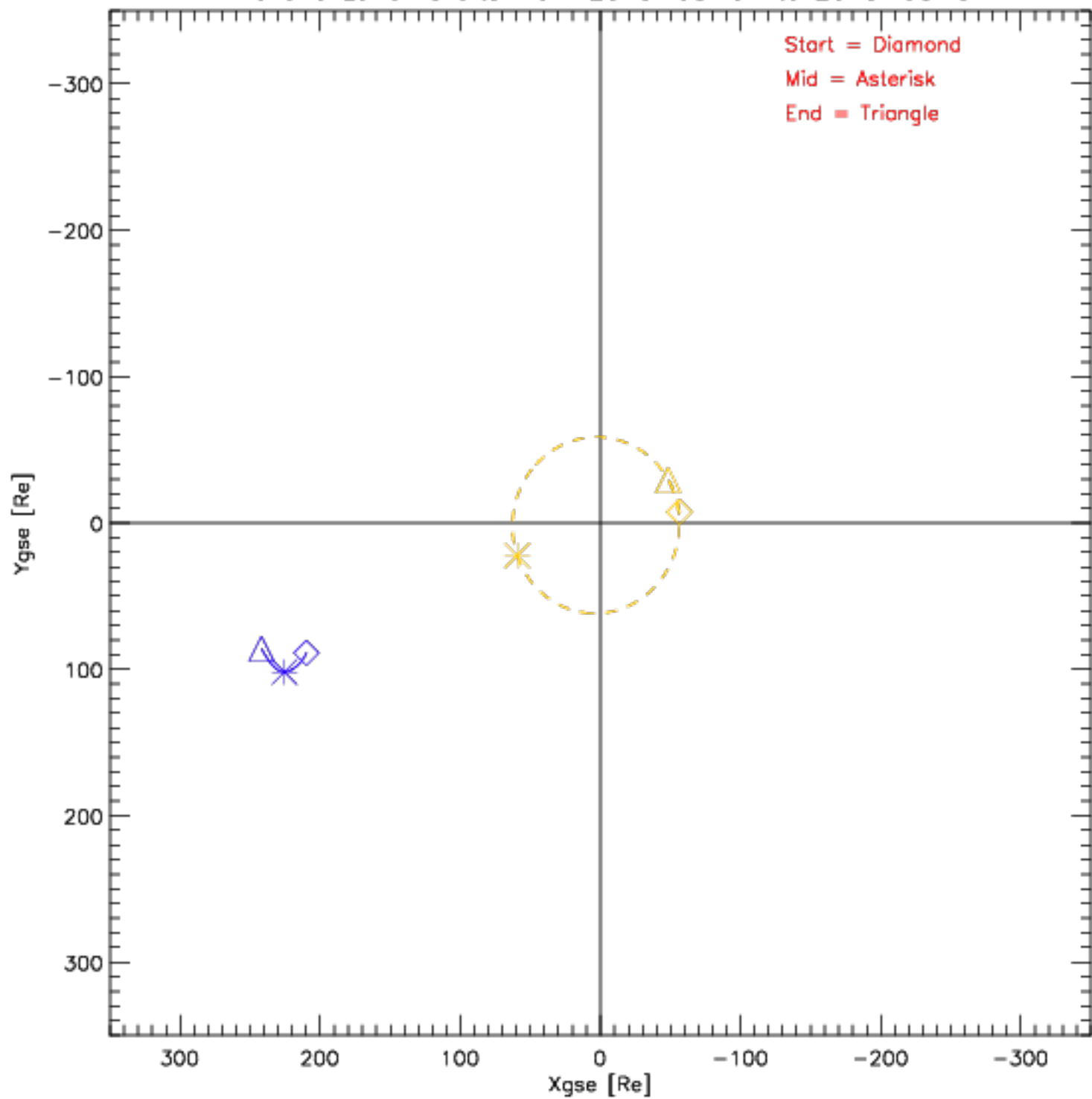
Wind and Lunar Orbits from 2015-08-01 to 2015-08-31
