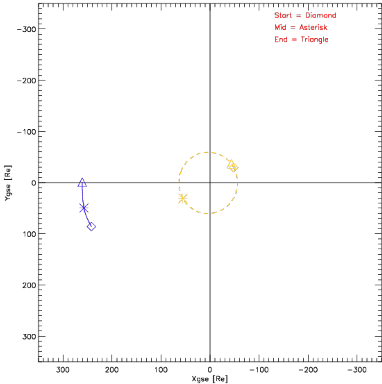
Wind and Lunar Orbits from 2015-09-01 to 2015-09-30
