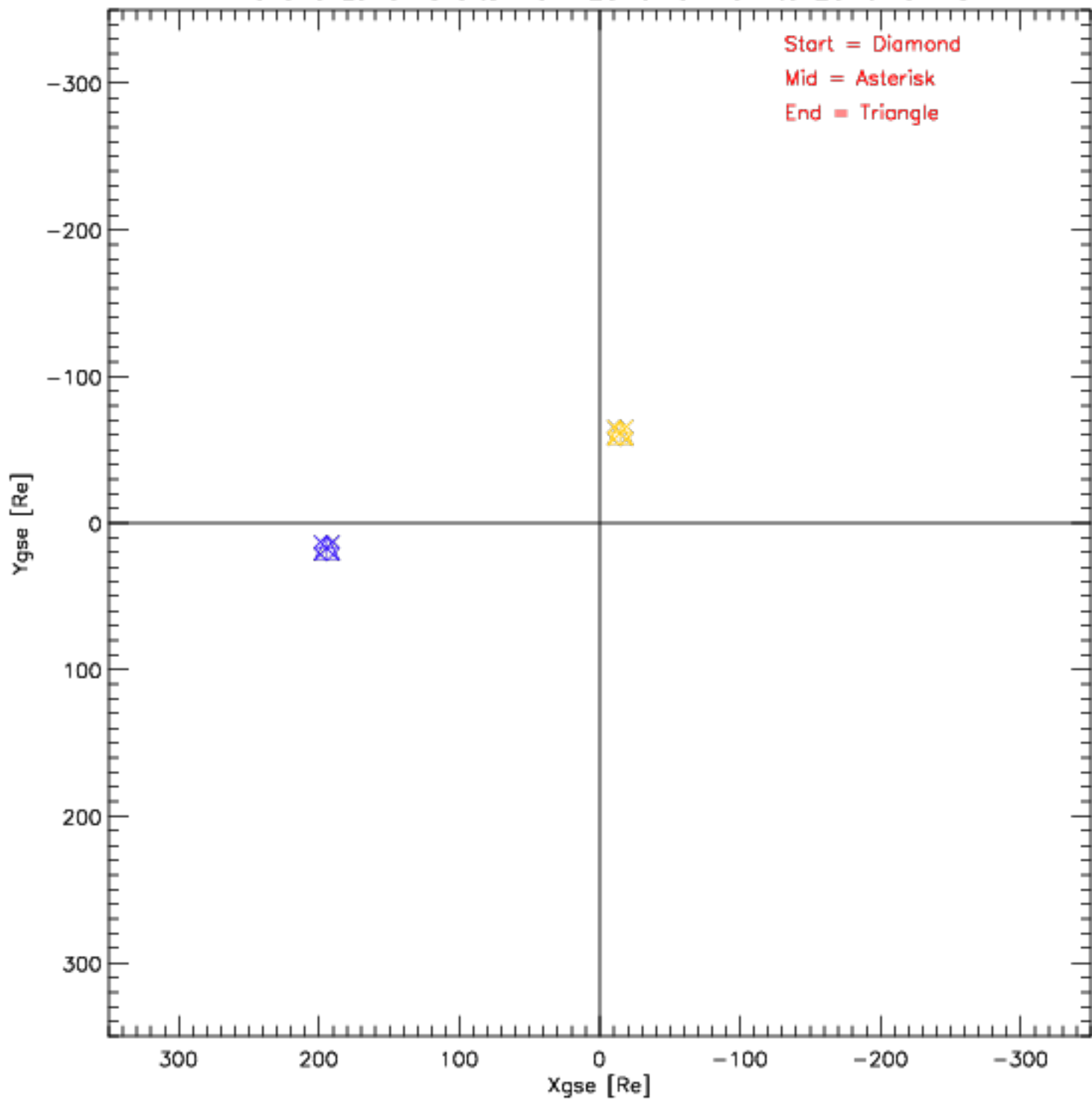
Wind and Lunar Orbits from 2016-01-01 to 2016-01-31
