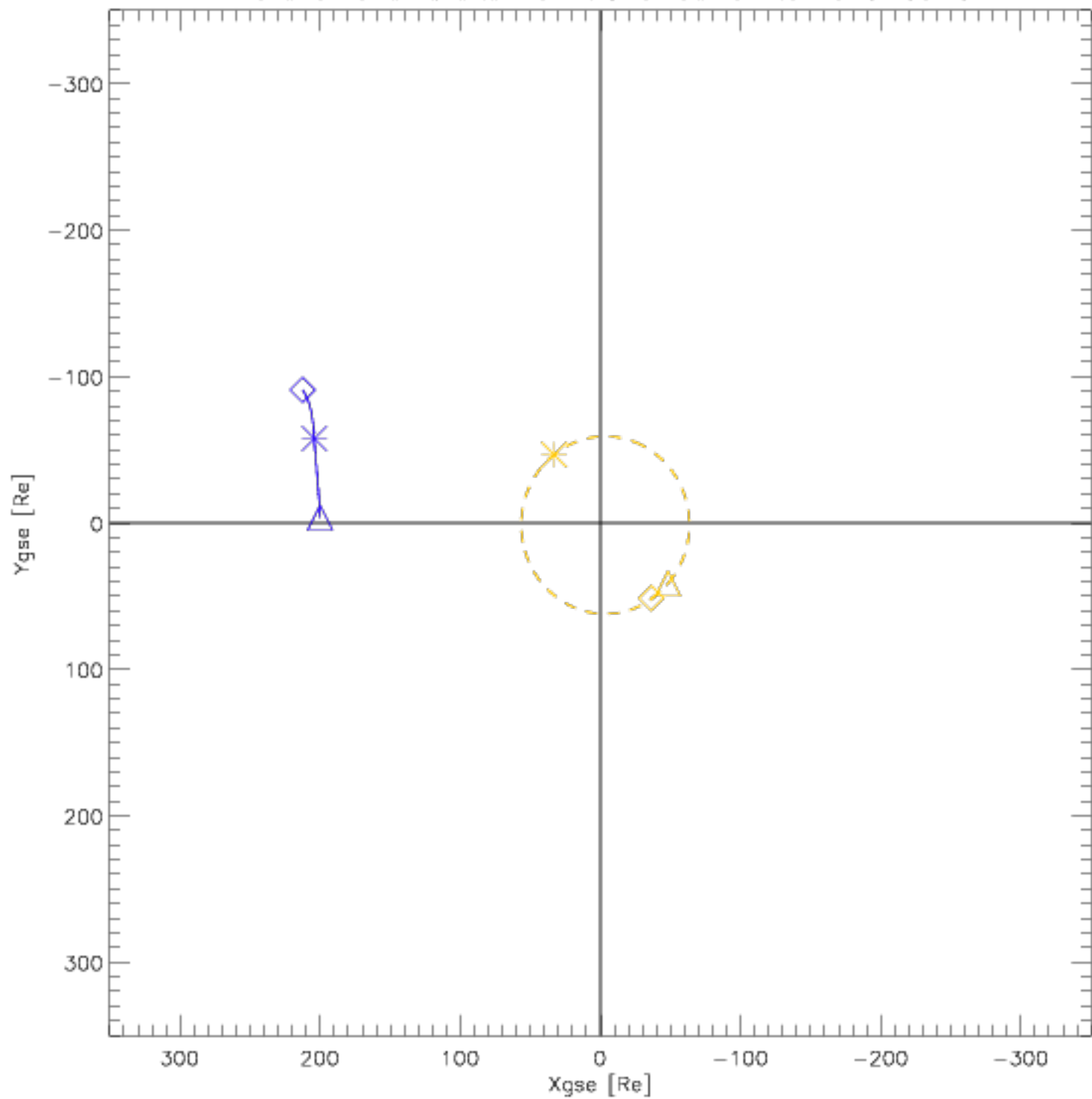
Wind and Lunar Orbits from 2016-08-01 to 2016-08-31
