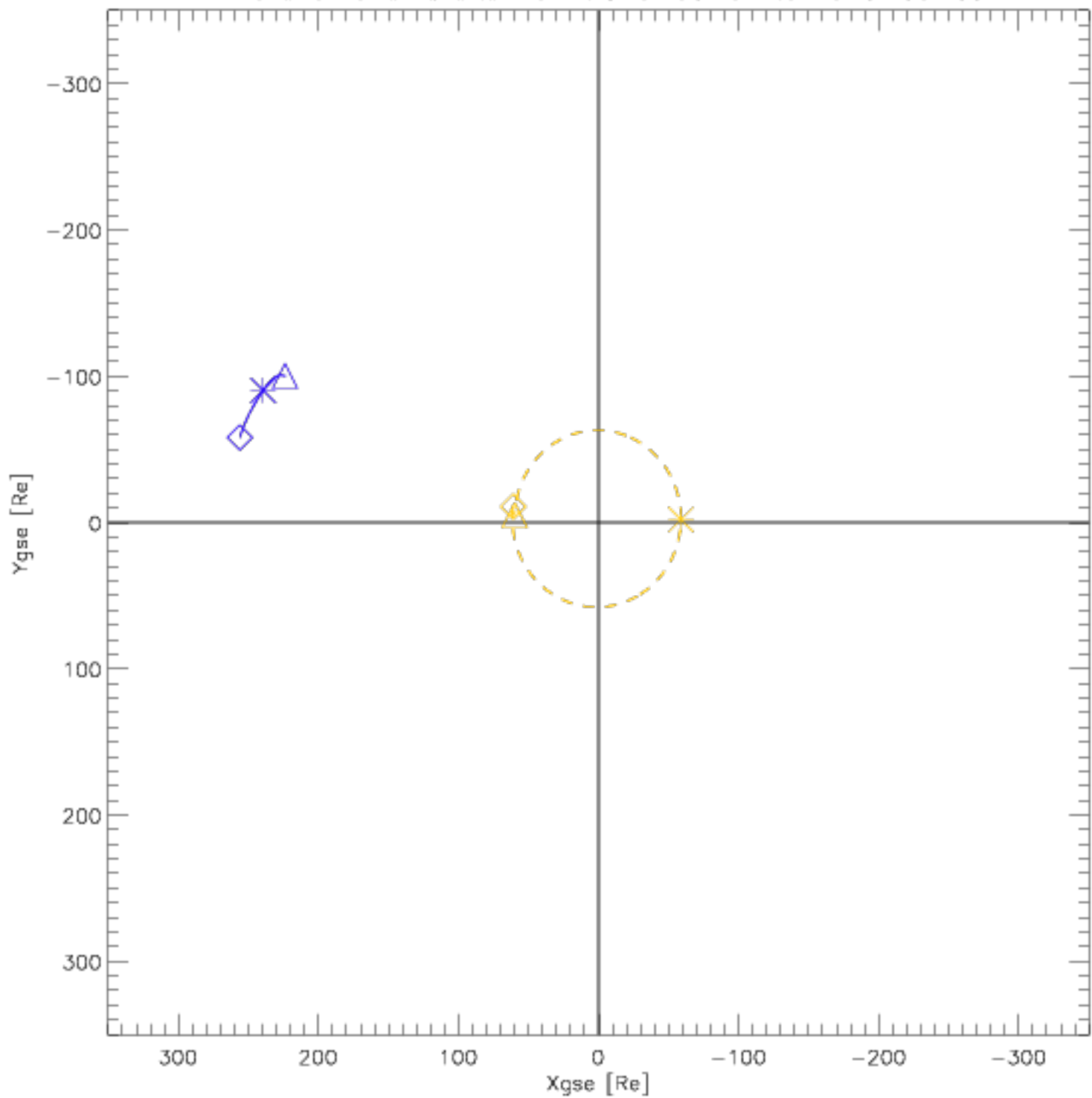
Wind and Lunar Orbits from 2016-09-01 to 2016-09-30
