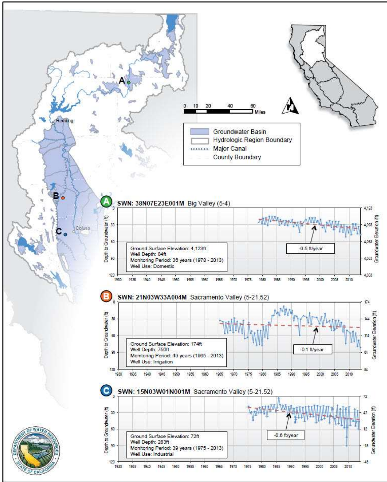
Figure 16 - Selected Hydrographs – Sacramento River Hydrologic Region
