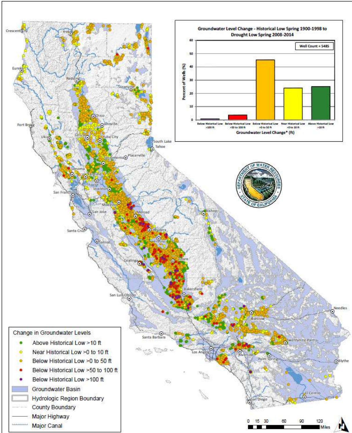
Figure 13 - Groundwater Level Change* – Historical Low Spring 1900-1998 to Drought Low Spring 2008-2014
