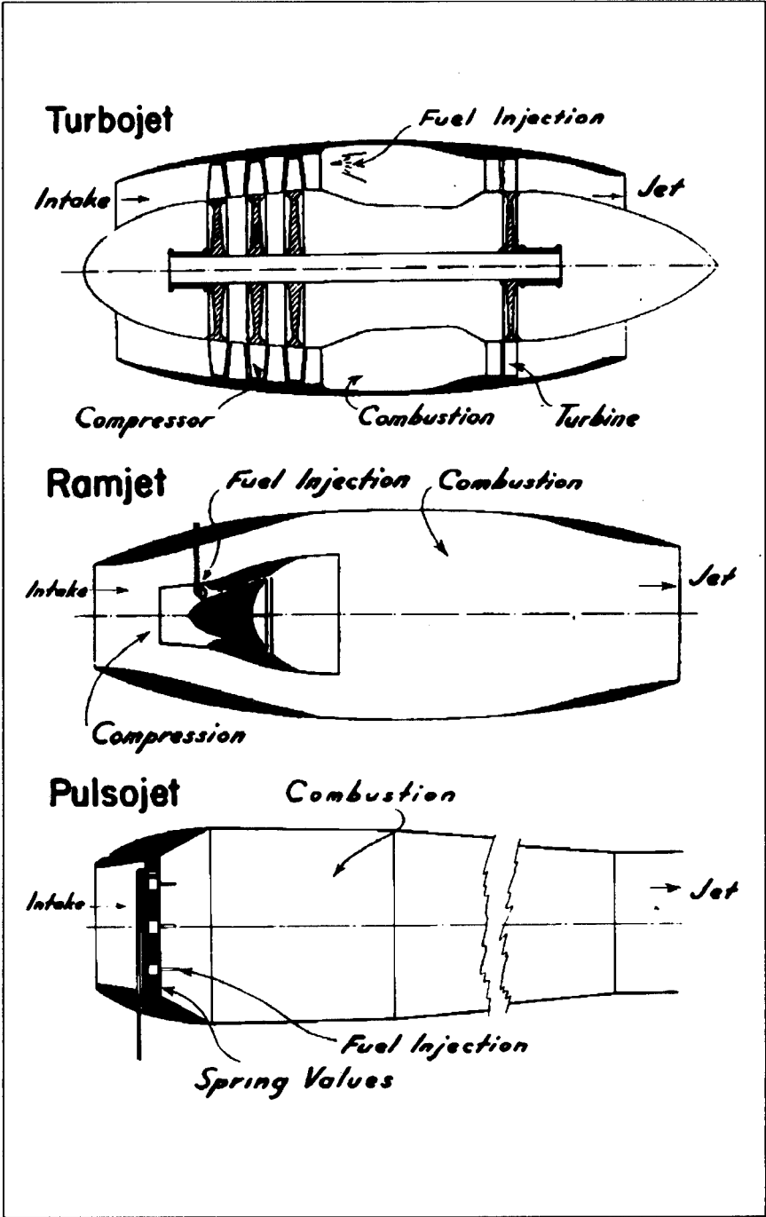
Figure 10-B—Various Propulsion Systems
