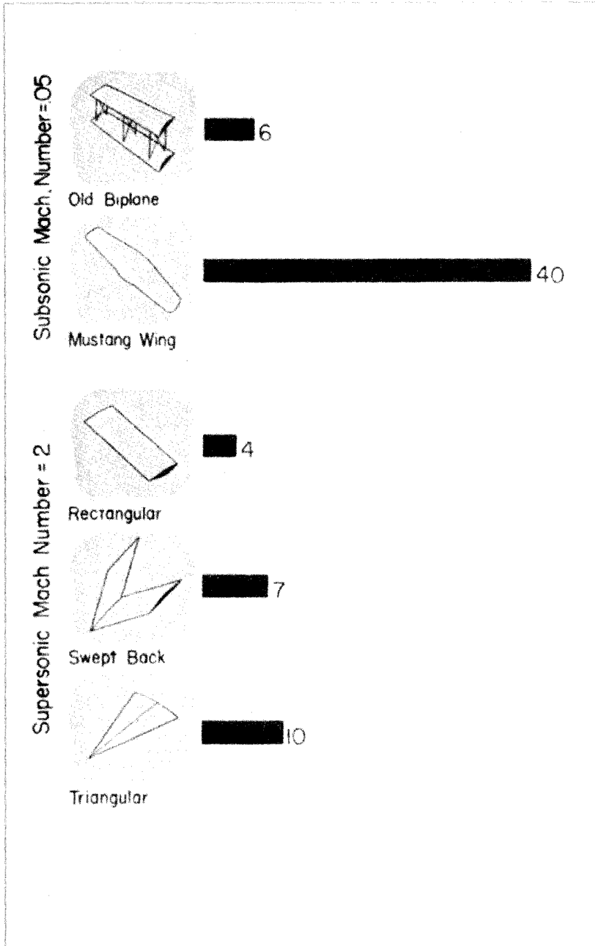
Figure 3—Optimum Lift-Drag Ratios
