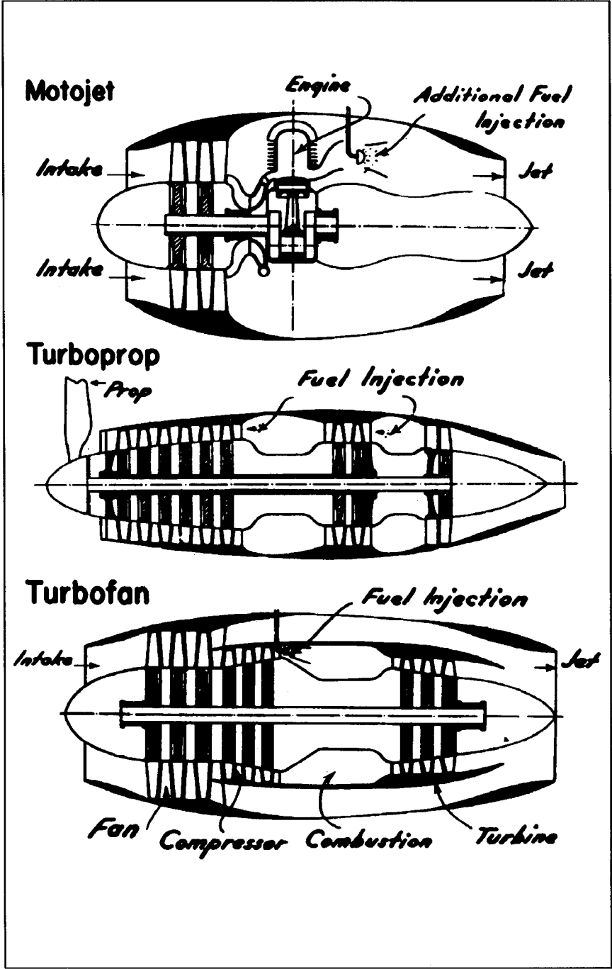
Figure 10-A-Variety Propulsion Systems
