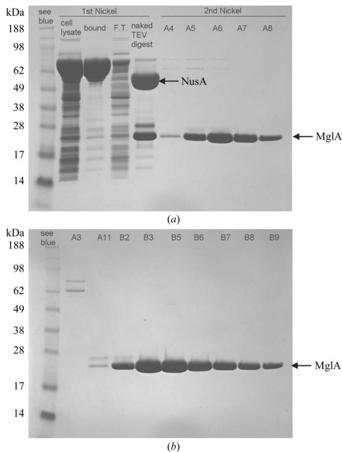
Figure 1 Protein purification. (a) First pass over Ni-NTA column followed by overnight TEV cleavage and subsequent second Ni-NTA-bound fractions. (b) Gel-filtration chromatography.
